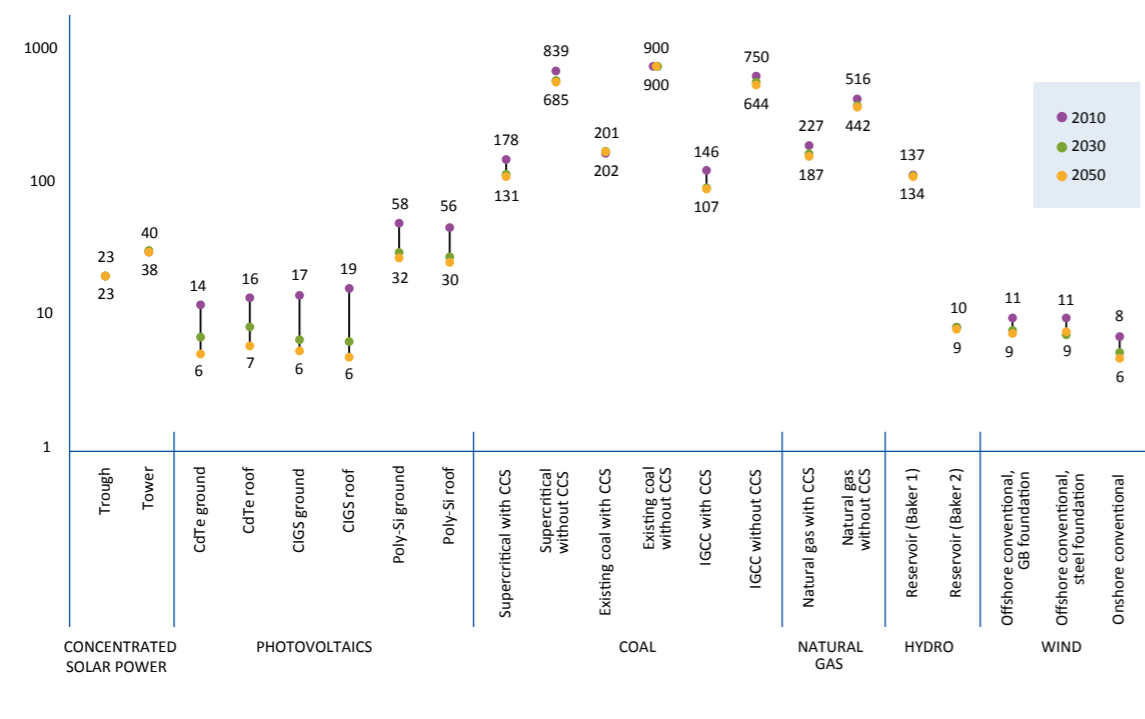
Figure 86: Life-cycle GHG emissions of different electricity generation technologies, in gCO 2 e/kWh
