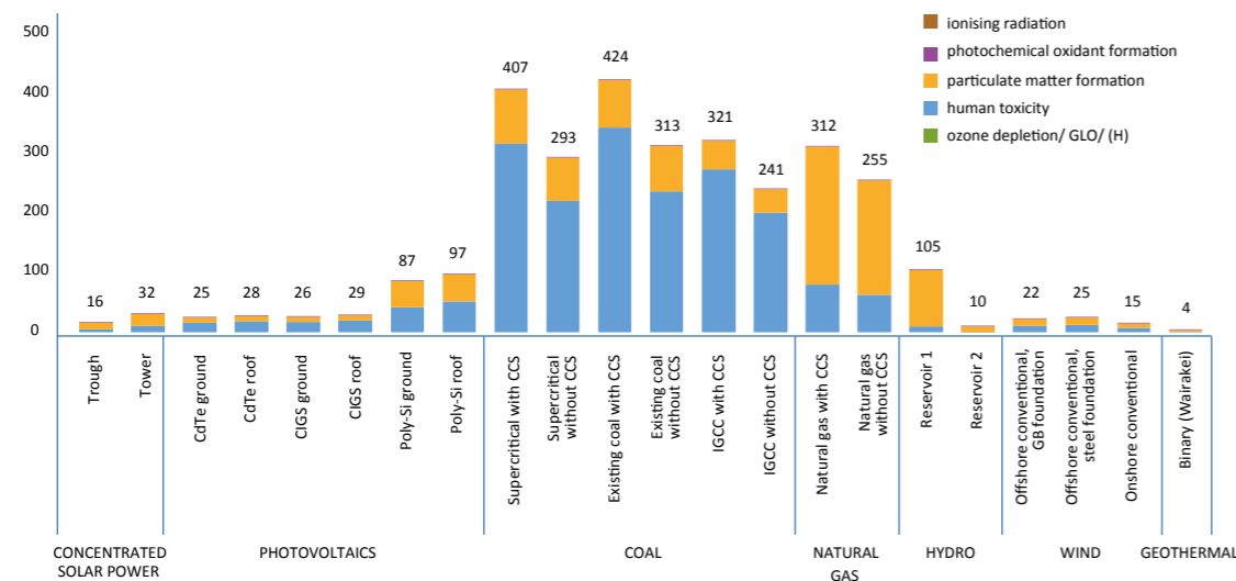
Figure 87: Human health impact in disability adjusted life years (DALY) per unit of electricity generated (kWh) of selected electricity generation technologies
