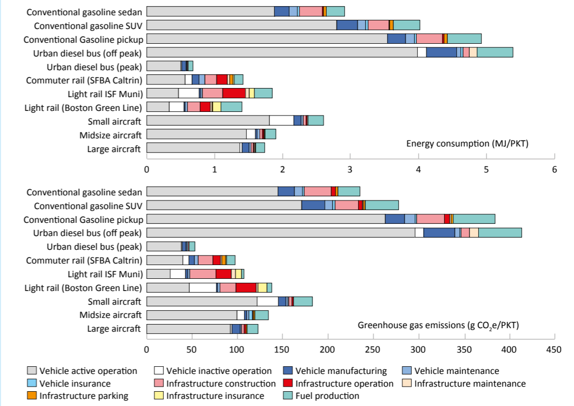
Figure 83: Energy consumption and GHG emissions per passenger-km travelled
