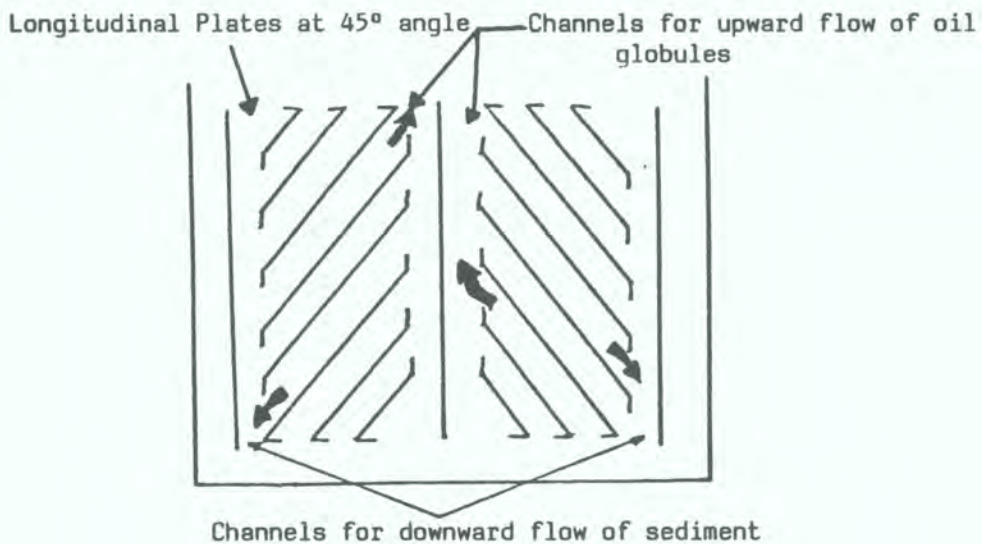
Figure III: Cross-section of a parallel plate interceptor
