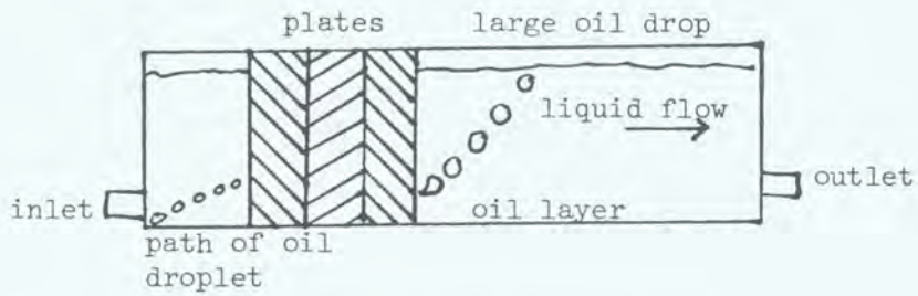
Figure VII: The essentials of a coalescer
