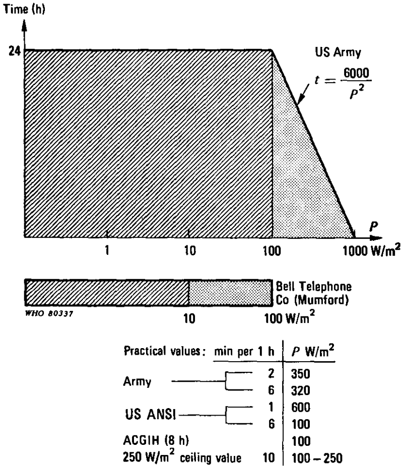
Fig. 19. Comparison of some of the exposure limits proposed in the USA (see also Table 18).
