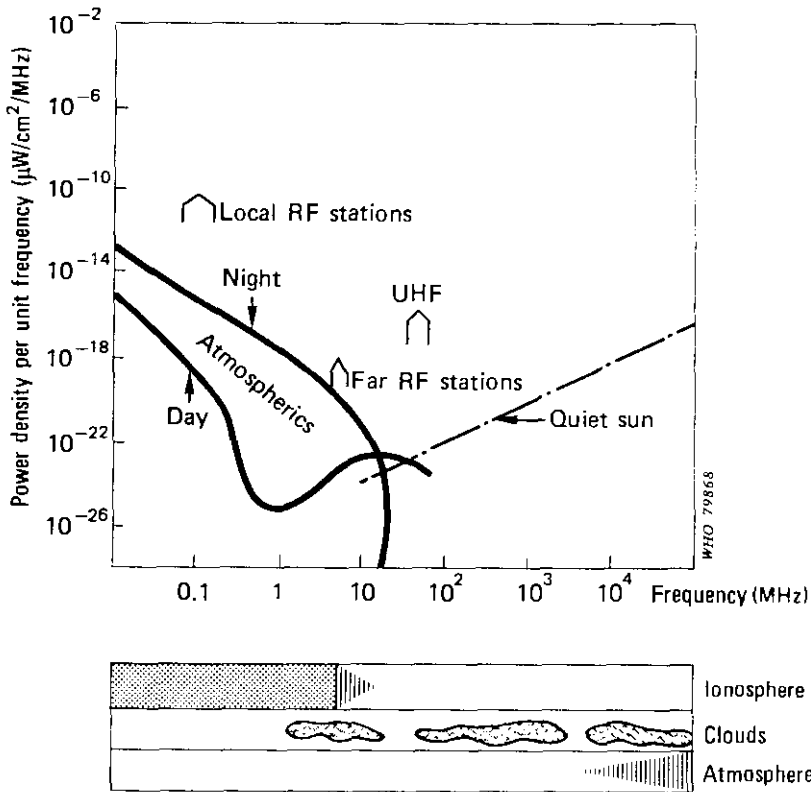
Fig. 3. Comparison of natural background and man-made RF and microwave radiation (From: Minin, 1974).
