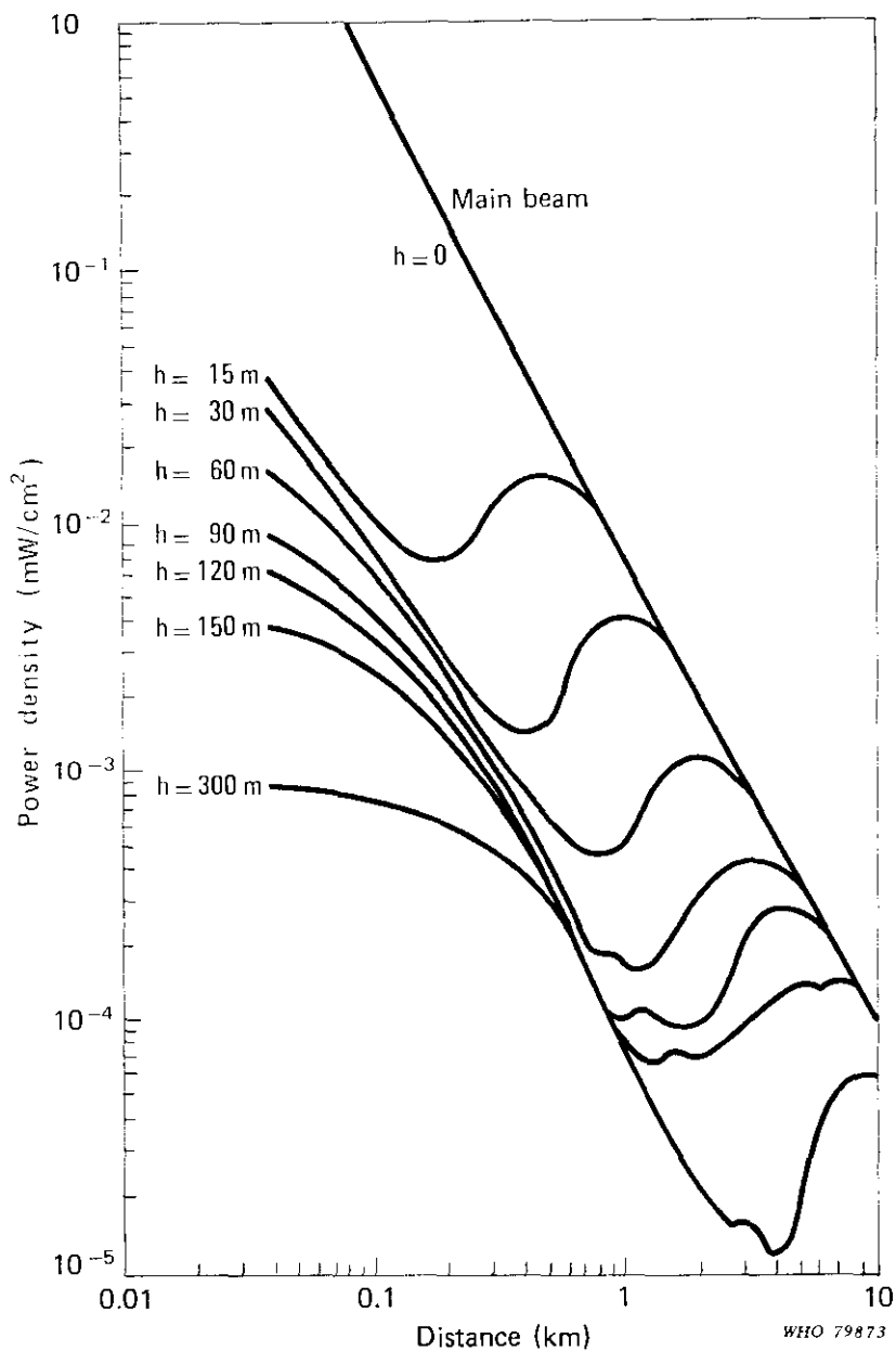
Fig. 8. Power density versus distance at various heights for a TV station with ERP equal to 1 mW/cm 2 (From: National Health and Welfare, Canada, 1977).
