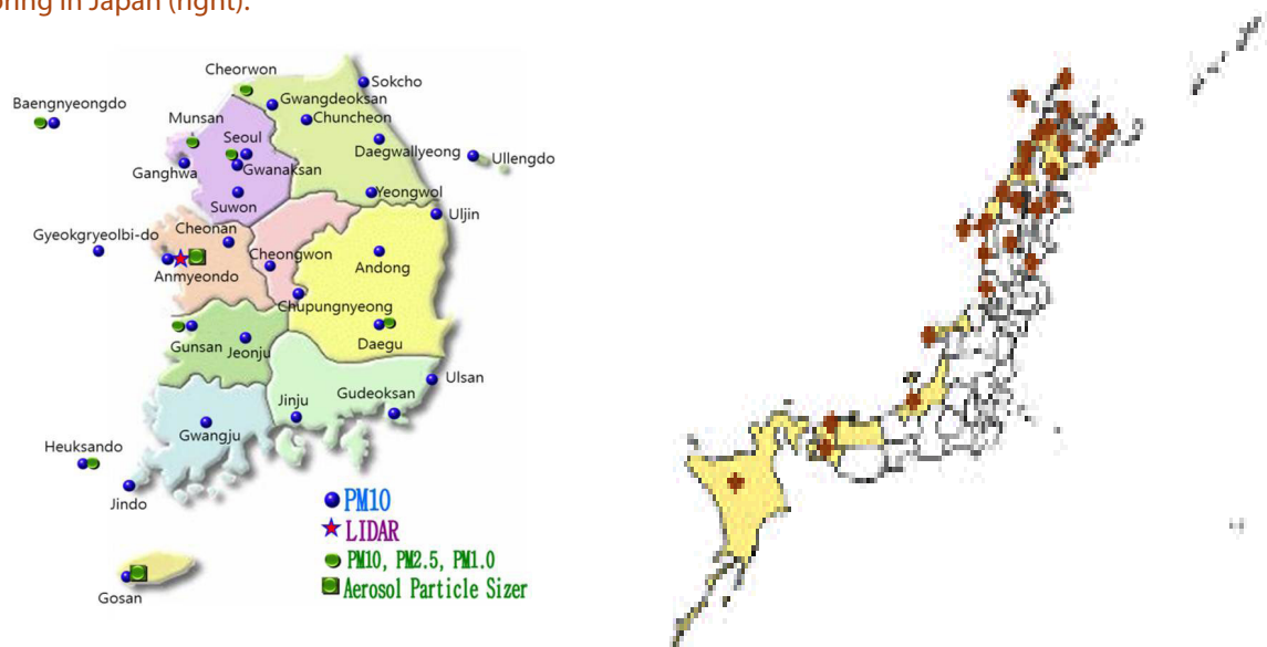
Figure 5.7: Sand and dust storm observation stations of the Korean Meteorological Association (left) and PM10 monitoring in Japan (right).
