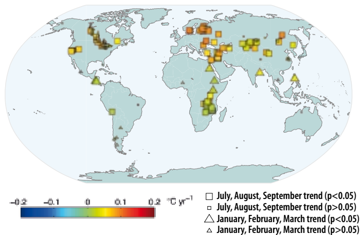
Figure 6: Worldwide trends in nighttime lake surface temperature derived from satellite data. Source: Schneider and Hook (2010)
