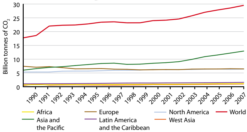
Figure 2: Carbon dioxide emissions from solid fuel consumption, expressed in billions of tonnes of CO 2 , 1989-2007. Although emissions from fossil fuel consumption are stabilizing in Europe and North America, they are increasing in Asia and the Pacific. Data sources: GEO Data Portal, compiled from the Carbon Dioxide Information Analysis Center (CDIAC), Boden et al. (2010)
