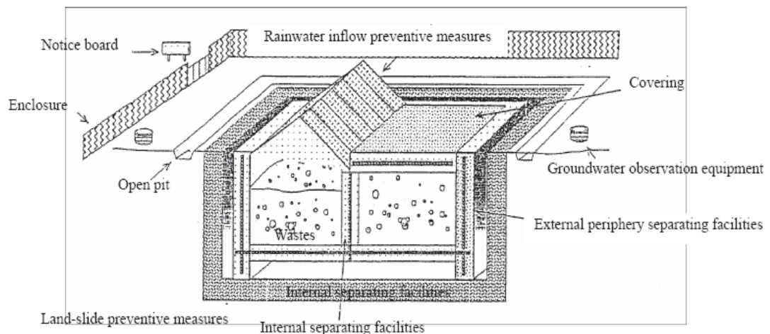
Figure -6 Specially engineered landfill (Ministry of the Environment, Japan 2007a)
