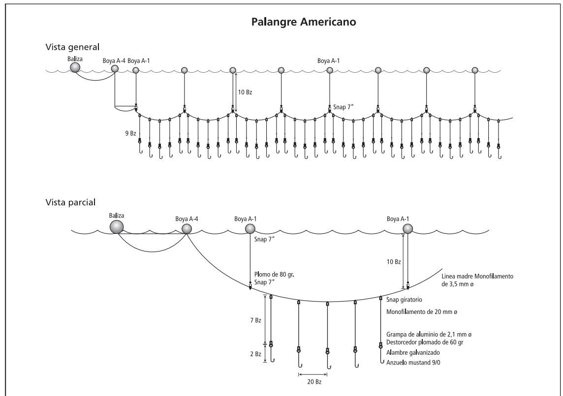
Fig. A2.5. Diagram of longline gear using the American System.
