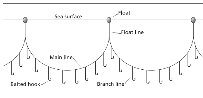
Fig. 1.1. Generalized configuration of pelagic longline gear.
