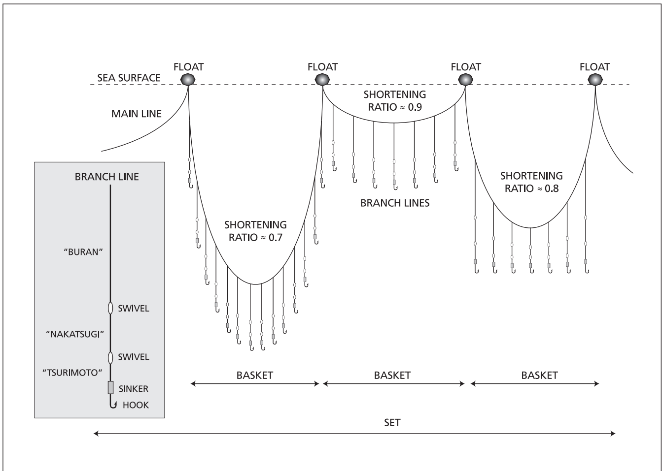
Fig. A5.4. Components of Japanese longline gear and various configurations used historically and currently (see text).
