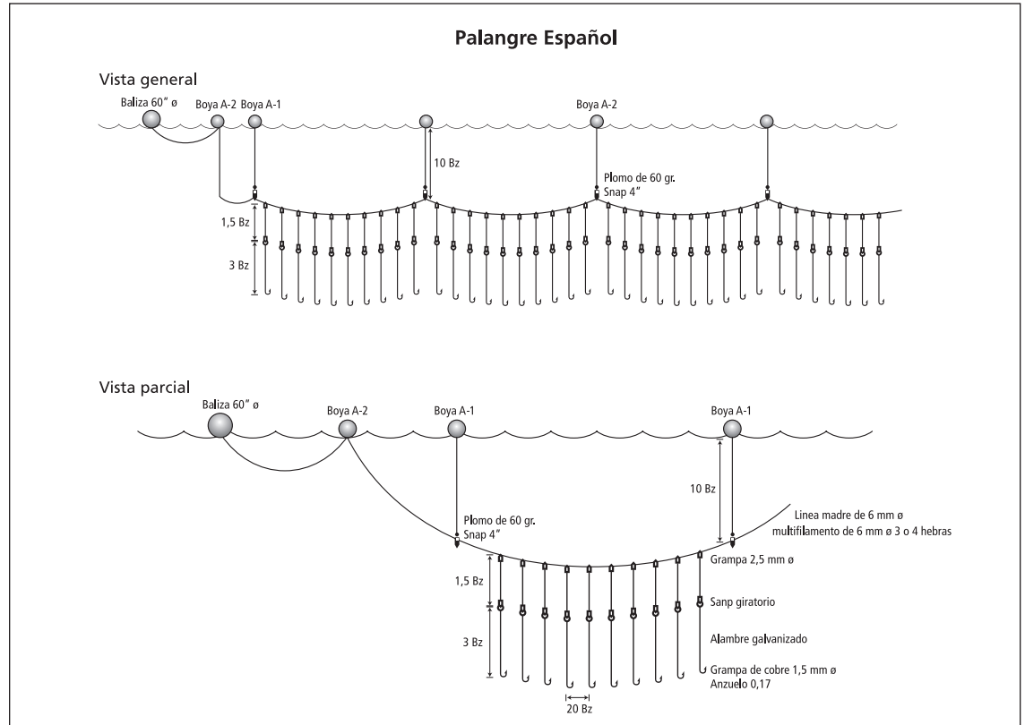
Fig. A2.4. Diagram of longline gear using the Spanish System.
