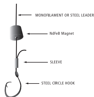
Fig. A9.7. Illustration of a magnet prototype that received first prize in the 2006 World Wildlife Fund Smartgear Competition ( http://www.worldwildlife.org/oceans/projects/smartgear.cfm ).
