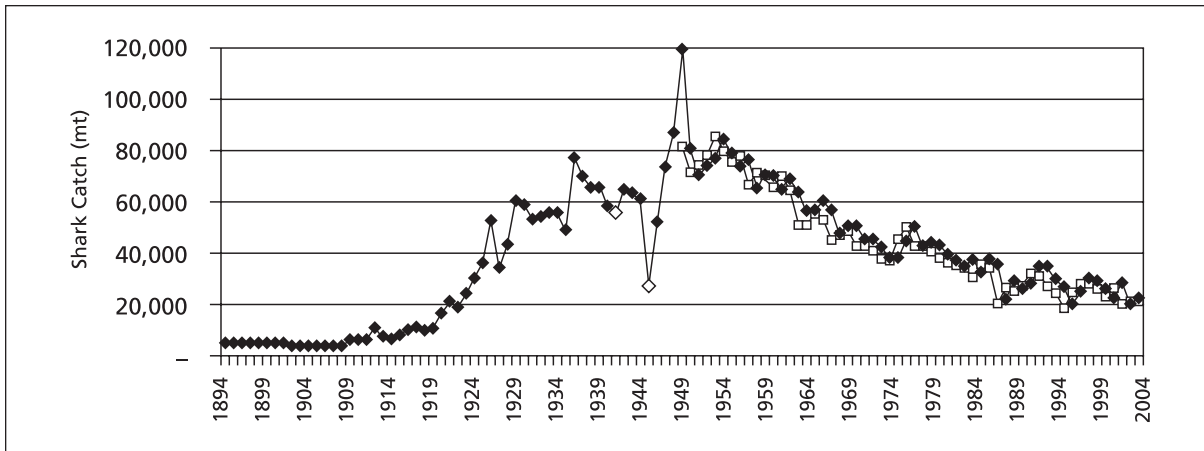
Fig. A5.2. Shark catch (in mt) by Japan, 1894-2004. Data from 1894-1949 (◆), when Japan's fishing activities were limited to the Pacific, were sourced from Okamoto (2004). Data from 1950-2004 (♦) are Japan's catches for all oceans and subset, to the maximum extent practical, to exclude non-shark elasmobranches (FAO 2006). Japan's reported catches for the Pacific (only) are denoted with □ (FAO 2006). The beginning (1941) and ending (1945) of WWII are shown with open circles (○).
