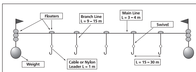
Fig. A6.2. Typical gear design of a Peruvian pelagic longline.
