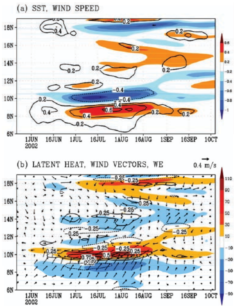
Figure 17: Time–latitude plots of (top) SST (°C, shaded) and wind speed (m/s, contoured with CI=0.2 m/s), and (bottom) latent heat flux (shaded, W/m 2 ), 10-m wind vectors (m/s) and Ekman pumping velocities (m/day, contoured with CI = 0.25). The fields shown are spatially highpass filtered (10°) parallel to the coast (southwest to northeast) and then averaged within 2° longitude from the coast (Seo et al. 2008).
