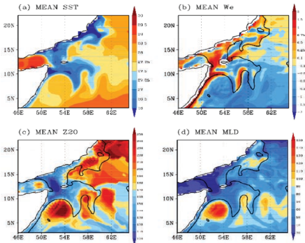
Figure 18: Mean (a) SST ( ^{\circ}\text{C} ), (b) Ekman pumping velocities ( W_e , m/day), (c) thermocline depth ( Z_{20} , m) and (d) mixed layer depth (MLD, m) for August 2002. The contour in (b–d) denotes isotherms of 27.25^{\circ}\text{C} , which represents the cold filaments (Seo et al. 2008).
