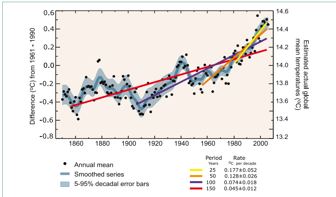
Figure 8.4 Recorded changes in global average temperature since 1850
