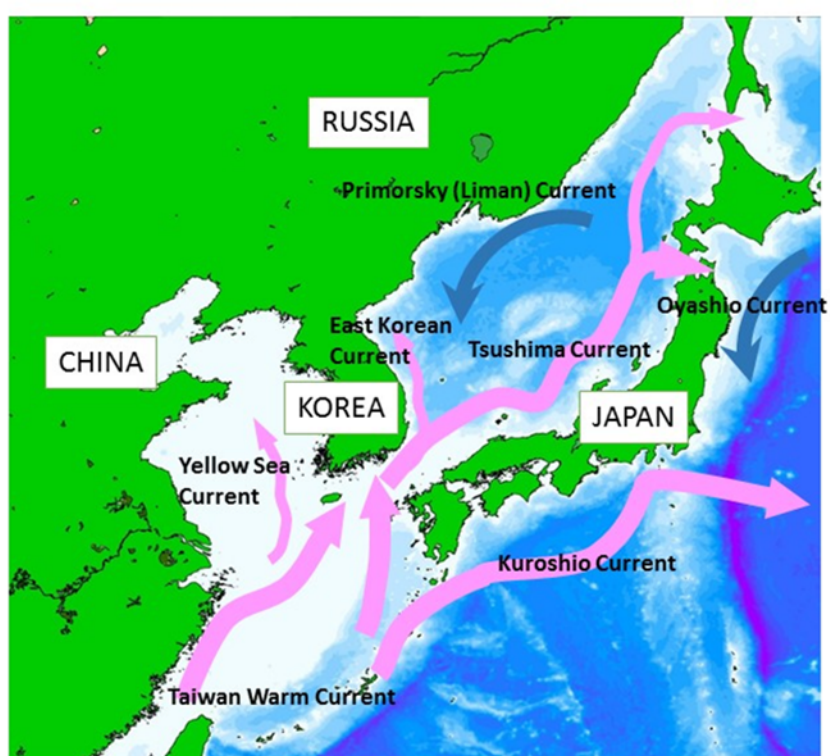
Figure 1 Ocean current in the NOWPAP region
