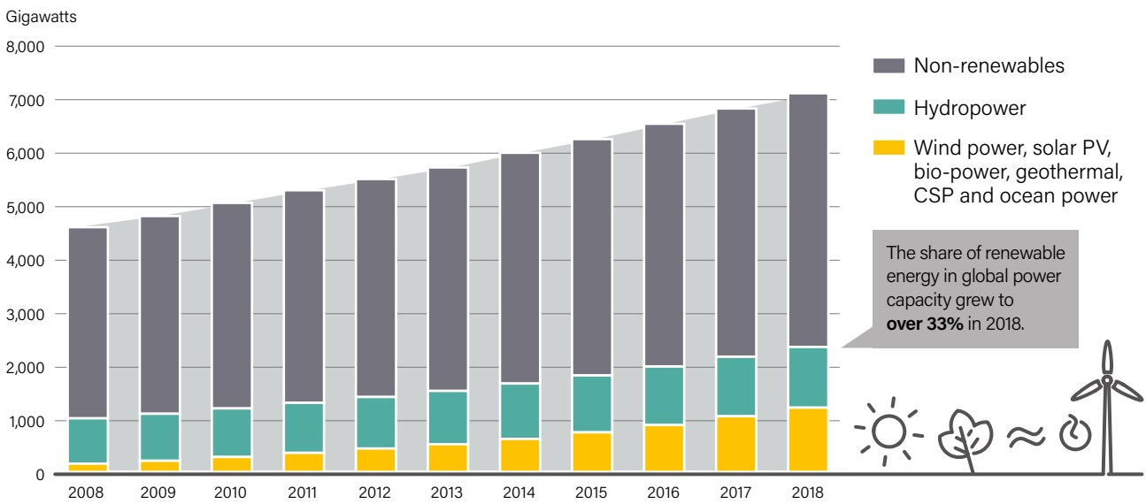
FIGURE 7. Global Power Generating Capacity, by Source, 2008-2018
