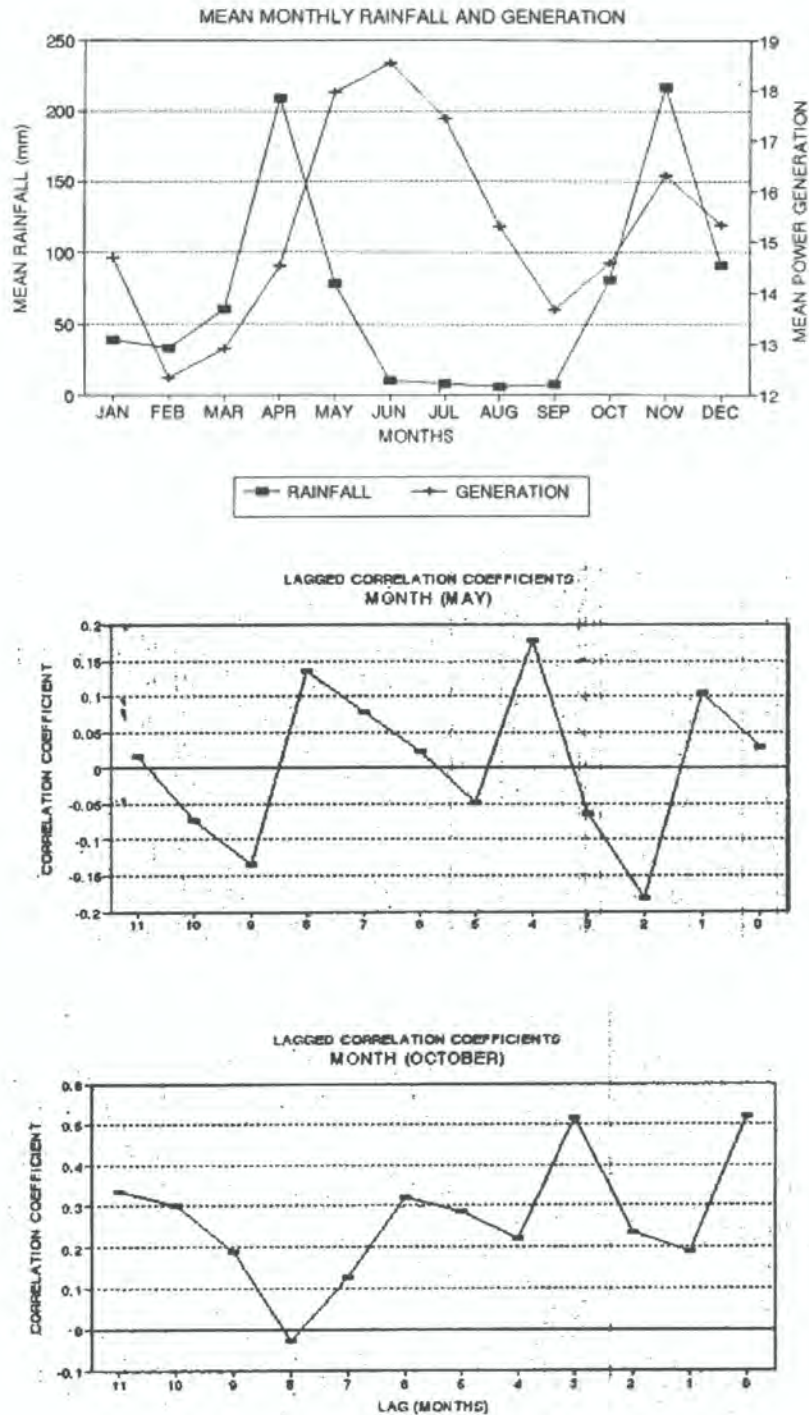
Fig. 5.19 Relationship between mean monthly rainfall and power generation for the Tana River Basin for the period 1969-1995
