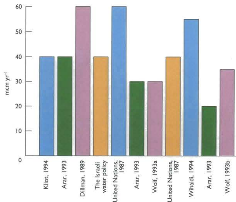
Figure 4.16 Estimates of the current annual water deficit in the Gaza Strip
