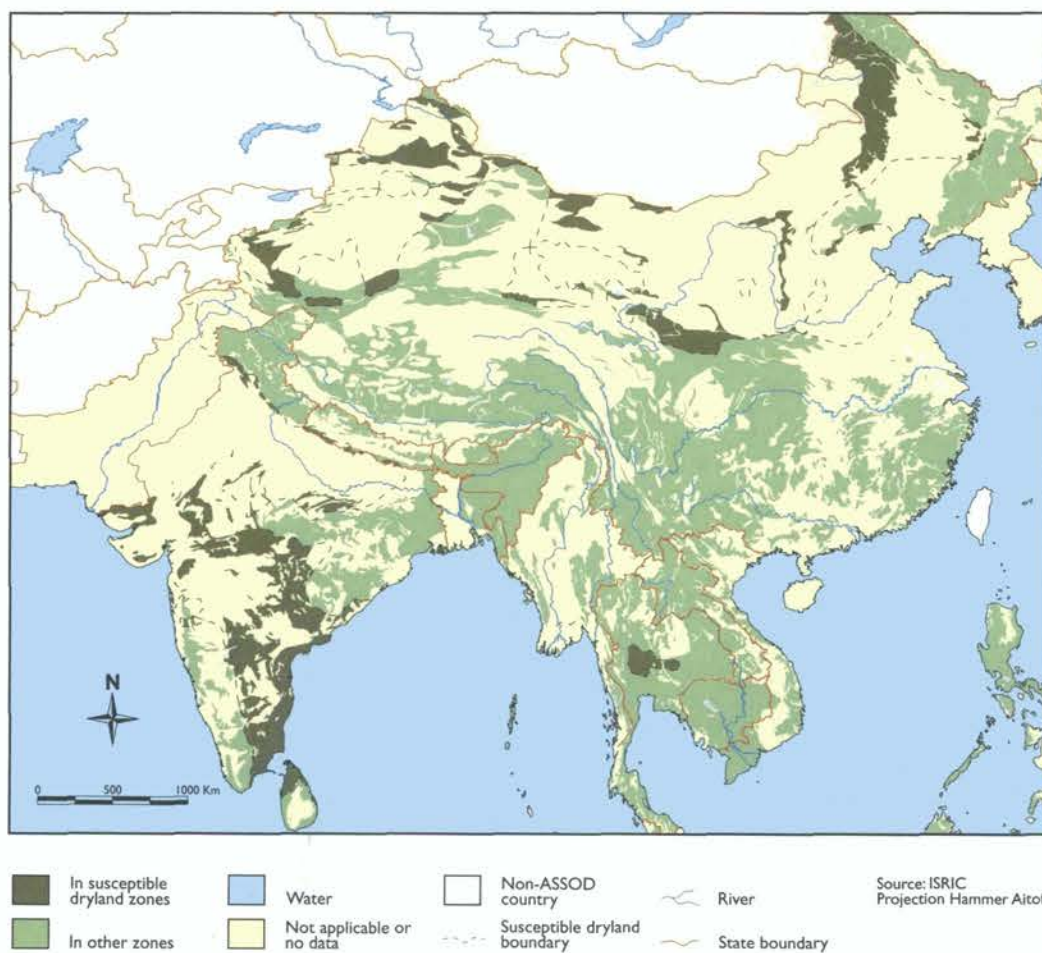
Map 3.12 Areas affected by deforestation
