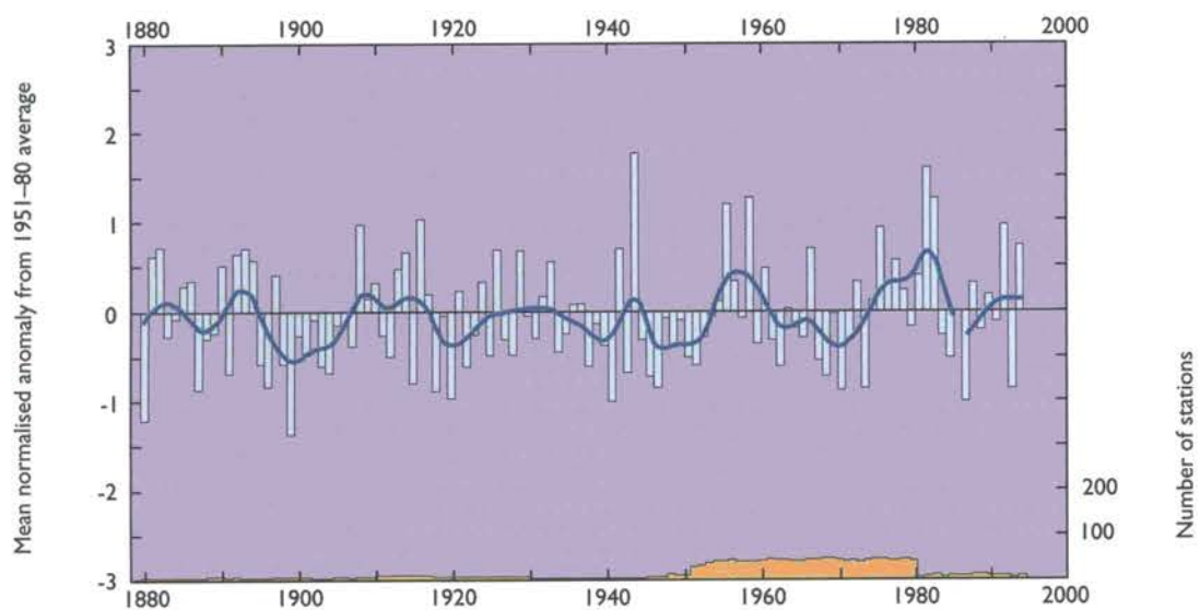
Figure 1.8 Pakistan annual rainfall, 1880–1994 (1951–80 mean = 435 mm). Source: CRU/UEA
