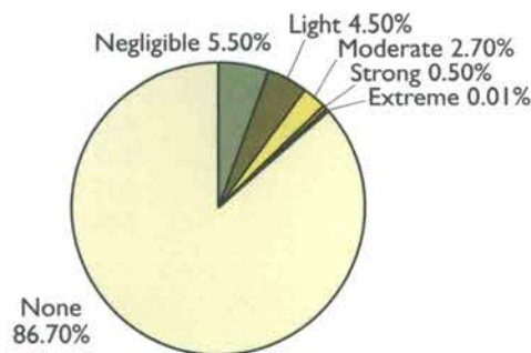
Figure 3.4 Chemical deterioration impact in ASSOD susceptible drylands. Source: ASSOD
