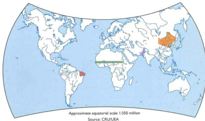
Map 1.6 Location of dryland regions referred to in Figures 1.5–1.8 (linked by colour)
