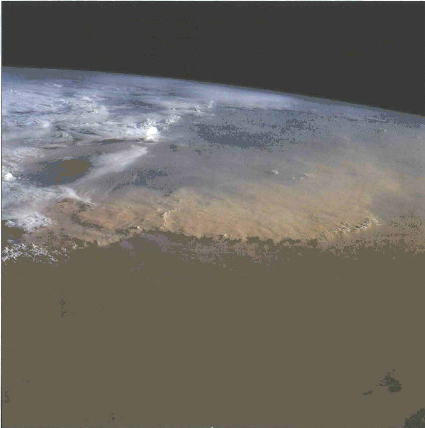
Figure 1.14 Dry, bare soils in arid environments can be susceptible to the liberation of fine particles as dust. In extreme cases, dust storms can have an impact beyond their source area. In this space shuttle photograph a major dust outbreak in the northern Sahel of Niger is moving west-south-west (NASA)
