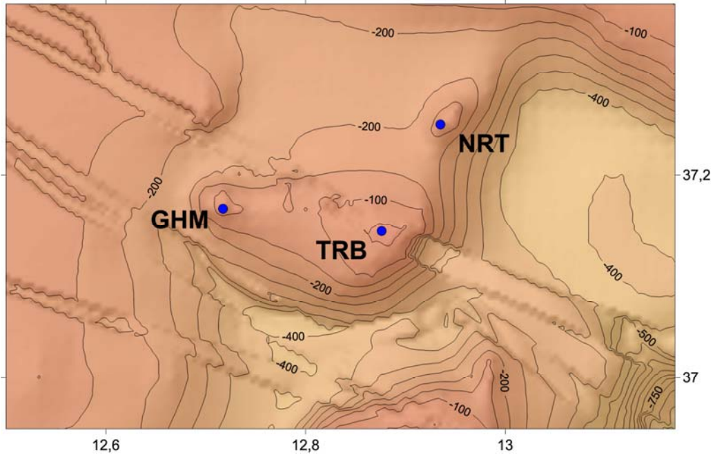
Fig. 5: Map of the Epedocle seamount, depth contours every 50 m. GHM, Graham bank; TRB, Terrible bank; NRT, Nerita bank.
