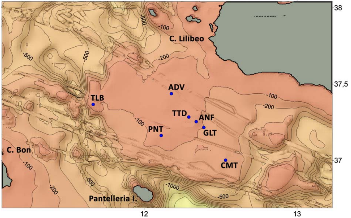
Fig. 4: Map of the Adventure bank, depth contours every 100 m. TLB, Talbot bank; ADV, Adventure bank; PNT, Pantelleria bank; TTD, Tetide volcano; ANF, Anfitrite volcano; GLT, Galatea volcano; CMT, Cimotoe, volcano.
