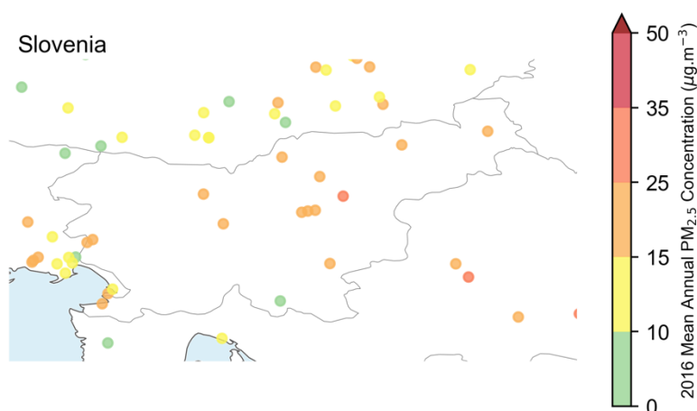
Figure Error! No text of specified style in document.-55: WHO mean annual PM 2.5 concentration observations in Slovenia (2016)
