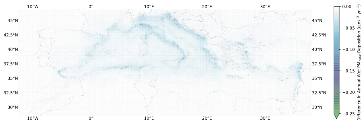
Figure -10. Decrease in annual wet PM Total deposition between MARPOL VI and the proposed Med SO x ECA
