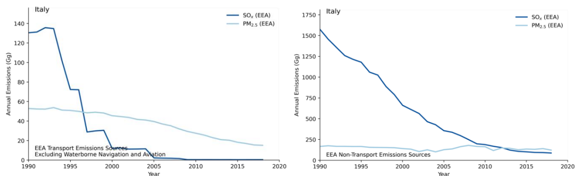
Figure Error! No text of specified style in document.-40: Transport (left) and non-transport (right) emissions of SO x and PM 2.5 in Italy
