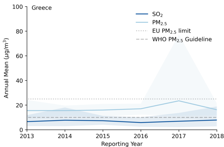
Figure Error! No text of specified style in document.-37: Annual mean concentrations of SO 2 and PM 2.5 in Greece (shaded areas show 95% CI)
