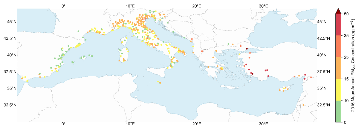
Figure Error! No text of specified style in document.-19: Mean annual air quality ( PM_{2.5} \mu\text{g}/\text{m}^3 ) observed at coastal observation stations (within 100 km of the coastline)
