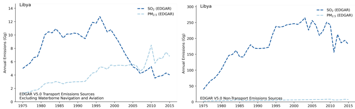
Figure Error! No text of specified style in document.-44: Transport (left) and non-transport (right) emissions of SO 2 and PM 2.5 in Libya
