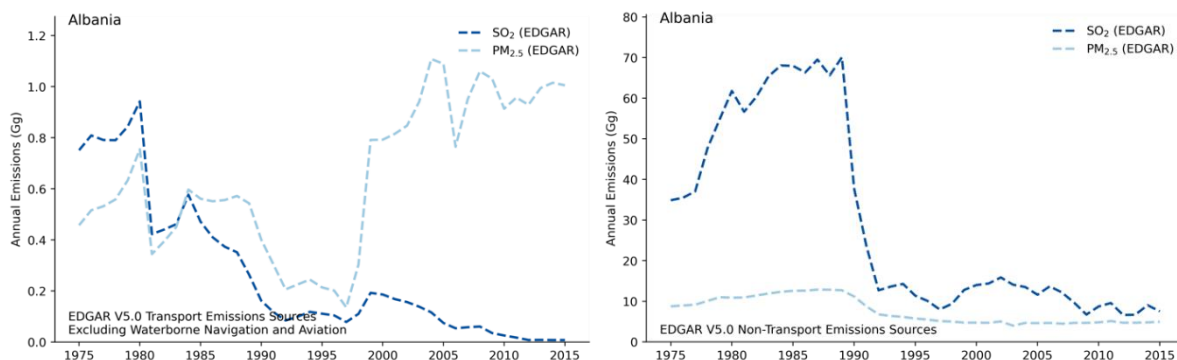
Figure Error! No text of specified style in document.-21: Transport (left) and non-transport (right) emissions of SO_2 and PM_{2.5} in Albania
