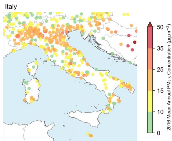
Figure Error! No text of specified style in document.-42: WHO mean annual PM_{2.5} concentration observations in Italy (2016)
