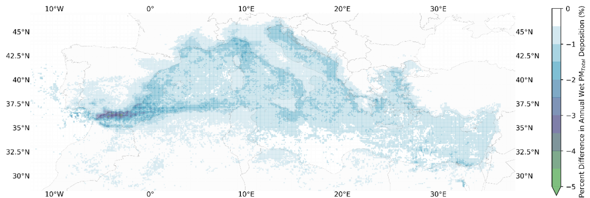
Figure-11. Percent decrease in annual wet PM_{Total} deposition between MARPOL VI and the proposed Med SO_x ECA
