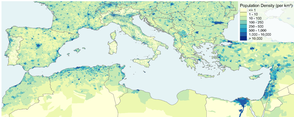
Figure -2. Gridded population in the Mediterranean coastal States
