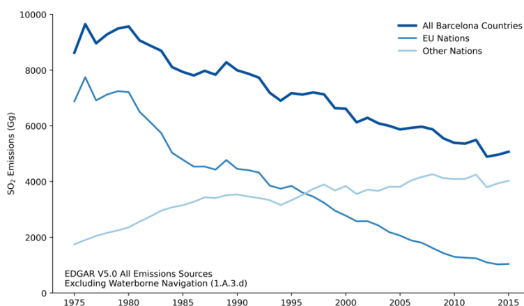
Figure-17: All sources of SO 2 emissions among Mediterranean coastal States that are Contracting Parties to the Barcelona Convention
