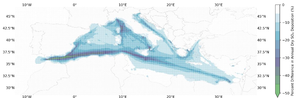
Figure 5.2-4: Percent decrease in annual dry sulphate deposition between MARPOL VI and the proposed Med \text{SO}_x ECA
