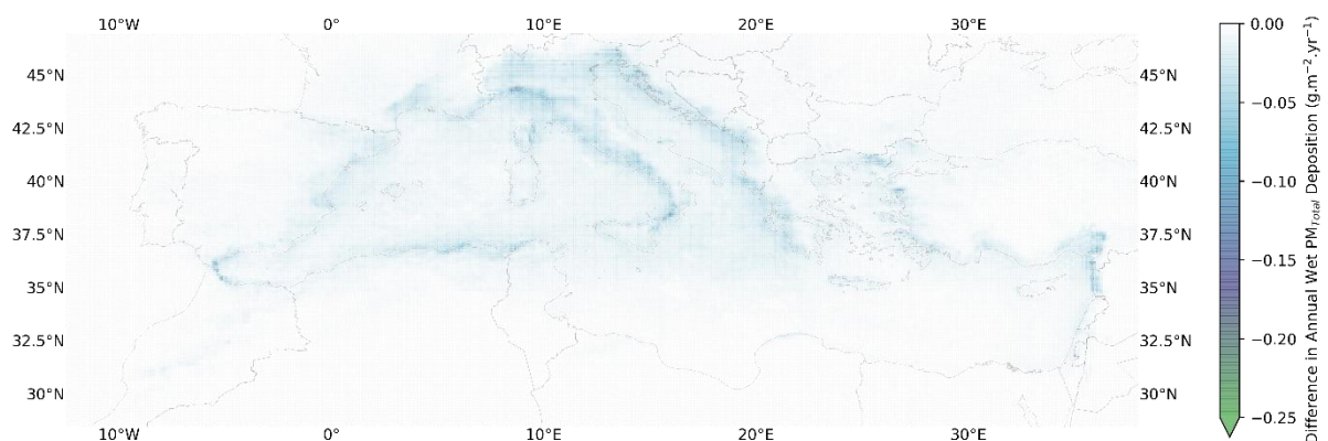
Figure 5.2-5: Decrease in annual wet \text{PM}_{\text{Total}} deposition between MARPOL VI and the proposed Med \text{SO}_x ECA
