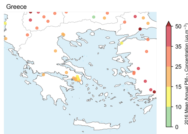
Figure 8.3-22: WHO mean annual \text{PM}_{2.5} concentration observations in Greece (2016)
