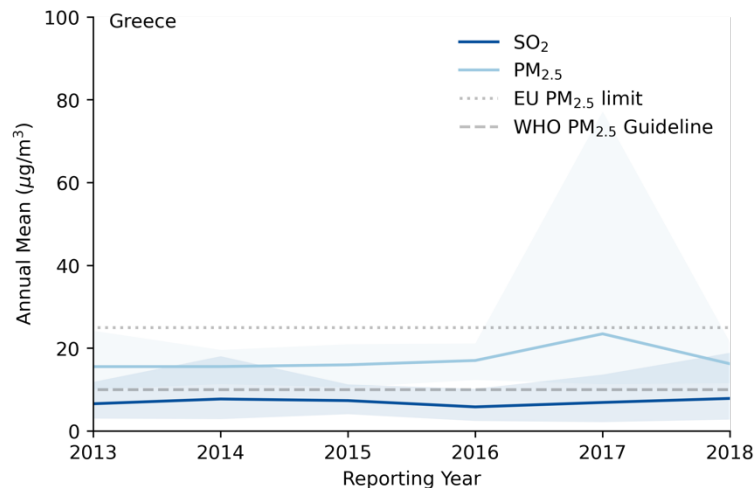
Figure 8.3-21: Annual mean concentrations of \text{SO}_2 and \text{PM}_{2.5} in Greece (shaded areas show 95% CI)
