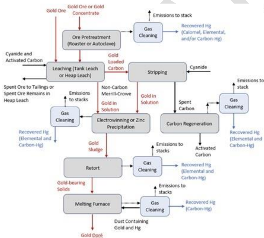
Figure 1: Example of gold production processing 9
