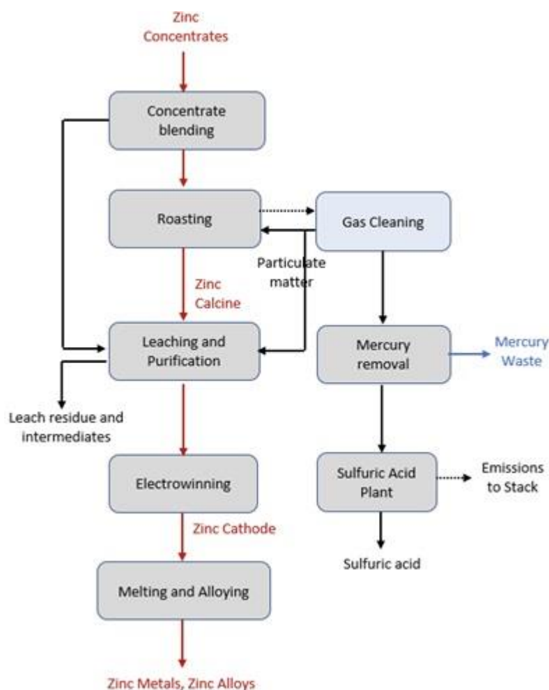
Figure 2: Zinc production process 9
