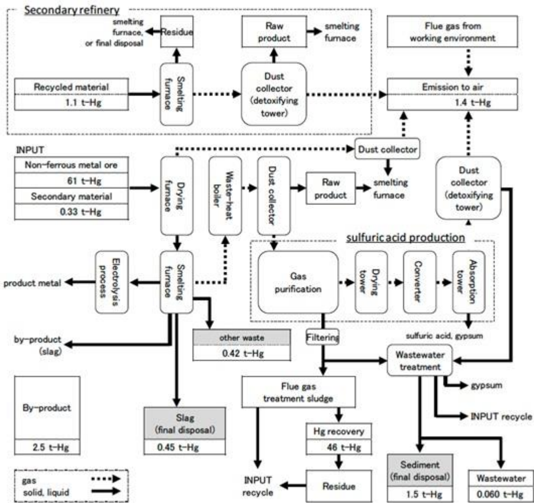
Figure 6: Mercury flow for non-ferrous metal smelting facilities in Japan (Ministry of the Environment Japan (MOEJ) 2018)
