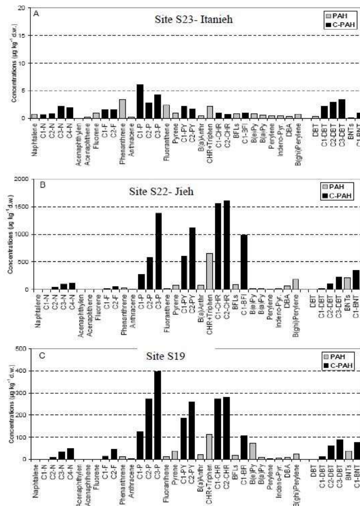
Figure 90. Chemical fingerprints of PAH and sulphur heterocyclic compounds in the three samples of mussels collected in the south of Lebanon (A, site S23 Itanieh), near the electric power plant in Jiyeh (B, site S22 Jiyeh) and in Beirut (C, site S19) (Khalaf et al., 2006 [32]).
