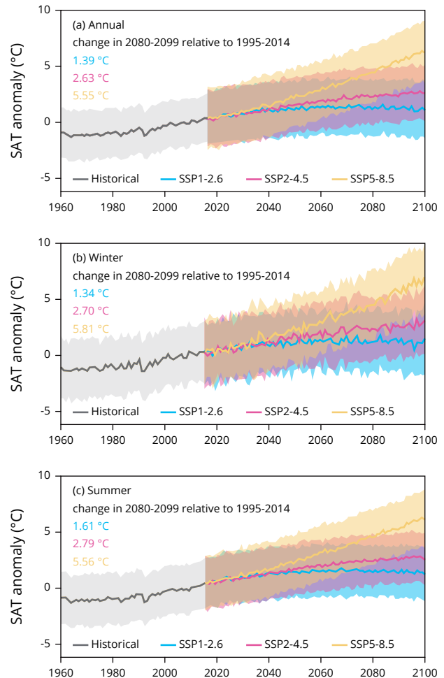
▲ Figure 4.1 Projected time series of (a) annual, (b) winter, and (c) summer surface air temperature anomalies
