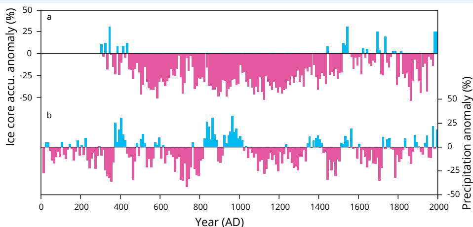
Δ Figure 2.2 Reconstructed precipitation variations in the TP over the past 2000 years through (a) Guliya ice core net accumulation, and (b) Dulan tree ring
