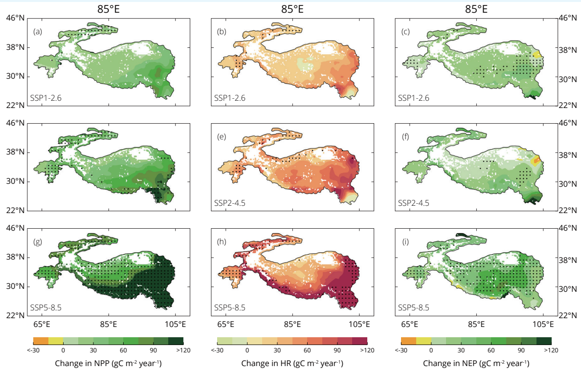
Figure 4.11 Spatial distributions of projected changes in NPP, HR and NEP
