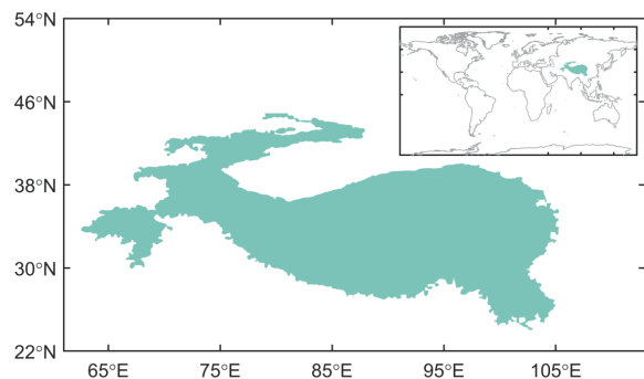
△ Source: The Shuttle Radar Topography Mission (SRTM) data at 90 meter (3 arc-second) resolution.
