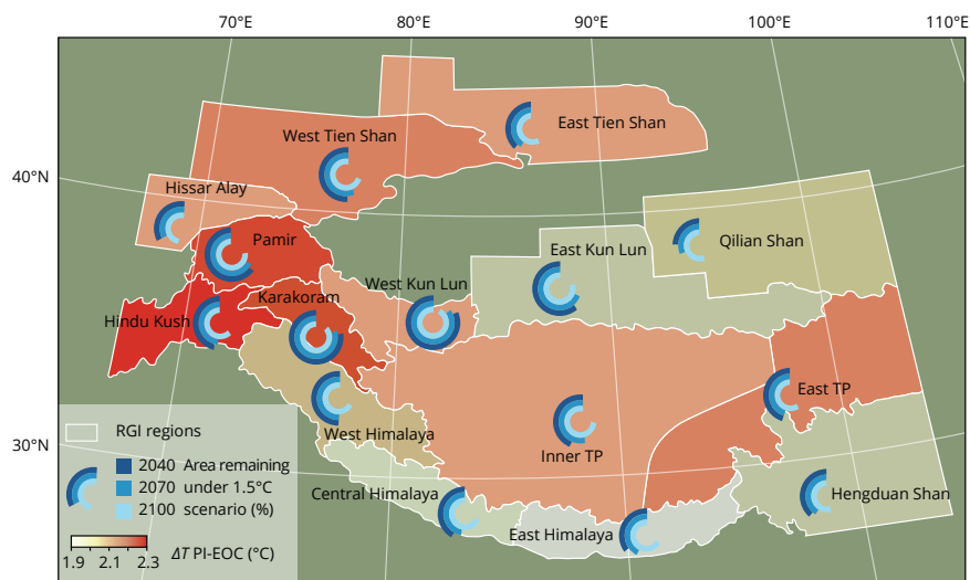
▲ Figure 4.5 Regional temperatures and projected glacier area associated with a 1.5°C increase
