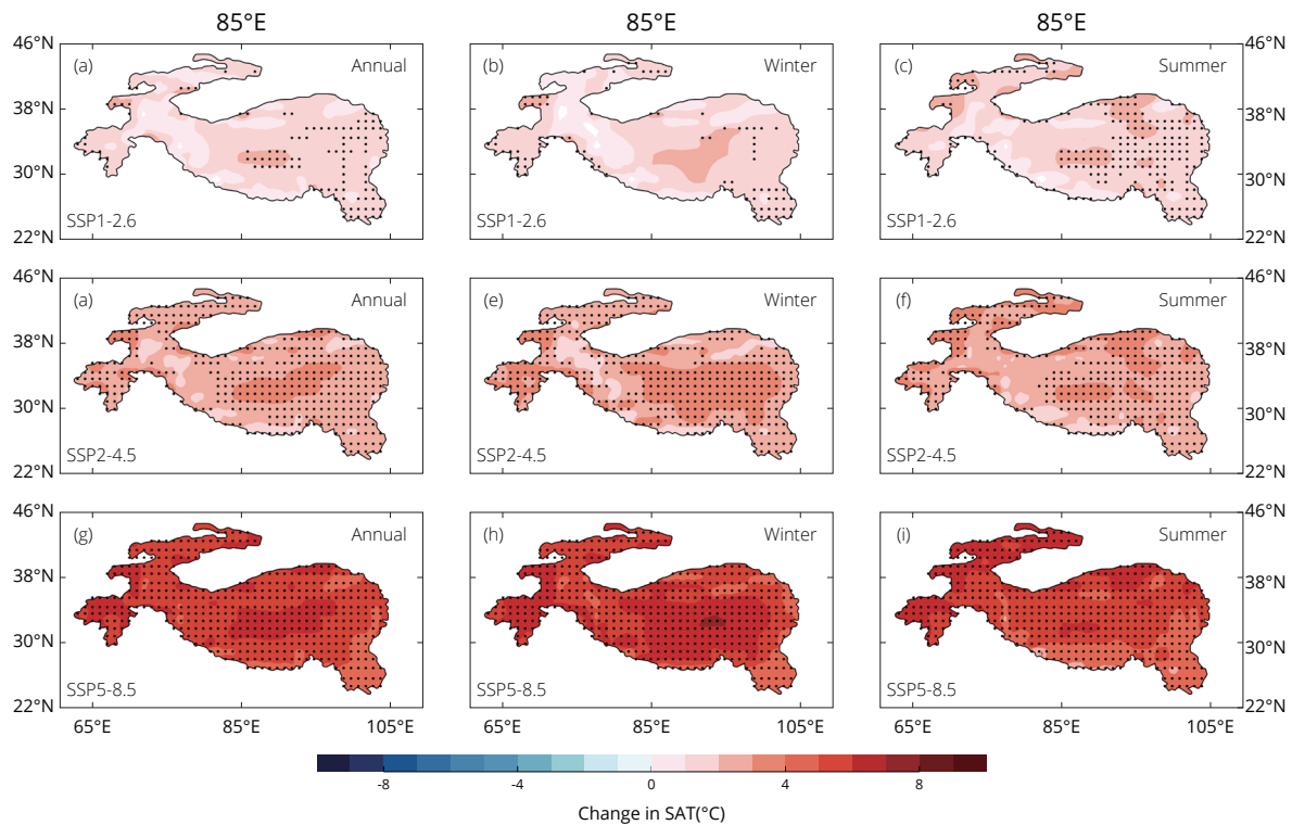
Δ Figure 4.2 Spatial patterns of annual, winter and summer surface air temperature anomalies
