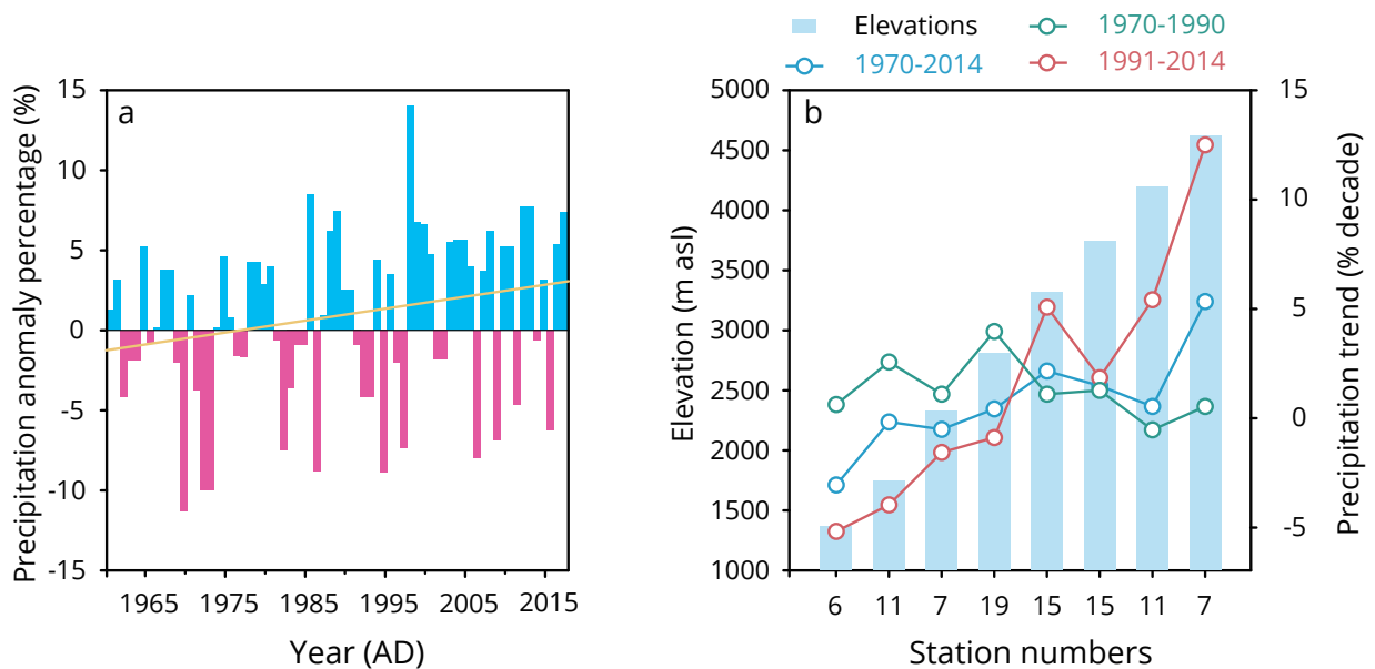
△ Figure 2.5 (a) Anomaly of annual mean precipitation in 95 TP meteorological stations, (b) elevation dependence of trends (per decade) in summer precipitation throughout the TP.
