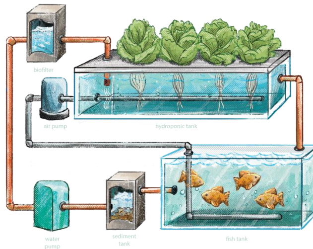
Figure 9. Flow diagram for Aquaponics. Sources: Earth.org
