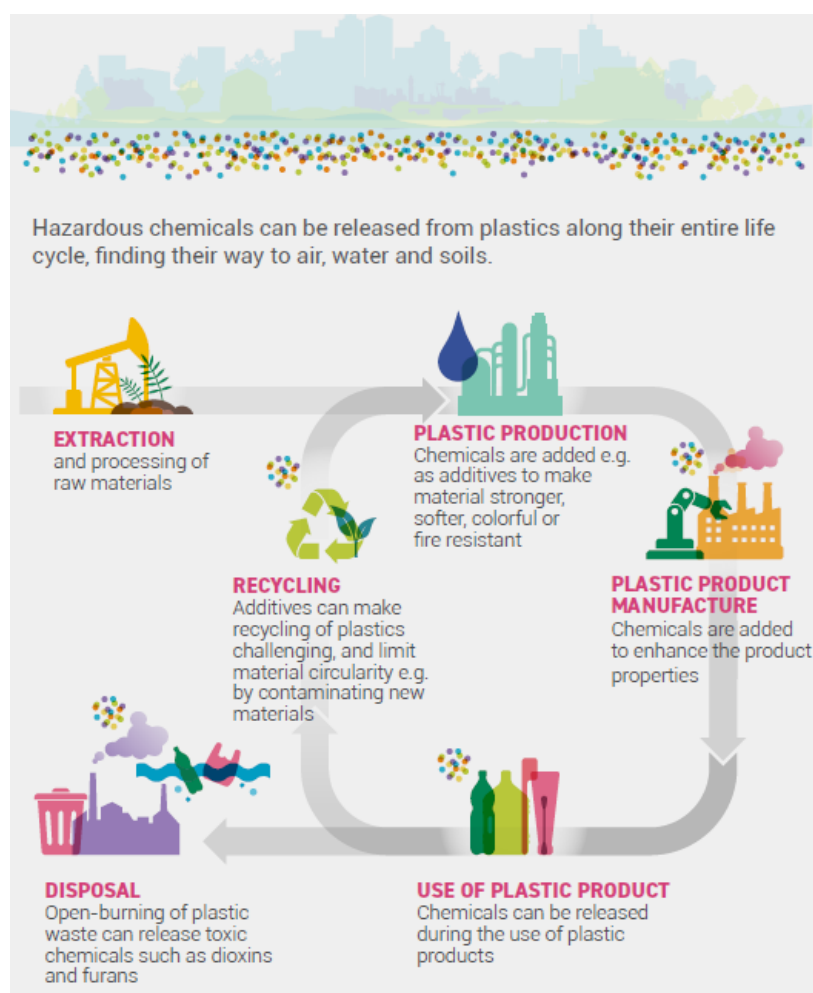
Figure 1. Chemicals along the plastic life cycle
