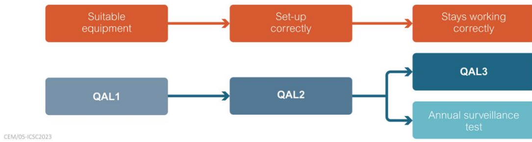
Figure 5 Process flow representation of QAL levels under EN 14181 (CEN, 2021)
