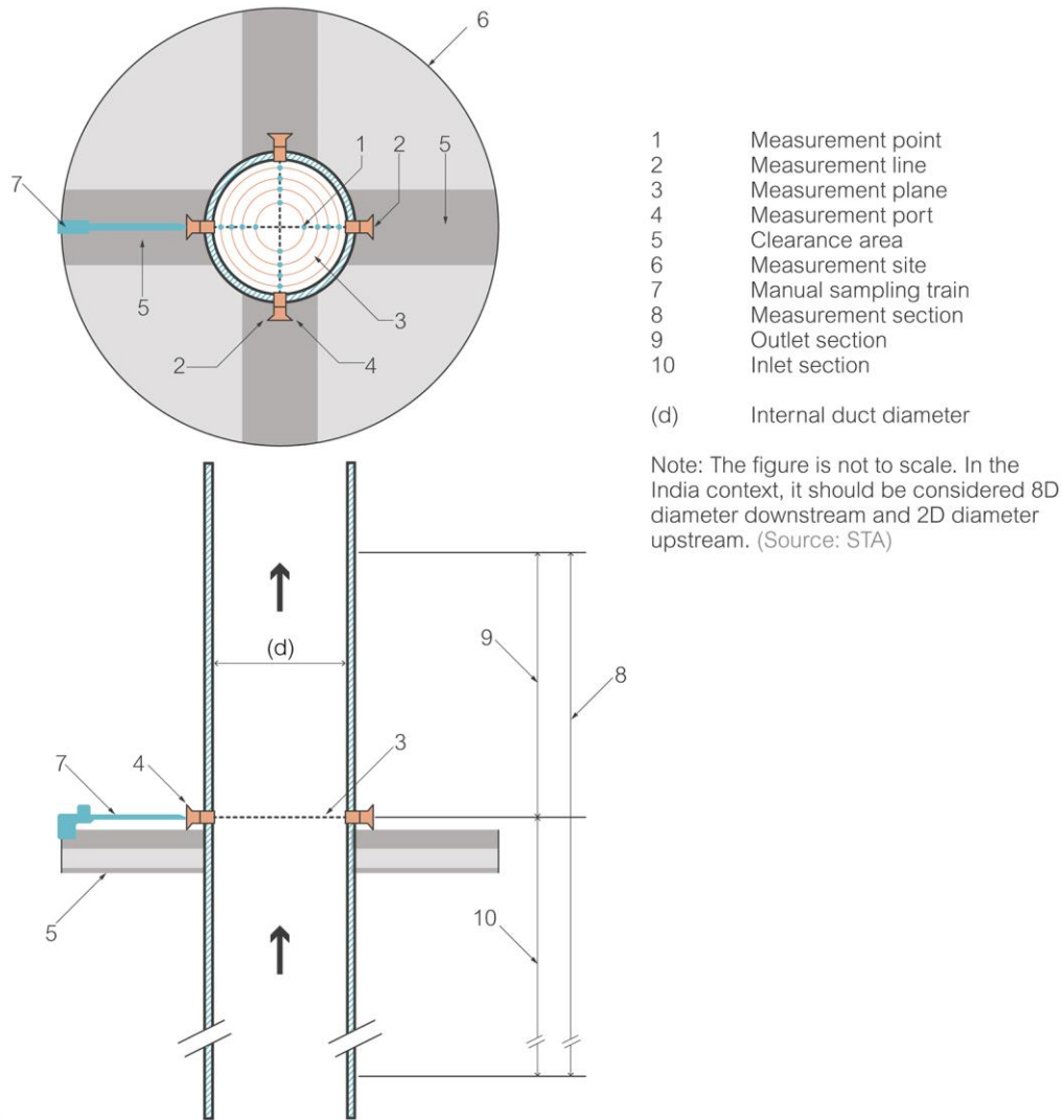
Figure 2 Measurement site and sectioning of stack for CEMS installation (CPCB, 2018)
