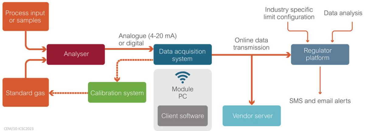
Figure 10 Direct data transmission set-up for remote calibration of CEMS (Kanchan, 2019a)
