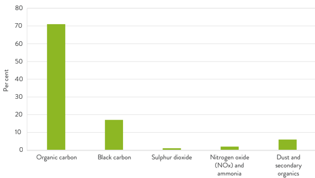
Figure 5.3 Africa, the contribution of different anthropogenic pollutant emissions to population-weighted fine particulate matter from the GISS model, 2030, per cent
