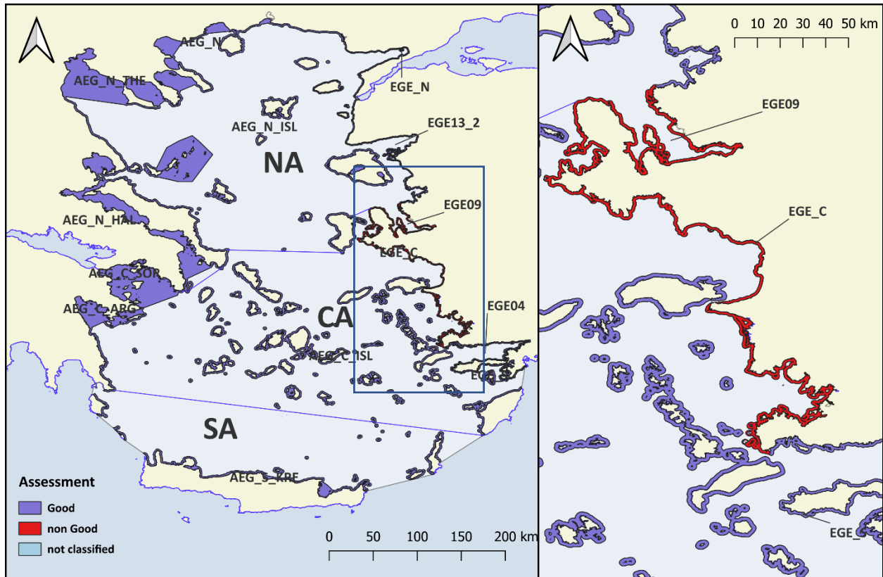
Figure AEL 3.1.3.1.5.E: The assessment results for CI 14 in the Aegean Sea Sub-division by applying the simplified G/M method on the satellite-derived COPERNICUS data at the level of subSAUs.
