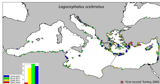
Distribution of Lagocephalus sceleratus in the Mediterranean Sea. First record(s) annotated with an asterisk, different colour symbols correspond to different 6-year reporting periods, corresponding frequency histograms depict number of records in each time bin.
