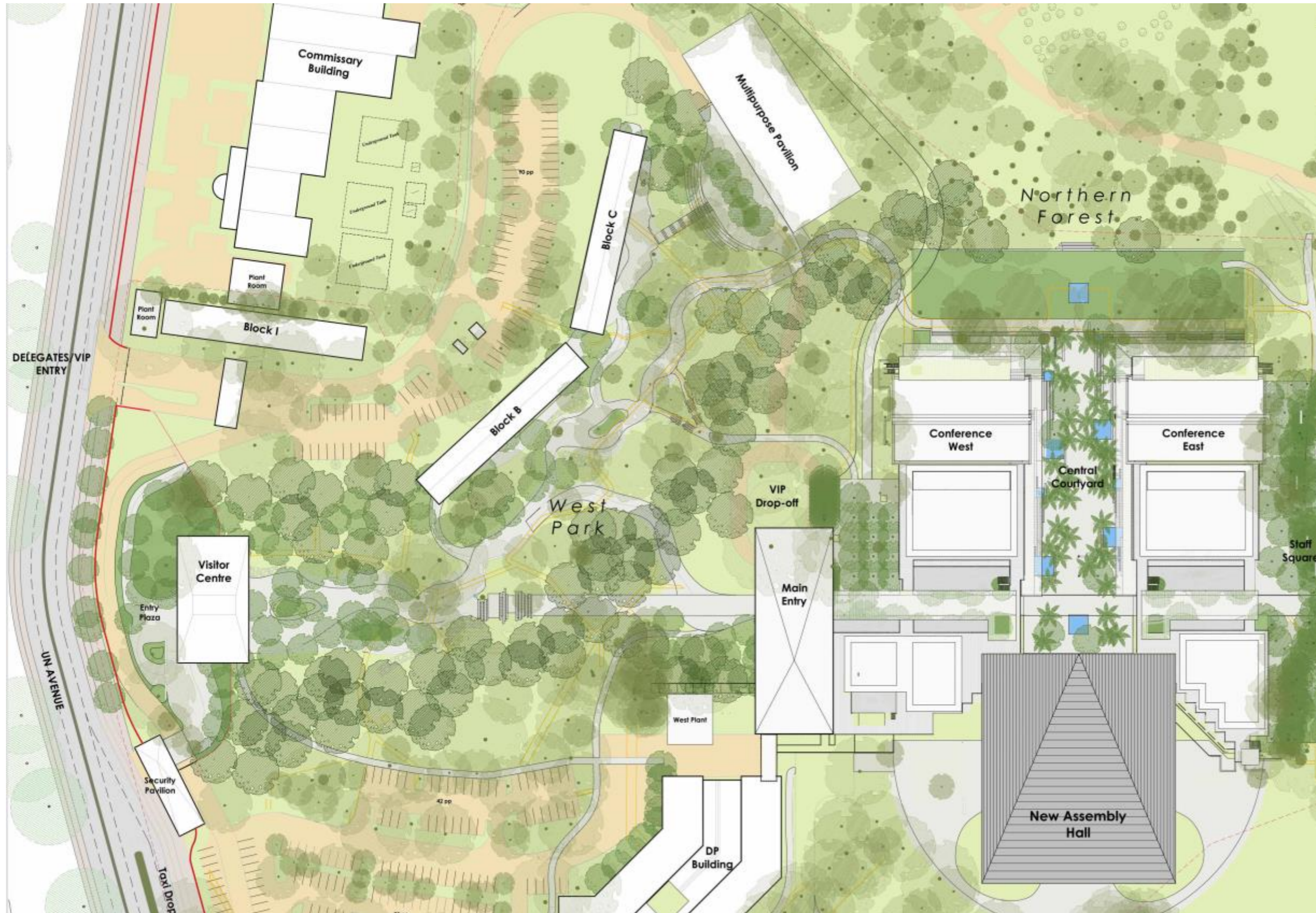
SITE PLAN
