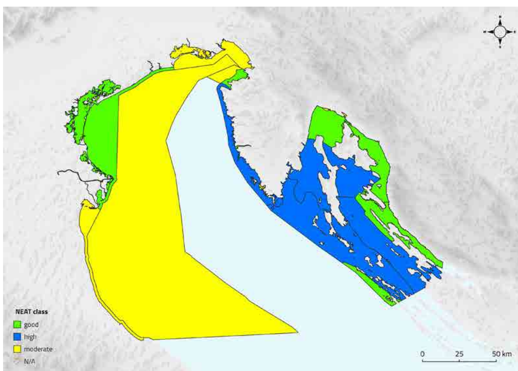
Figure 73: The NEAT assessment results for IMAp C17 in the North Adriatic Sea. Aggregation of all contaminants per sub-SAU. Blank area corresponds to no available data/decision or not established monitoring.
