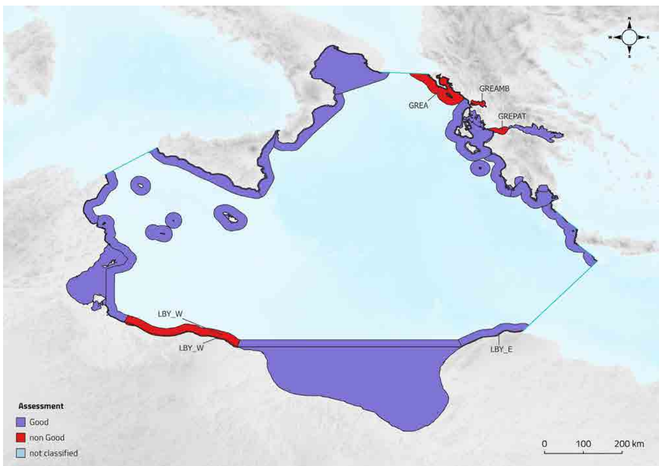
Figure 40: The assessment results for CI 14 in the CEN Sub-region by applying the simplified G/M method at the level of subSAUs.
