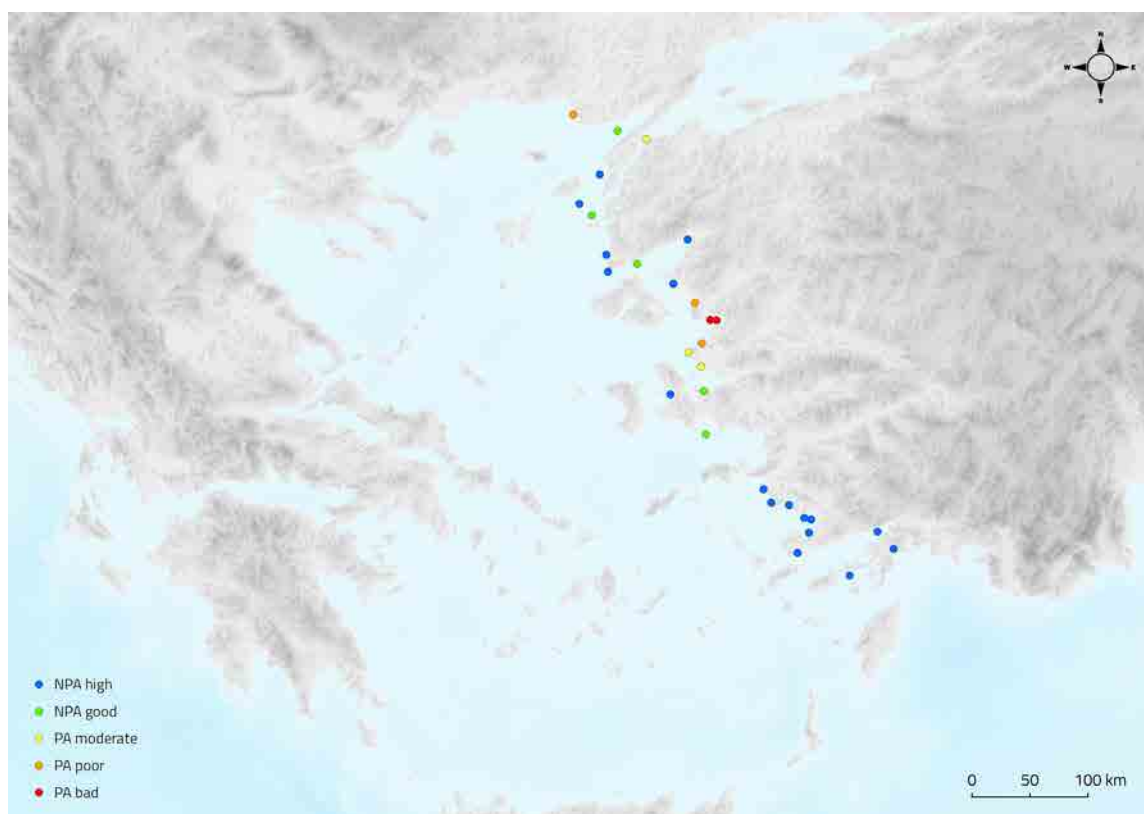
Figure 62: Results of the CHASE+ assessment methodology to assess the environmental status of \Sigma 7 PCBs in sediments in the AEGS, using AEL_BACs as thresholds. Stations in blue - NPAhigh (CR=0.0-0.5); stations in green- NPAgood (CR =0.5-1.0); Stations in yellow- PAmoderate (CR =1.0-2.0); stations in brown - PApoor (CR =2.0-5.0) and stations in red - PAbad (CR > 5.0). Blue and green stations are considered in GES; yellow, brown and red stations are considered non-GES.
