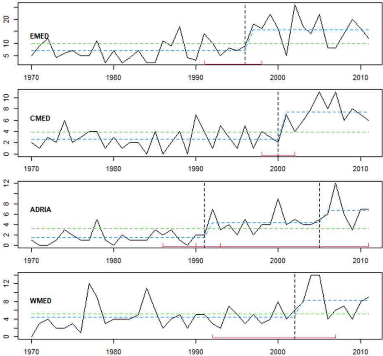
Figure 184: Number of new NIS introductions per year (y-axis) in different Mediterranean subregions for the period 1970-2011 (continuous black line) with breakpoints and fitted mean values superimposed: vertical dashed line indicates breakpoint or year of significant change in the mean values of new NIS, with 95% confidence intervals around the breakdate (CIs) in red brackets; dashed green line shows the null model of no temporal change in new NIS numbers; and dashed blue line represents fitted mean values before and after the identified breakpoint.
