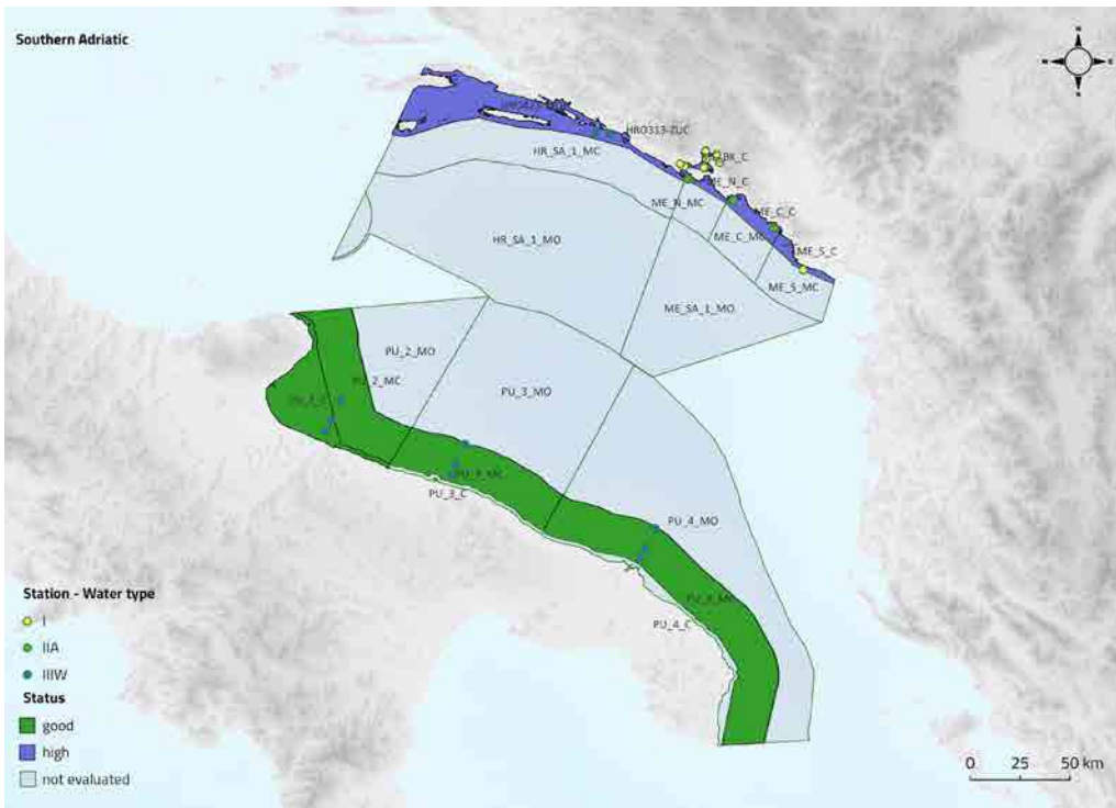
Figure 35: The NEAT assessment results for IMAP Cls 13 and 14 in the South Adriatic Sea. All IMAP SAUs are in GES, characterized by High or Good status. Blank area corresponds to no available data.
