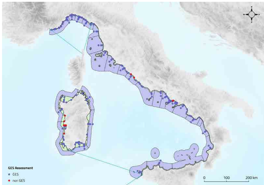
Figure 57: Result of the GES assessment by applying the EQR methodology in the Italian waters in the Tyrrhenian Sea and CWMS at the level of subSAUs.
