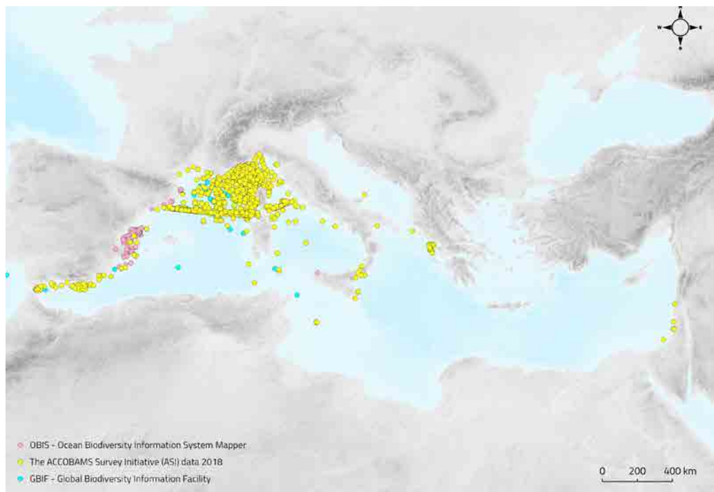
Figure 164: Balaenoptera physalus occurrence data from INTERCET Project. Source: INTERCET Presentation map https://www.intercet.it/
