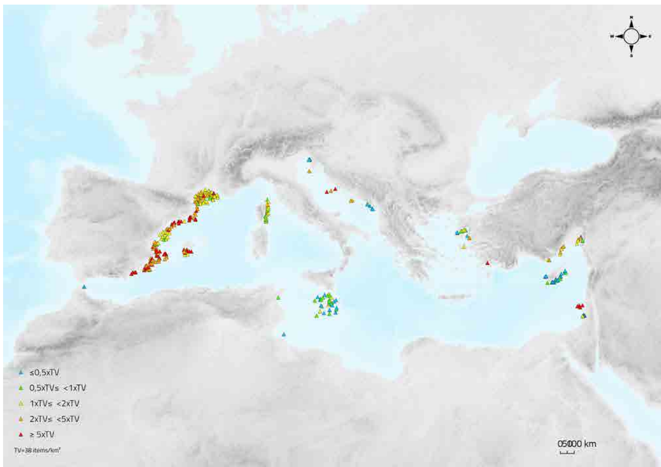
Figure 117: GES assessment classification of the seafloor stations monitored for marine litter in the Mediterranean Region.
