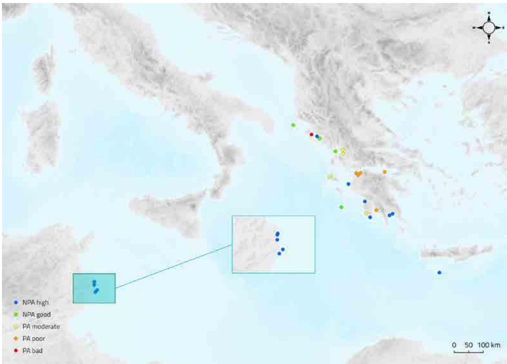
Figure 69: Results of the CHASE+ approach to assess the environmental status of \Sigma 16 PAHs in sediments in the CEN, using MED_BACs as thresholds. Stations in blue - NPAhigh (CR=0.0- 0.5); stations in green- NPAgood (CR=0.5- 1.0); Stations in yellow- PAmoderate (CR =1.0-2.0); stations in brown - PApoor (CR =2.0-5.0) and stations in red - PAbad (CR > 5.0). Blue and green stations are considered in GES; yellow, brown and red stations are considered non-GES. Part of the coastal area of Tunisia was enlarged to improve visibility and clarity (i.e. area delimited by broken line).
