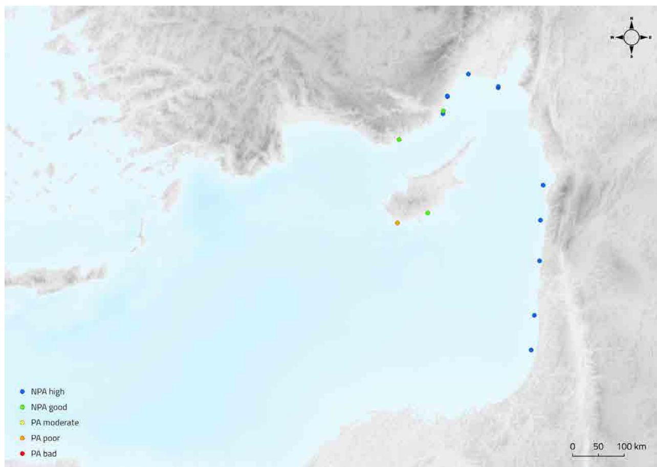
Figure 67: Results of the CHASE+ assessment methodology application to assess the environmental status of TM in M. barbatus in the LEVS, using AEL_BACs as thresholds. Stations in blue - NPAhigh (CS=0.0-0.5); stations in green- NPAgood (CS =0.5-1.0); Stations in yellow- PAmoderate (CS =1.0-2.0); stations in brown - PApoor (CS =2.0-5.0) and stations in red - PAbad (CS > 5.0). Blue and green stations are considered in-GES; yellow, brown and red stations are considered non- GES.
