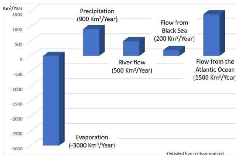
Figure 2: Annual hydrological balance of the Mediterranean Sea
