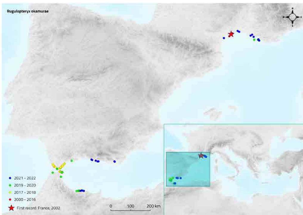
Figure 196: Distribution of Rugulopteryx okamurae in the Mediterranean Sea. Details as in Figure 187.
