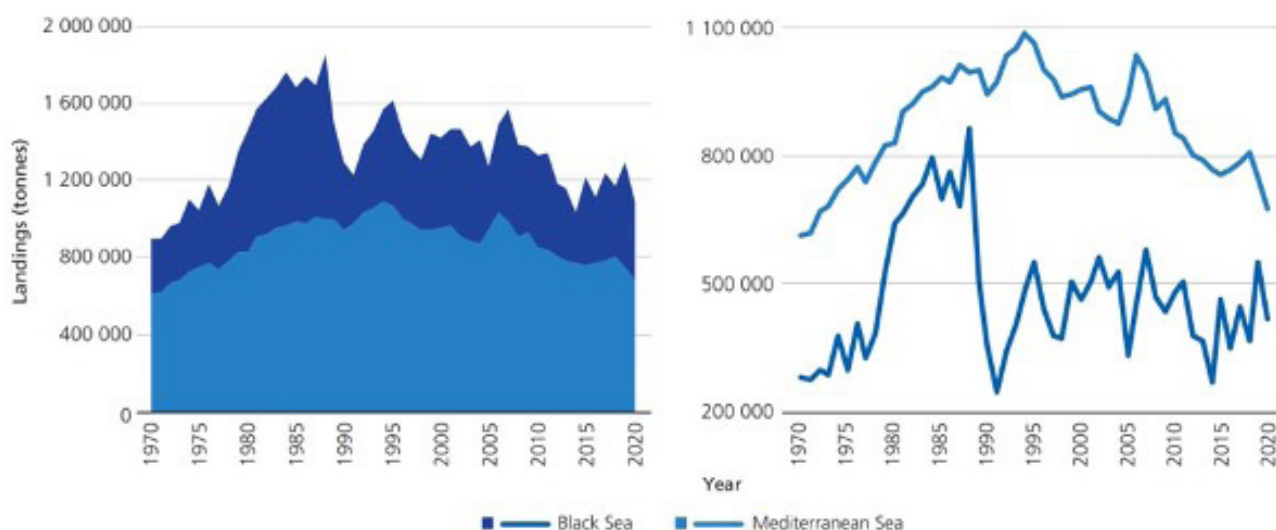
Figure 203: Total landings in the Mediterranean and the Black Sea per year, 1970–2020
