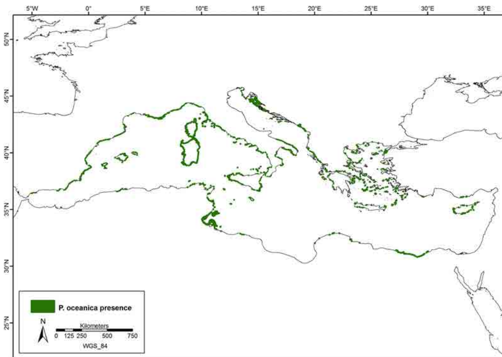
Figure 136: Distribution of Posidonia oceanica meadows in the Mediterranean Sea (green areas) (from Telesca et al. 2015).
