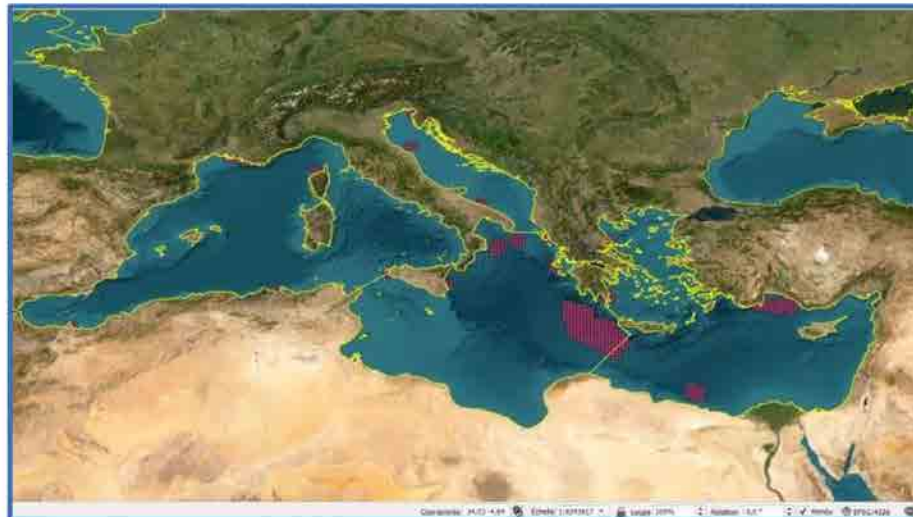
Figure 96: Impulsive noise events data for 2021. Each purple cell indicates the position of impulsive noise events, meaning that the impulsive noise emissions occurred during at least 1 day in that cell.
