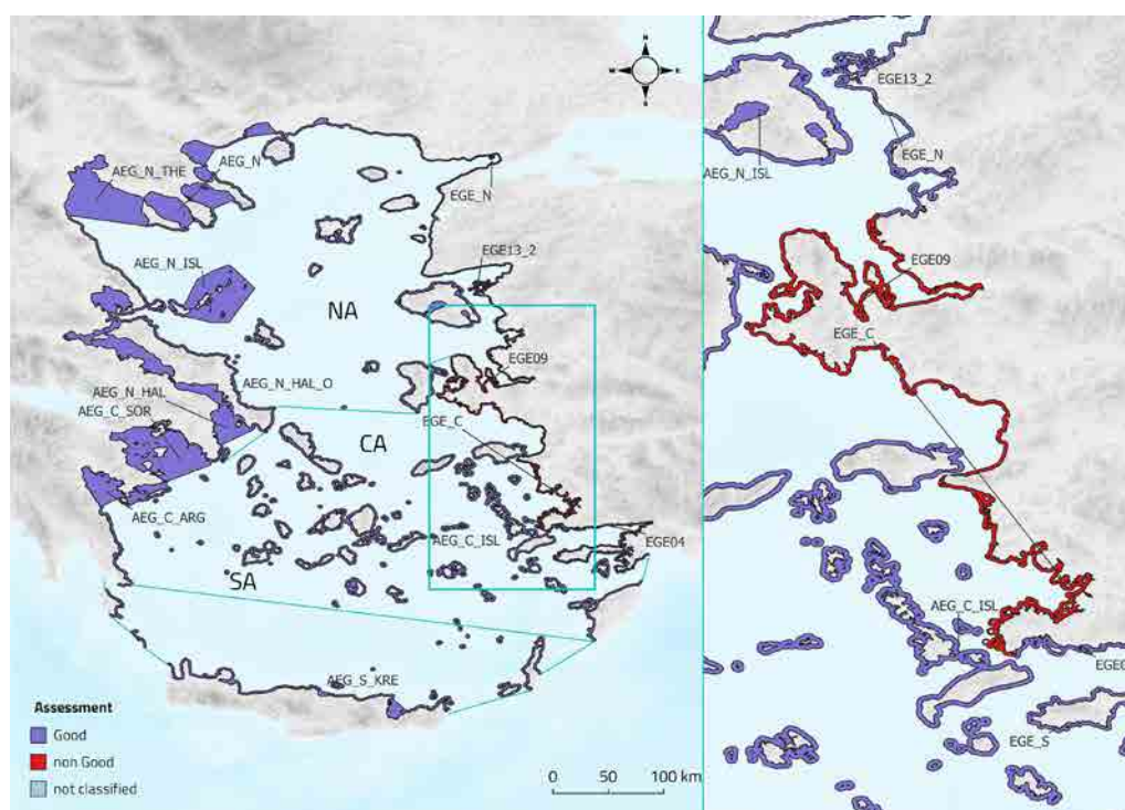
Figure 30: The assessment results for CI 14 in the Aegean Sea Sub-division by applying the simplified G/M method on the satellite-derived COPERNICUS data at the level of subSAUs.
