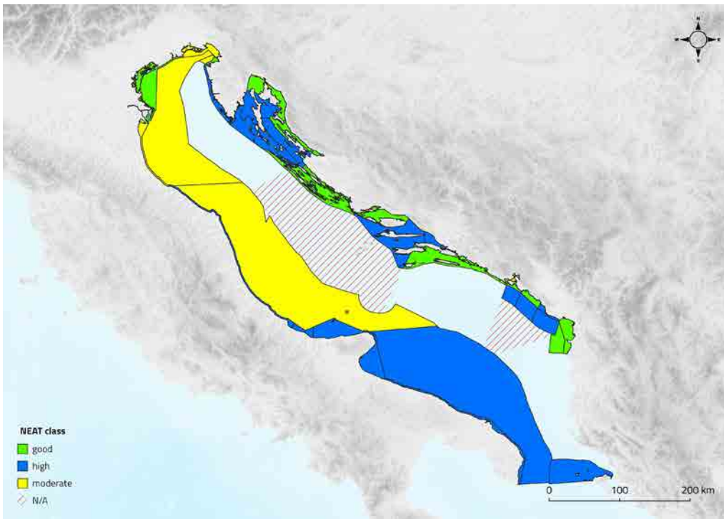
Figure 76: The NEAT assessment results for IMAP CI17 in the Adriatic Sea sub-region. Aggregation of all contaminants per sub-SAU. Blank area corresponds to no available data/decision or not established monitoring.
