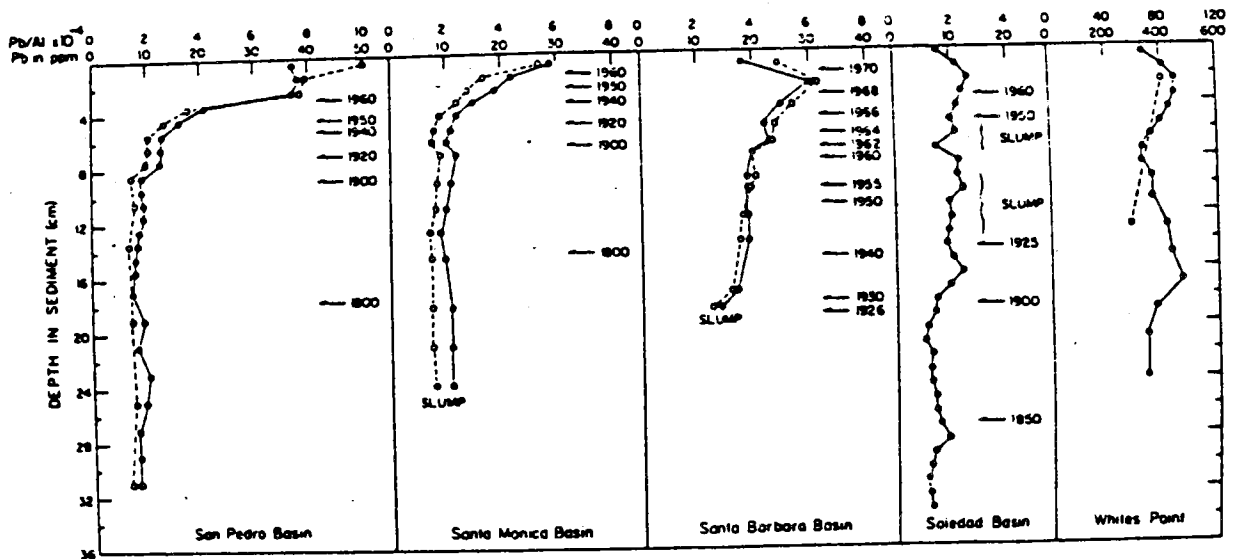
Fig. 4. Lead content (•) and lead/aluminum ratios (o) in Southern California Basin sediments, and Whites Point sewer outfall sediments; note change of scale, Whites Point. Vertical dating of sediments is indicated. From: Bertine (1980).
