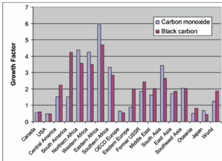
FIGURE 3 Black carbon emission growth factors from 2000 to 2030 by selected world regions and by source sector.
