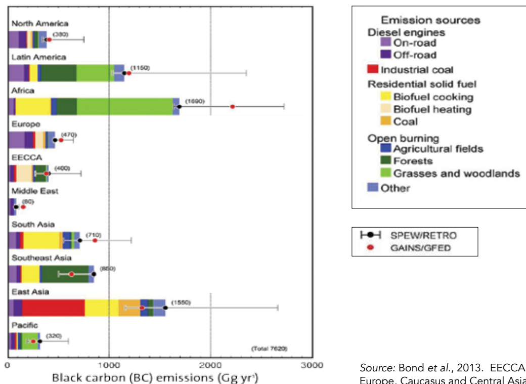
FIGURE 2 Black carbon emissions (kt / year) by region and source sector in 2000.
