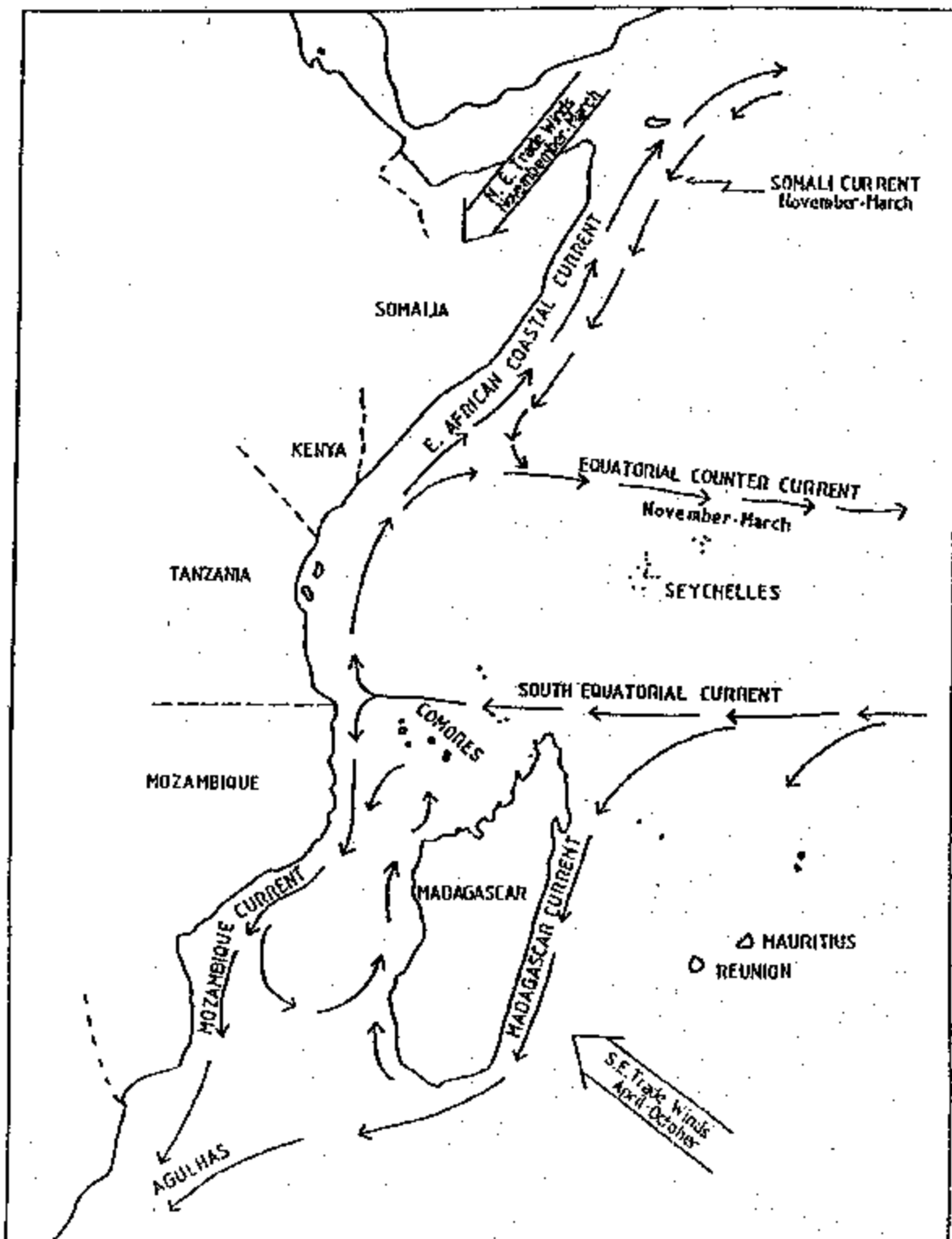
Figure 2. Ocean currents and winds in the Eastern African Region (After IUCN/UNEP 1982)
