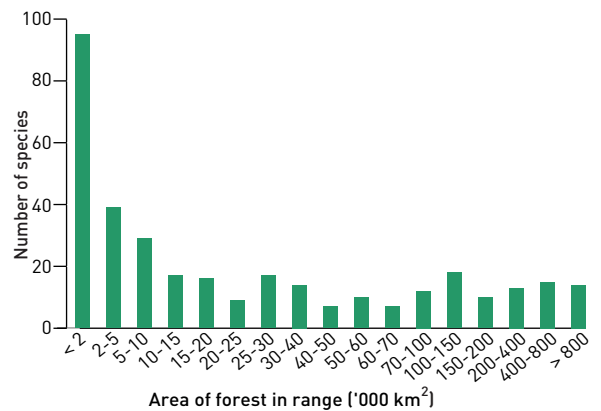
Figure 5. Number of bamboo species in the Americas with different areas of forest remaining within their geographical ranges. Species that are dependent on forest and have less than 20 000 km 2 of forest in their ranges should be considered as threatened in any preliminary assessment of conservation status.
