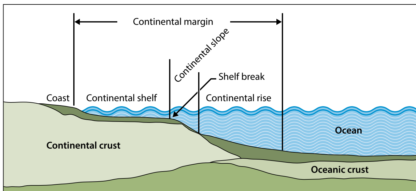
Figure 8.1. Schematic of the components of a generalized passive continental margin.
