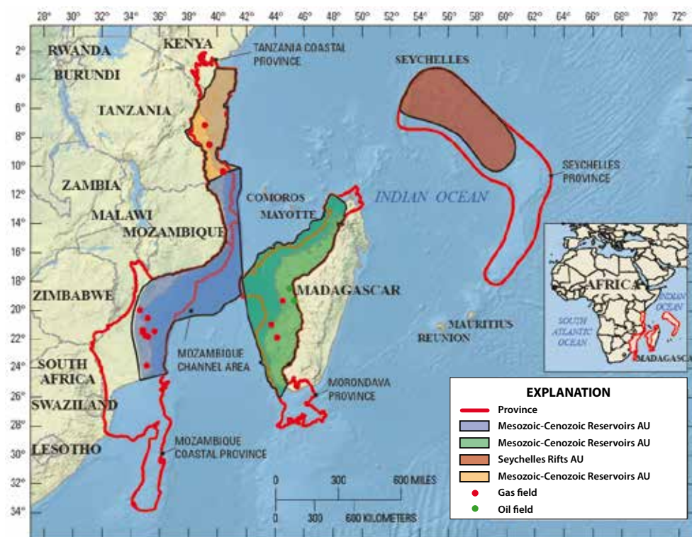
Figure 26.1. Locations of the four assessed geological provinces and assessment units (AU) in the WIO region. Source: Brownfield and others (2012).
