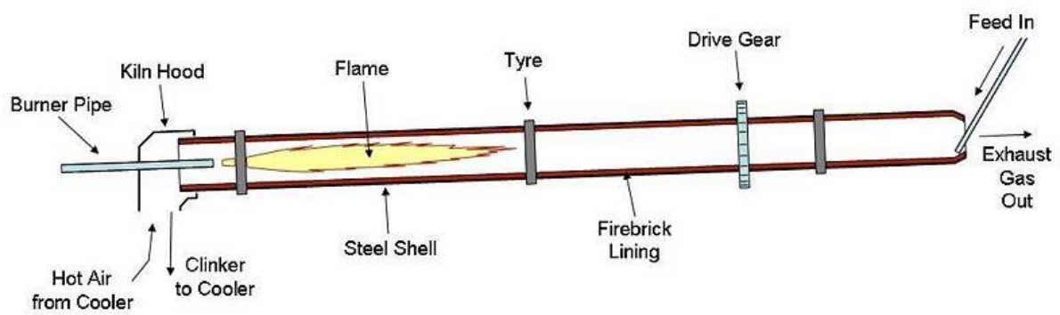
Fig. 25: Example of rotary kiln [30]
