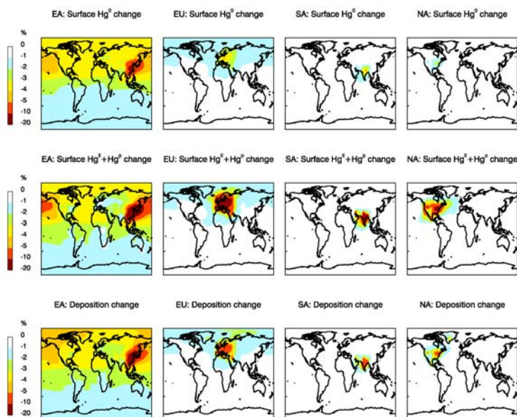
Figure 18.3 - Percentage change in annual surface concentrations of Hg^0 and Hg^{II}+Hg^P (top 2 rows) and in deposition (bottom row) for each perturbation simulation. The perturbation simulations are shown from left to right: East Asia (EA), Europe and North Africa (EU), South Asia (SA), and North America (NA).
