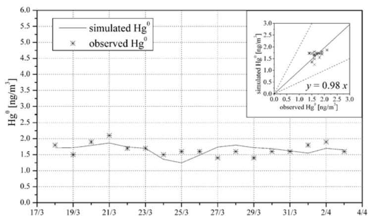
Figure 13.11 - The measured and calculated \text{Hg}^0_{(g)} concentration during the Med-Oceanor 2004 oceanographic campaign. (Hedgecock et al. 2006).
