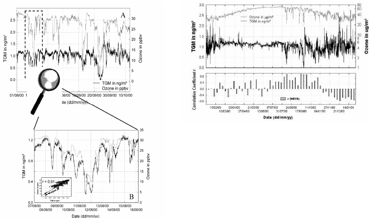
Figure 10.5 - Ozone and TGM concentrations during the AMDEs observed at Neumayer, Antarctica from August to October 2000 (Reprinted with permission from Ebinghaus et al., 2002 and Temme et al., 2003. Copyright 2002 and 2003 American Chemical Society).
