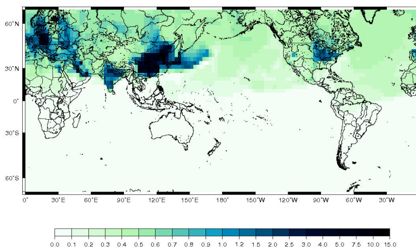
Figure 19.15 - Changes (control run minus reduction experiment) in \text{Hg}^0 concentration [ppq] with a reduction of 20% in all 4 source regions, Jan-Mar 2001.
