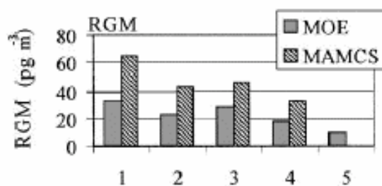
Figure 9.21 - Average TGM, IPM and RGM values obtained at campaign MOE 1-5 and MAMCS 1-4. The IGM value from the MAMCS campaign 4 should be regarded with some caution since it is based on measurements from two sites only.
