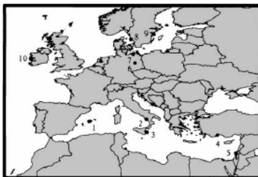
Figure 9.18 - The measurement sites: 1. Mallorca (39°40'30" N, 2°41'36"E); 2. Calabria (39°25'N, 16°00'E); 3. Sicily (36°40'N, 15°10'E); 4. Turkey (36°28'12"N, 30°20'24"E); 5. Israel (32°40'N, 34°56'E); 6. Germany (53°08'34"N, 13°02'00"); 7. Germany (54°26'14"N, 12°43'30"E); 8. Sweden (57°24'48"N, 11°56'06"E); 9. Sweden (58°48'00", 17°22'54"E); 10. Ireland (53°20'N, 9°54'W)
