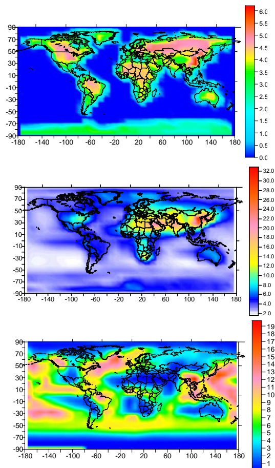
Figure 21.2 - Atmospheric deposition of mercury ( \mu\text{g}/\text{m}^2\text{-y} ) in the base simulation: Top: Hg(0) dry deposition; middle: Hg(II) dry deposition; bottom: Hg(II) wet deposition.
