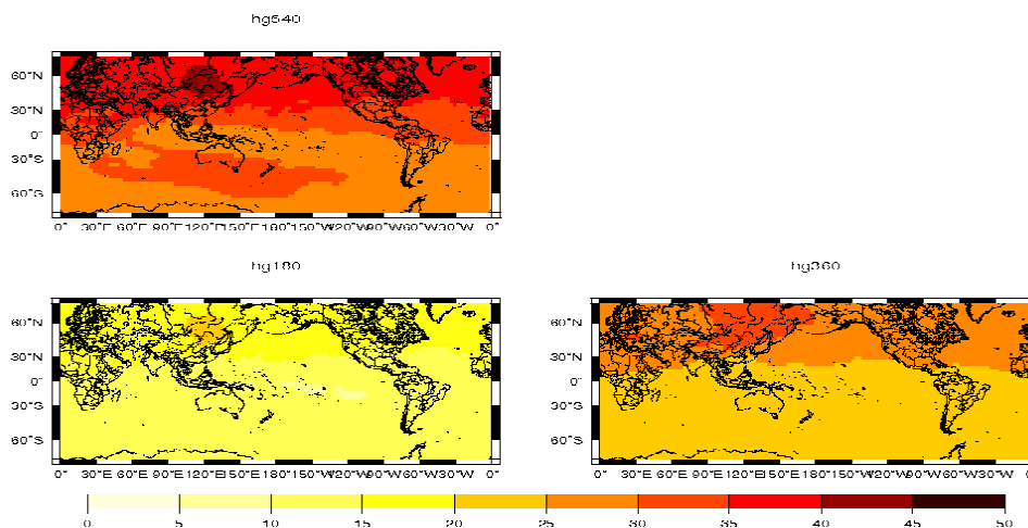
Figure 19.9 - Hg-like tracers with different lifetimes [days], concentration [ppq] in 500 hPa.
