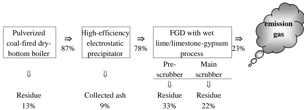
Figure 5-1 Reducing mercury emissions with wet FGD systems; mercury flows and outputs in % of mercury input to boiler based on Pacyna and Pacyna (2000) (figure from UNEP, 2002)
