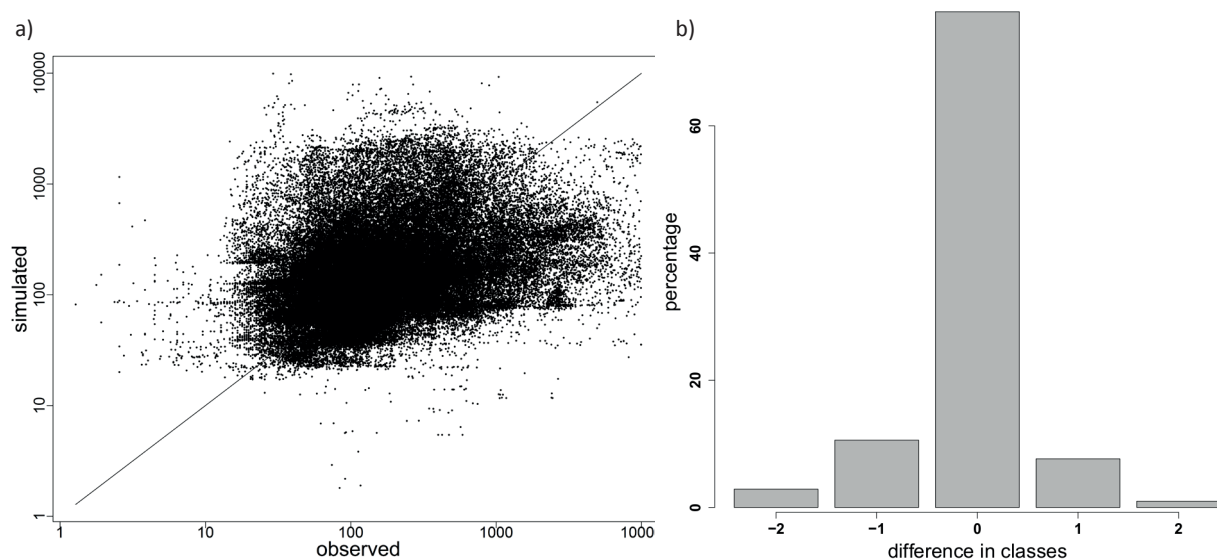
Figure B.5: a) Observed versus calculated (WorldQual) total dissolved solids for the period 1990–2010 for stations from Latin America, Africa, and Asia between 1990 and 2010. Units are in mg/l. b) Measured and simulated TDS in-stream concentrations were grouped into three water pollution classes which were derived from thresholds given by governments and international organizations. The difference in classes between observed and simulated in-stream concentrations was determined and displayed as percentage of grid cells (having measurements) in which a difference occurred between the observed class (see Table 3.12) and the computed pollution class. “0” indicates that there was no difference between the observed and computed pollution class. GEMStat data are not used for this scatter plot so as to avoid overlap with the stations used to estimate TDS background concentrations (Section B1.2.9). Also stations influenced by marine saltwater intrusion were omitted.
