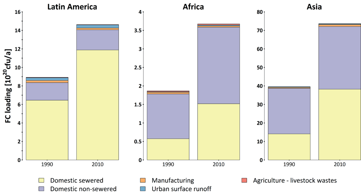
Figure 3.7: Faecal coliform bacteria loadings for Latin America, Africa and Asia for 1990 and 2010.
