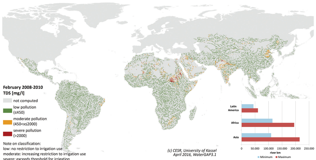
Figure 3.19: Estimated in-stream concentrations of total dissolved solids (TDS) for Latin America, Africa, and Asia for February 2008–2010. Bar charts show minimum and maximum monthly estimates of river stretches in the severe pollution class per continent in the 36-month period from 2008–2010 corresponding to data in Table 3.14.
