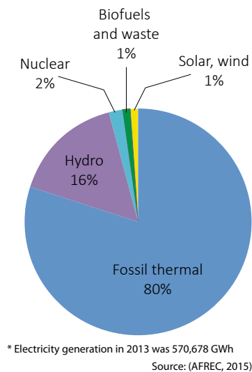
Figure 7: Fuel shares of electricity generation, 2013
