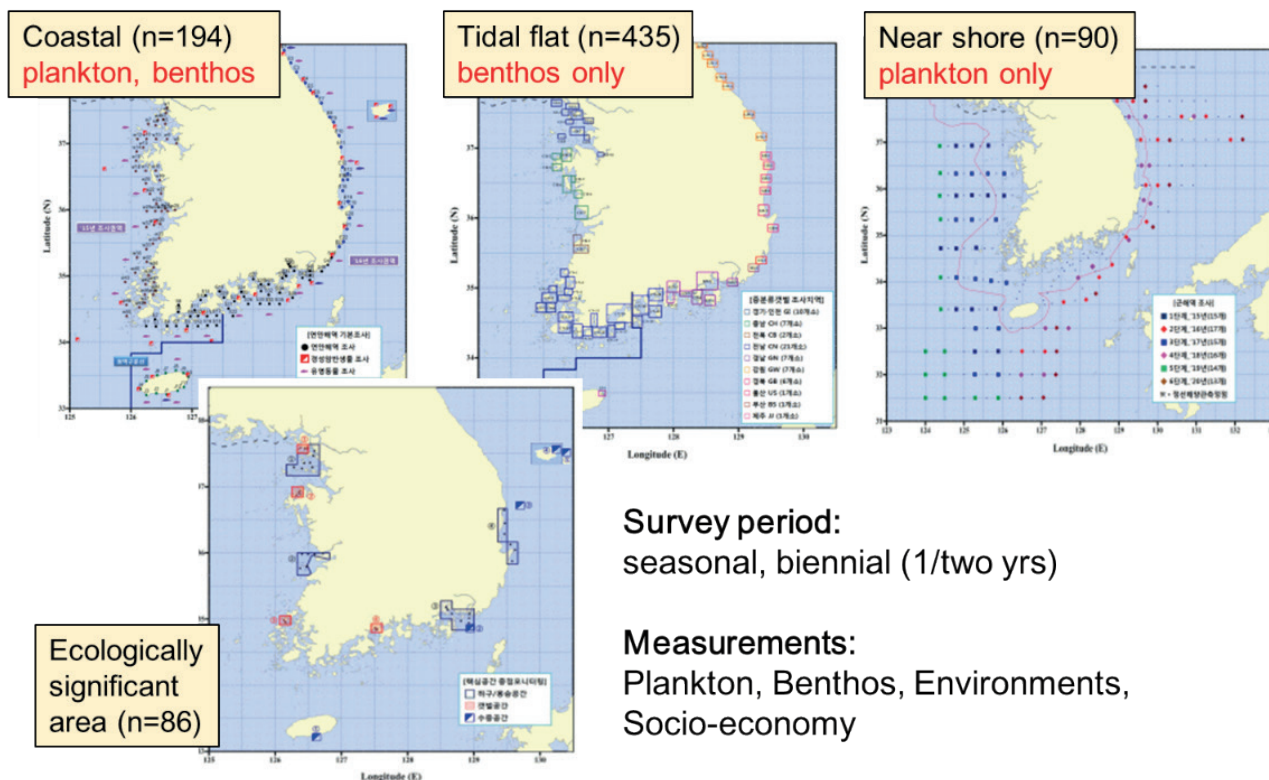
Fig. 3.1. Map showing the locations covered in the Integrated Marine Ecosystem Monitoring (I-MEM) program in Korea (“n” indicates the number of stations)
