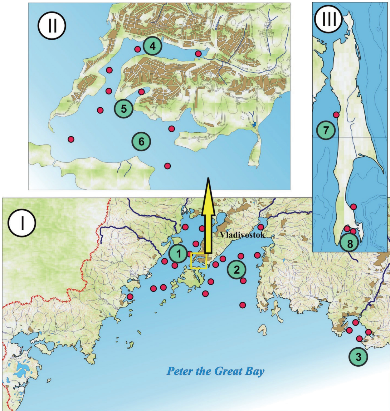
Fig. 4.1. Monitoring stations of State Observation Network in the Russian part of the NOWPAP region. 1 – Amursky Bay, 2 – Ussuriysky Bay, 3 – Nakhodka Bay, 4 – Golden Horn Bay, 5 – Diomid Bay, 6 – Bosphorus Vostochny Strait (Primorsky Krai); 7 – Tatar Strait, 8 – Aniva Bay (Sakhalin Island).
