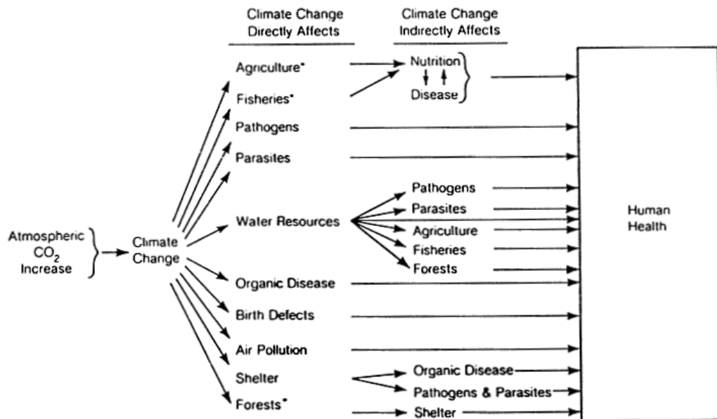
Figure 8. Pathways by which CO 2 -induced climate change may affect human health (from de Sylva, 1993).
