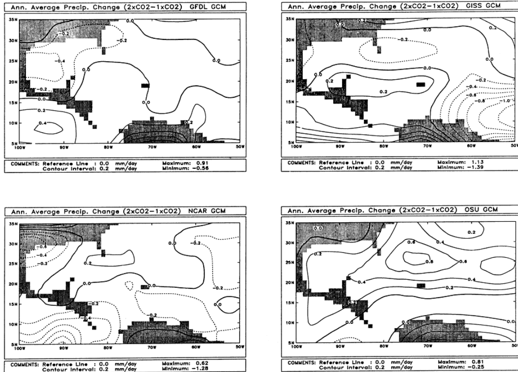
Figure 9b. Annual average precipitation change due to effective CO 2 doubling from GCMs of the Geophysical Fluid Dynamics Laboratory (GFDL), Goddard Institute for Space Studies (GISS), Oregon State University (OSU), and the National Center for Atmospheric Research (NCAR). Maps courtesy of Wigley and Santer (1993).
