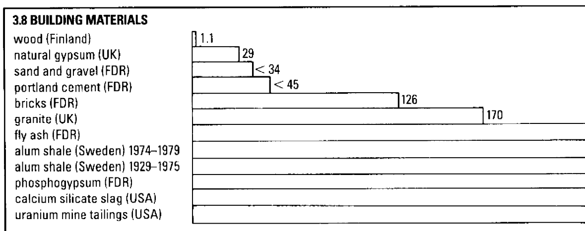
Mean activity concentrations in building materials as measured in various countries.
