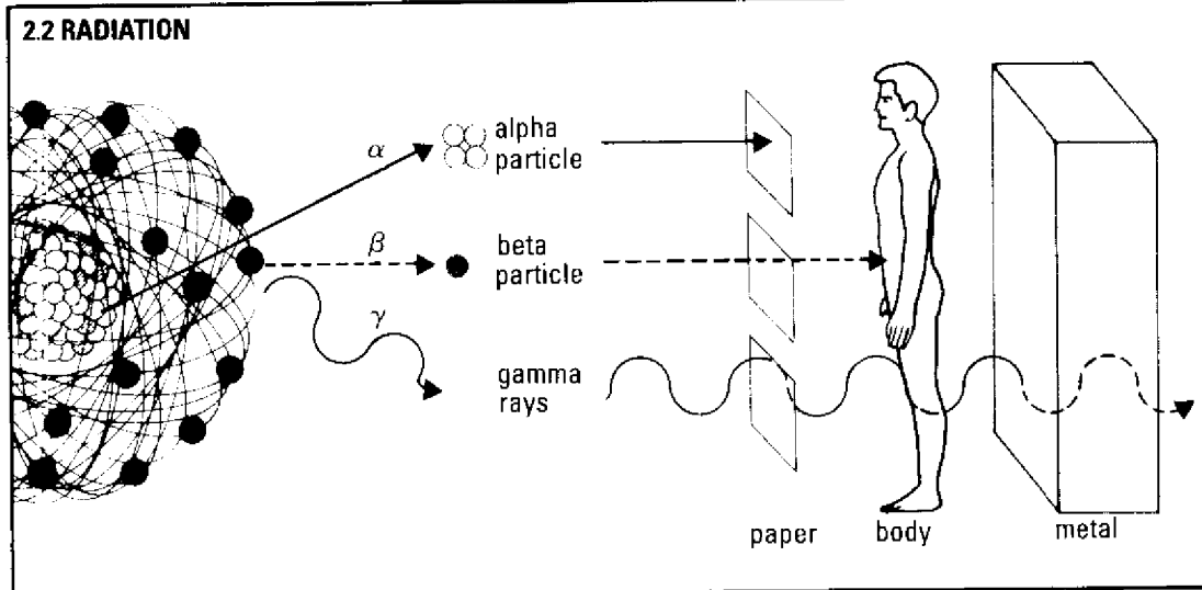
Three types of radiation and their penetrating power.
