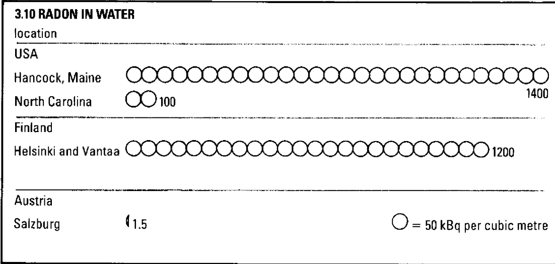
Average radon activity concentrations (kBq per cubic metre) in water sources.
