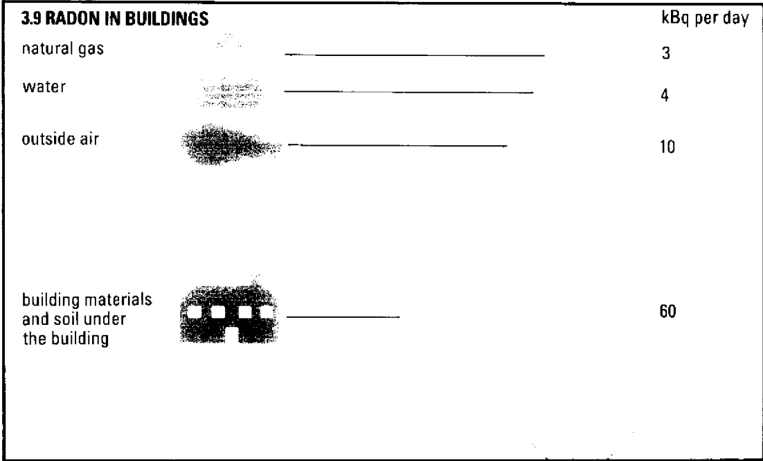
The relative contribution of different radon sources in a reference house.
