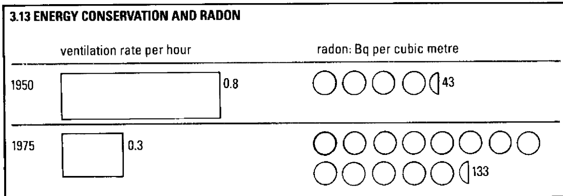
Decrease of ventilation rates and increase of average radon activity concentrations in Swedish apartment houses.
