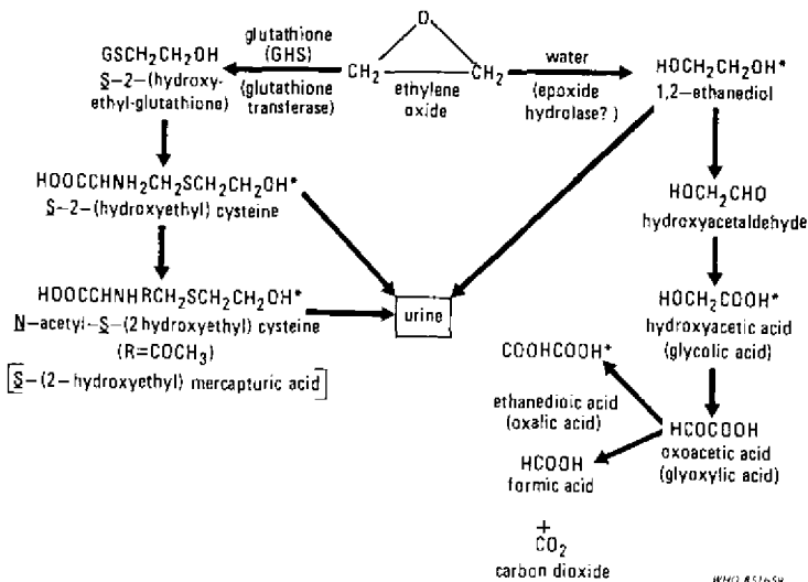
Fig. 1. Metabolism of ethylene oxide (*metabolites experimentally-identified by Gessner et al., 1961; McChesney et al., 1971; Jones & Wells, 1981). GSH = glutamylcysteinylglycine.
