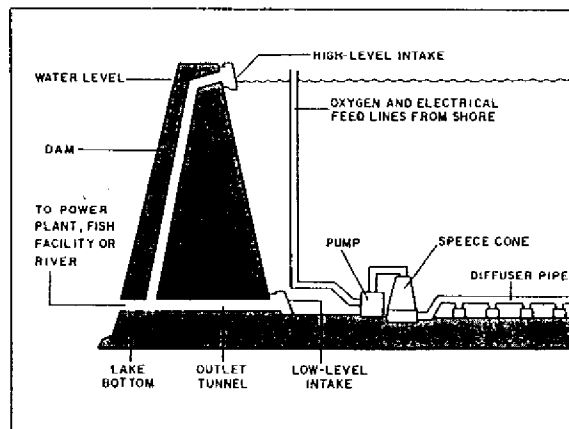
Fig. 11.5 The Speece cone for reservoir oxygenation with oxygen supersaturated water.
