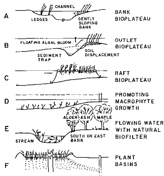
Fig. 10.2 Different methods of the use of aquatic and terrestrial vegetation for water quality protection in rivers. According to Klapper (1993).
