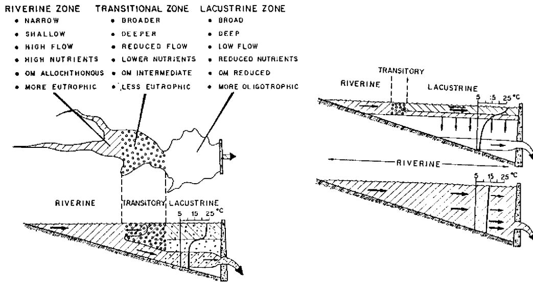
Fig. 4.11 Longitudinal zonation in a reservoir after Kimmel & Groeger (1984) and changes in the zone extension, flow and mixing pattern for reservoirs (reservoir conditions) with different ranges of R . Top - 10 < R < 100 days, center - R > 100 days, bottom - R < 10 days
