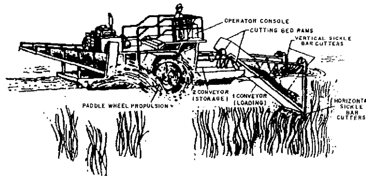
Fig. 11.11 One elaborate type of macrophyte harvester. Redrawn from Moore & Thornton (1988).
