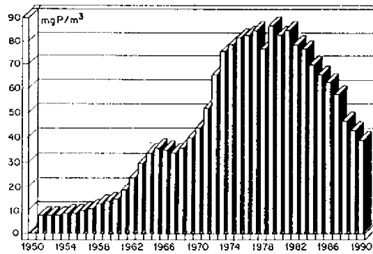
Fig. 6.7 Time sequence of phosphorus concentrations in Switzerland.
