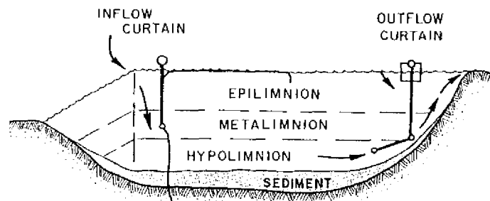
Fig. 11.10 The possible use of submersible curtains. The inflow curtain placed at the surface distributes the inflowing water to deeper strata. If the inflow curtain will be placed at the bottom, the inflowing water will be diverted to the reservoir surface. Similarly the outflow curtain may direct the flow to outlets from the top, bottom, but also middle layers of the reservoir.
