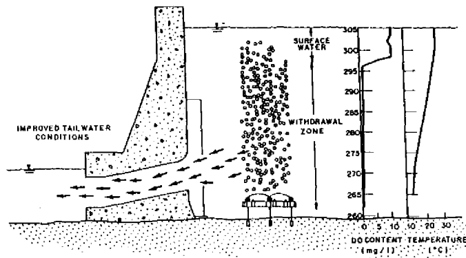
Fig. 12.2 Aeration near turbine intakes to improve downstream water quality. Redrawn from Mobley (unpublished).
