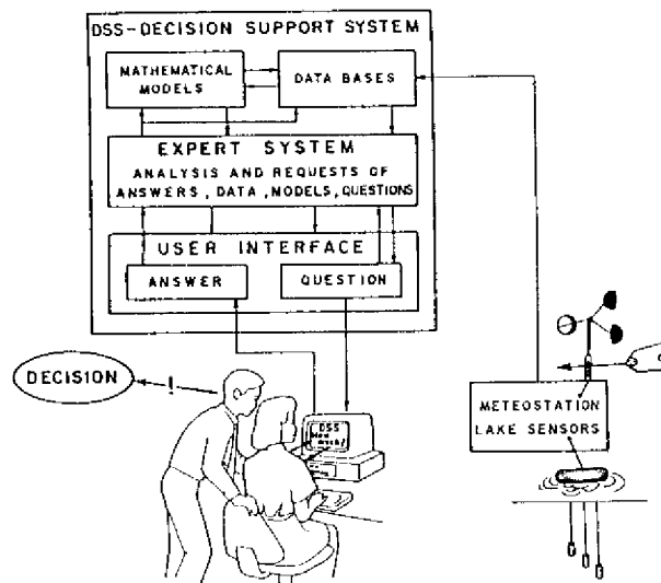
Fig. 14.4 The structure of a Decision Support System for water quality control.
