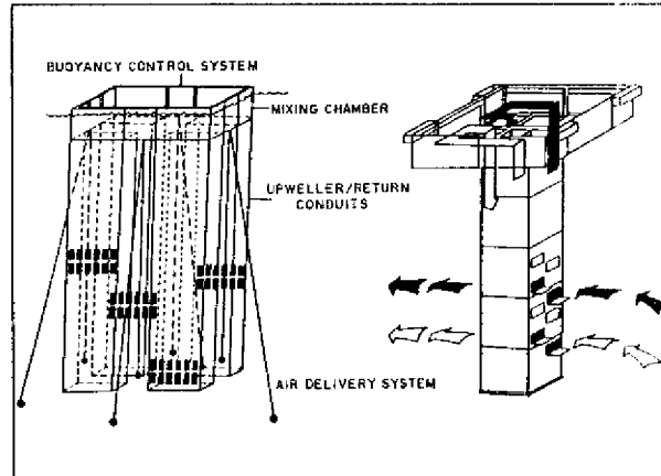
Fig. 11.4 Two possible types of layer aeration according to Kortman et al. (1988).
