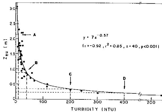
Fig. 4.7 Dependence of the depth of the epilimnion ( z_e ) on turbidity.
