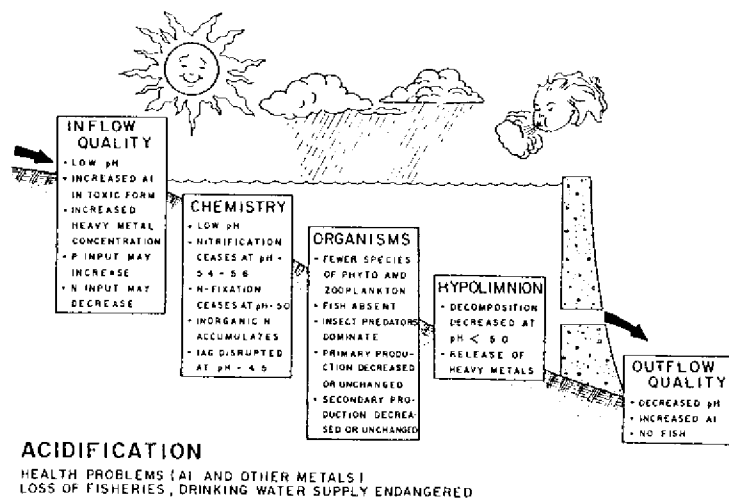
Fig. 6.8 Schematic representation of major consequences of acidification in a reservoir. Below economic impacts are listed
