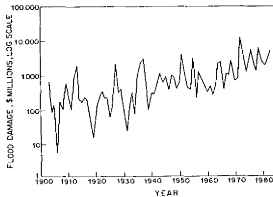
Fig. 6.4 Increasing flood damage. Note that the scale is logarithmic. Redrawn from Naiman et al. (1995).
