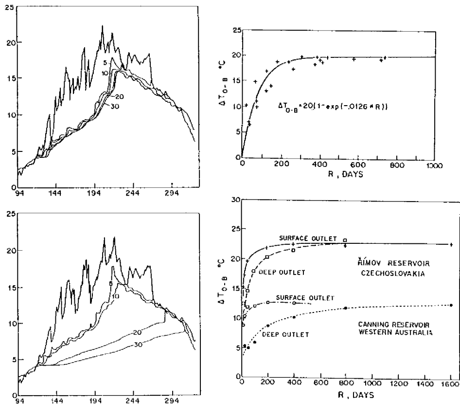
Fig. 4.9 Temperature stratification in reservoirs in dependence of the outlet location. Left - Upper panel - annual changes of temperature in a temperate reservoir with the theoretical retention time R = 12 days and with the bottom outlet. Lower panel - The same reservoir with the surface outlet (values calculated by the model DYRESM). Right - Upper panel: observed dependence of the degree of stratification in a number of Central European reservoirs on the theoretic retention time, R . Lower panel: The same dependence calculated with the model DYRESM for the temperate Římov and a subtropical Canning Reservoir, with localization of outlets in the depth as observed and at the surface (the latter representing a lake situation).
