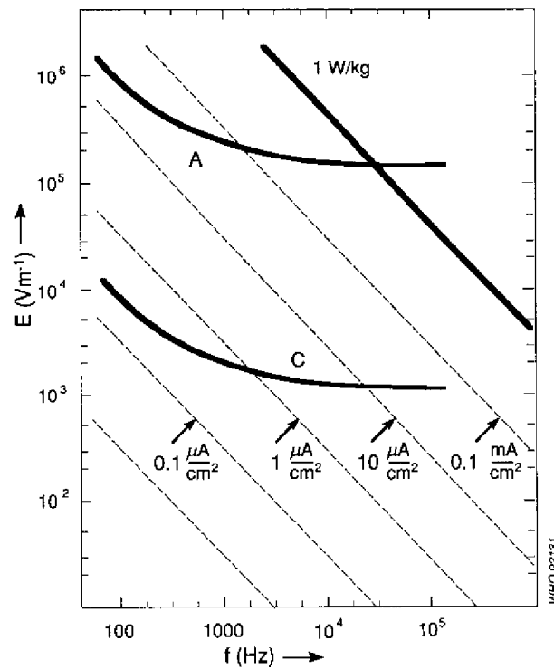
Fig. 23. Unperturbed electric field strength ( E in \text{V/m} ), as a function of frequency ( f in \text{Hz} ), that induces the indicated current density ( \mu\text{A}/\text{cm}^2 or \text{mA}/\text{cm}^2 ) in the head or cardiac region of a person exposed with the long axis of the body parallel to the orientation of the E -field. From: Bernhardt (1985). In other parts of the body (e.g., neck, trunk, ankles), the current densities are larger at the same external field strengths.
