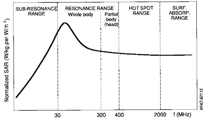
Fig. 7. Variation of normalized SAR with frequency and related absorption characteristics in living organisms.
