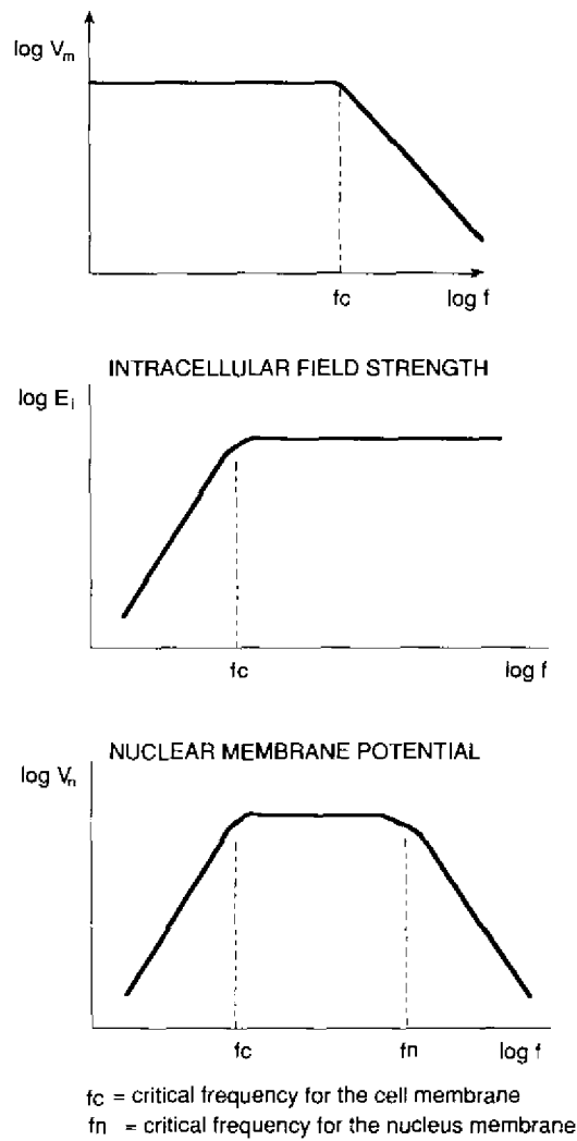
Fig.11. Induced membrane potentials and electric fields in various cell compartments. From: Schwan (1985).
