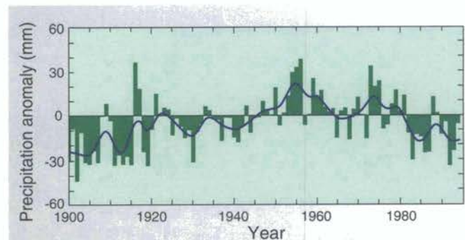
Figure 11: Changes in land-surface precipitation averaged over regions between 55°S and 85°N. Annual precipitation departures from the 1961-90 period are depicted by the hollow bars. The continuous curve is a smoothing of the same data.
