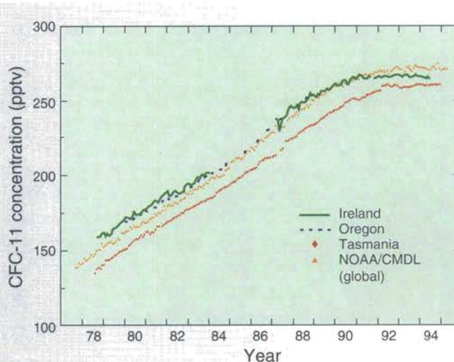
Figure 4: Global CFC-11 concentrations (pptv) for 1978 to 1994. As one of the ozone-depleting gases, the emissions of CFC-11 are controlled under the Montreal Protocol and its Adjustments and Amendments. Observations at some individual measurement sites are also shown.
