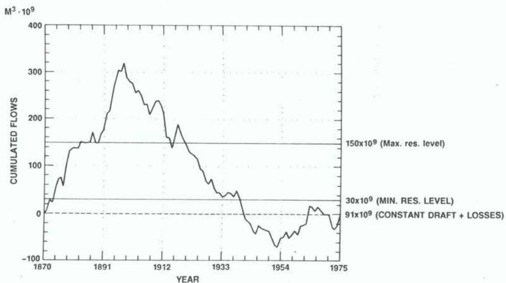
Figure 7. Cumulated flow of the Nile to Lake Nasser at Aswan, Egypt, in billions of cubic metres. Reservoir extremes and losses are also indicated.
