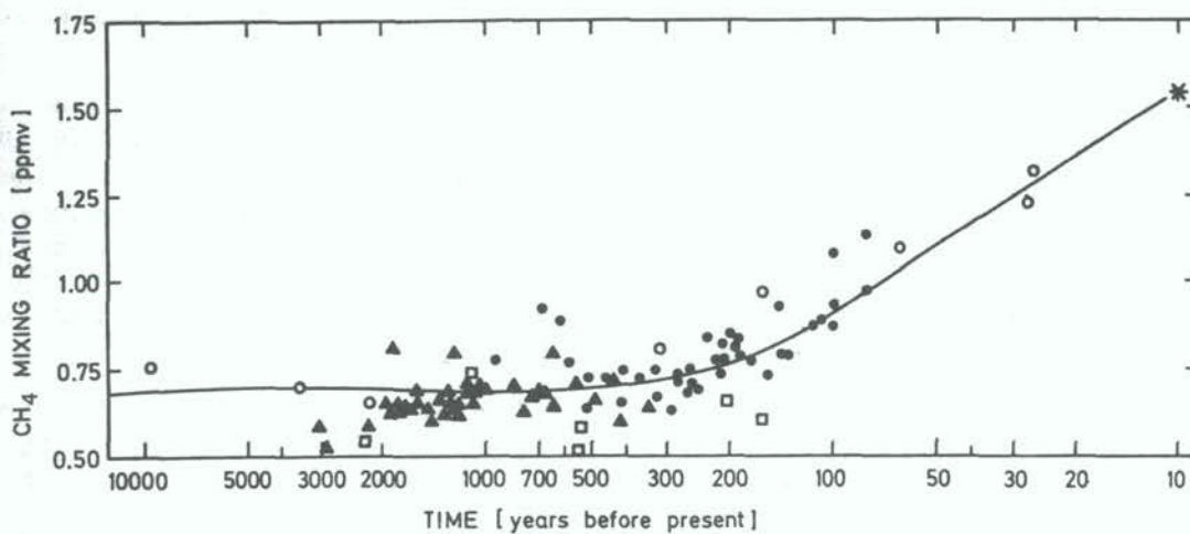
Figure 2. CH 4 mixing ratios measured in air trapped in ice cores as a function of time (Bolle et al., 1986).
