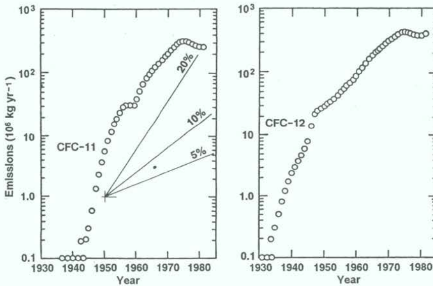
Figure 1b. Historical emissions of CFC-11 and CFC-12 (Bolte et al., 1986).
