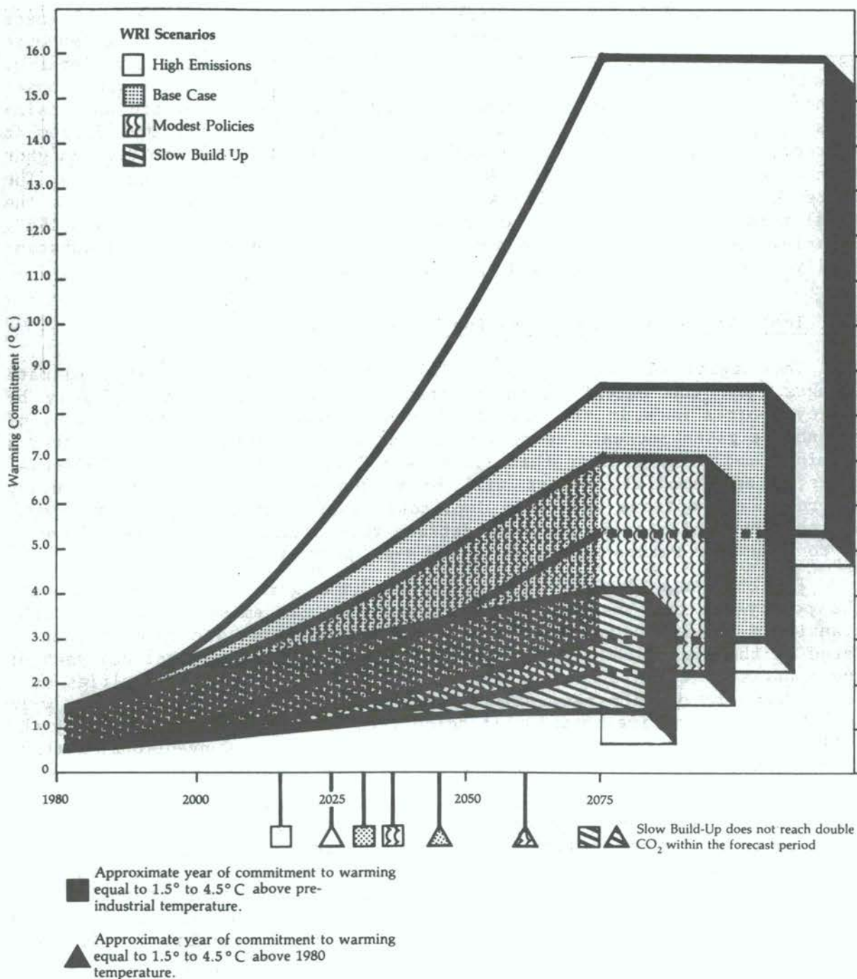
Figure 5. Commitment to future warming in the WRI Scenarios.
