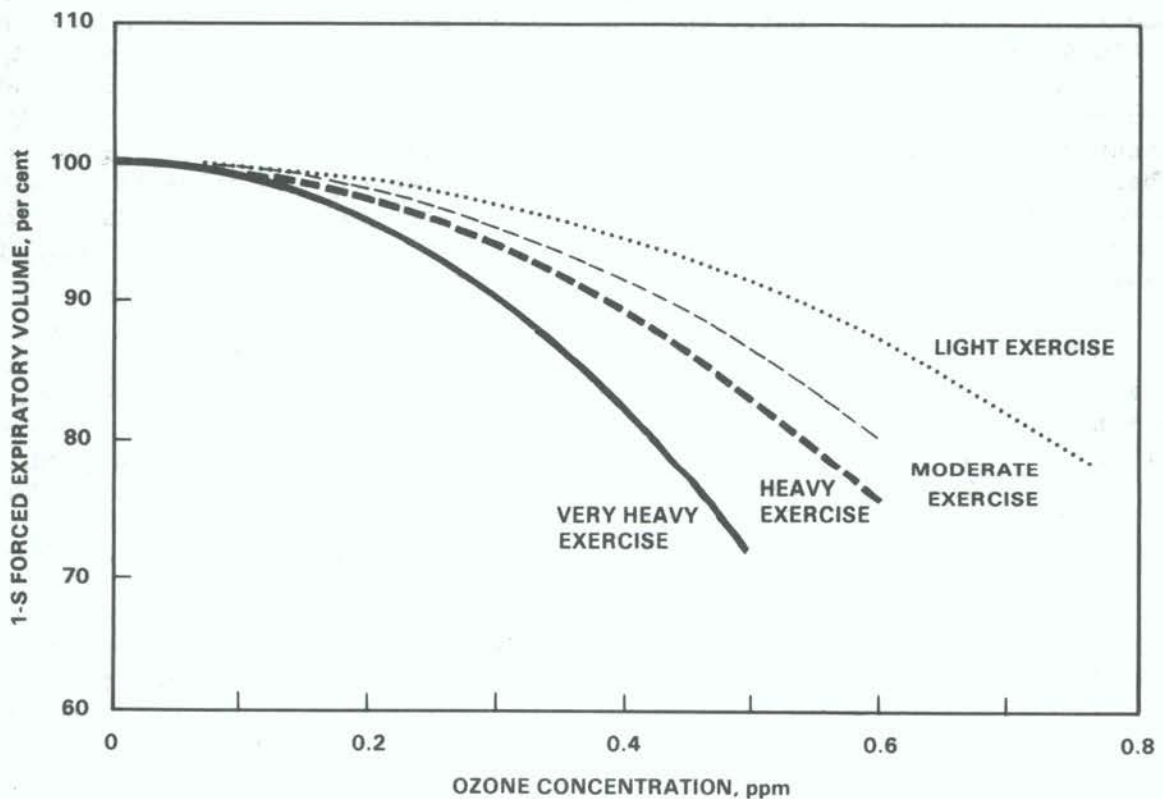
Figure 1. Group mean decrements in a 1-s forced expiratory volume during 2-h ozone exposures with different levels of intermittent exercise. The concentration-response curves shown are typical of other measures of pulmonary function decrements due to ozone (adapted from U.S. EPA, 1986).
