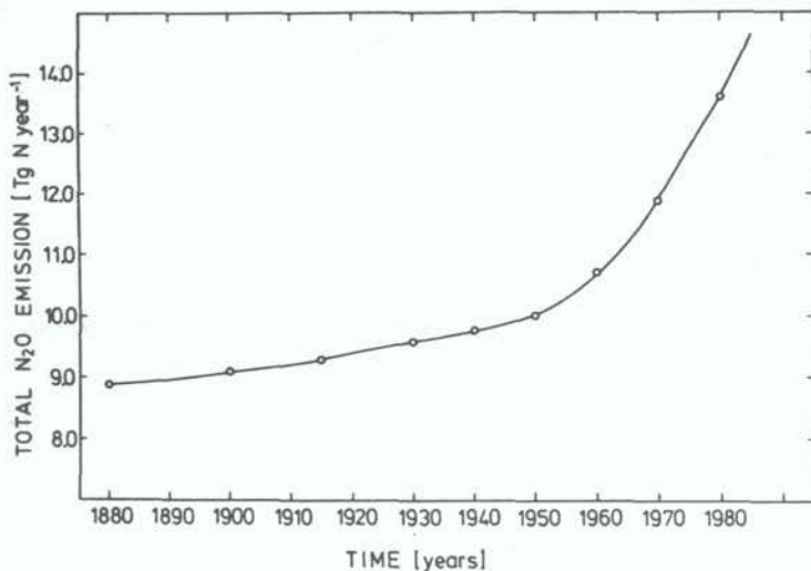
Figure 3. Trend of estimated total N 2 O emission rates between 1880 and 1980 (Bolle et al., 1986).
