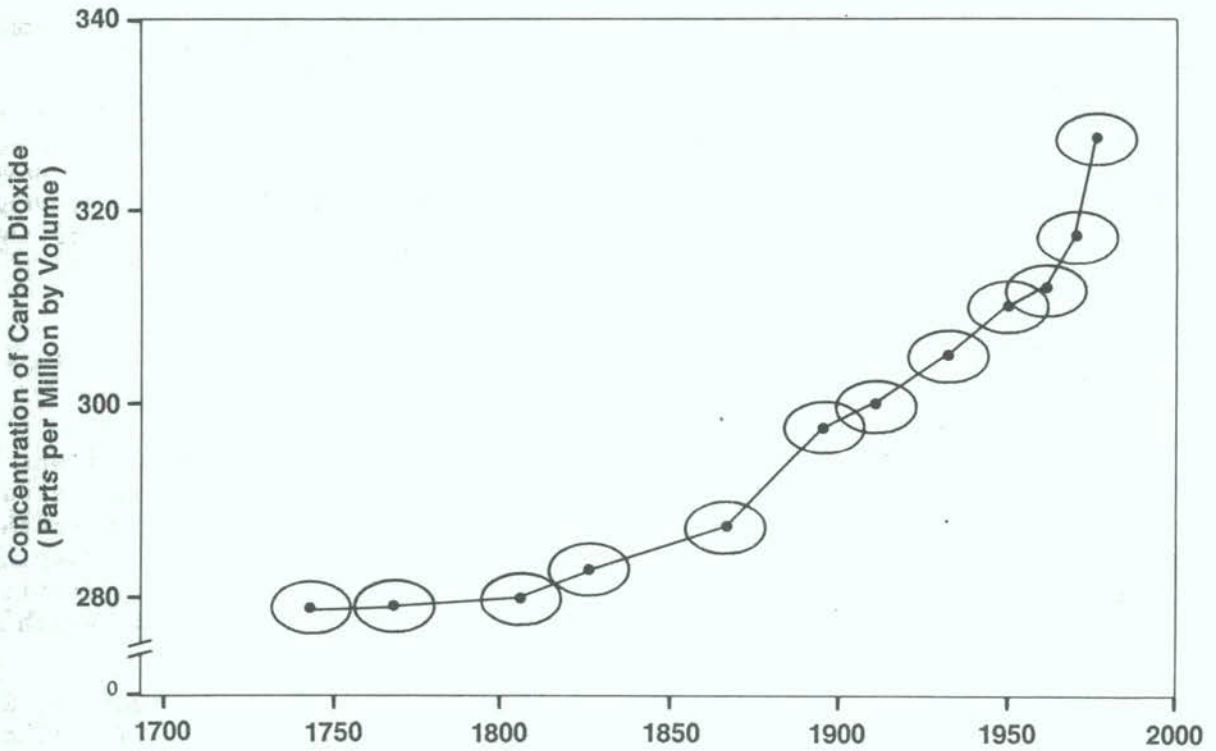
Figure 1a. CO 2 concentrations measured in glacier ice formed during the last 200 years (Neftel et al., 1985).
