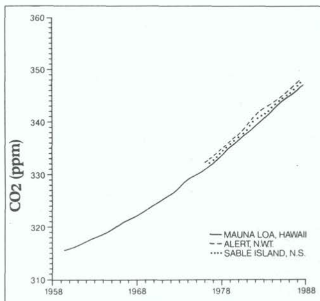
Figure 1. Atmospheric CO 2 concentrations measured at Mauna Loa, Hawaii, Alert, Northwest Territories and Sable Island, Nova Scotia.
