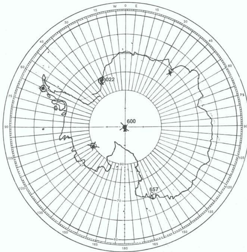
Figure 5. WMO Antarctic Ozone Observing Network.
