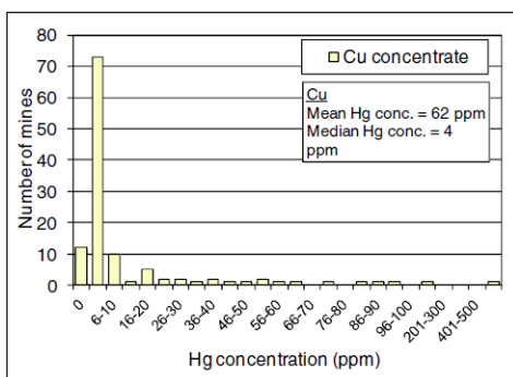
Figure 5-5 Distribution of mercury concentrations in copper concentrates globally (reprinted with permission from Hylander and Herbert, 2008. Copyright 2008 American Chemical Society).
