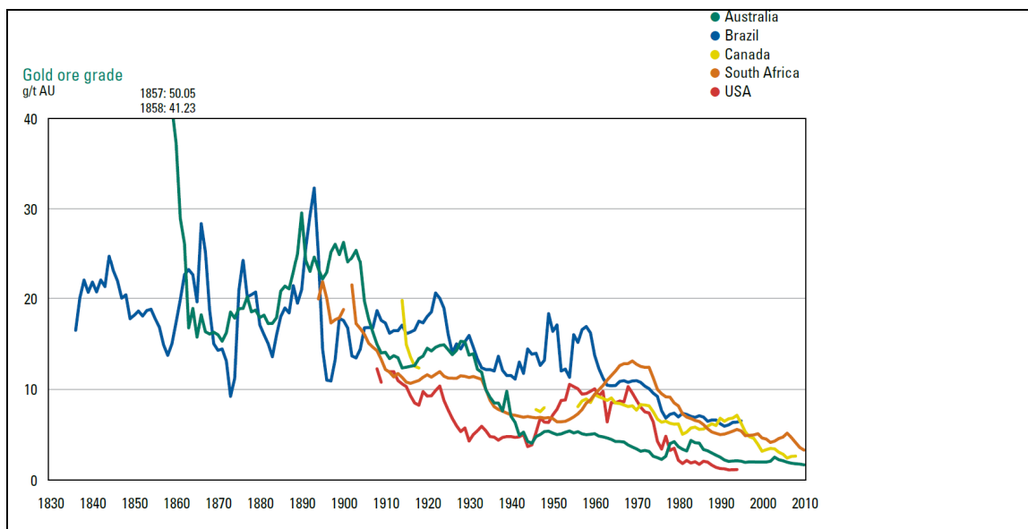
Figure 5-7 The development in gold concentration in gold ore from various countries (UNEP, 2011c citing Giurco et al, 2010).
