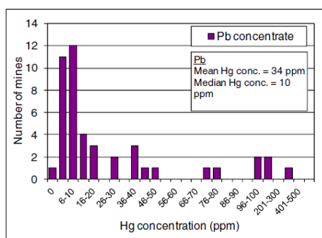
Figure 5-6 Distribution of mercury concentrations in lead concentrates globally (reprinted with permission from Hylander and Herbert, 2008. Copyright 2008 American Chemical Society).
