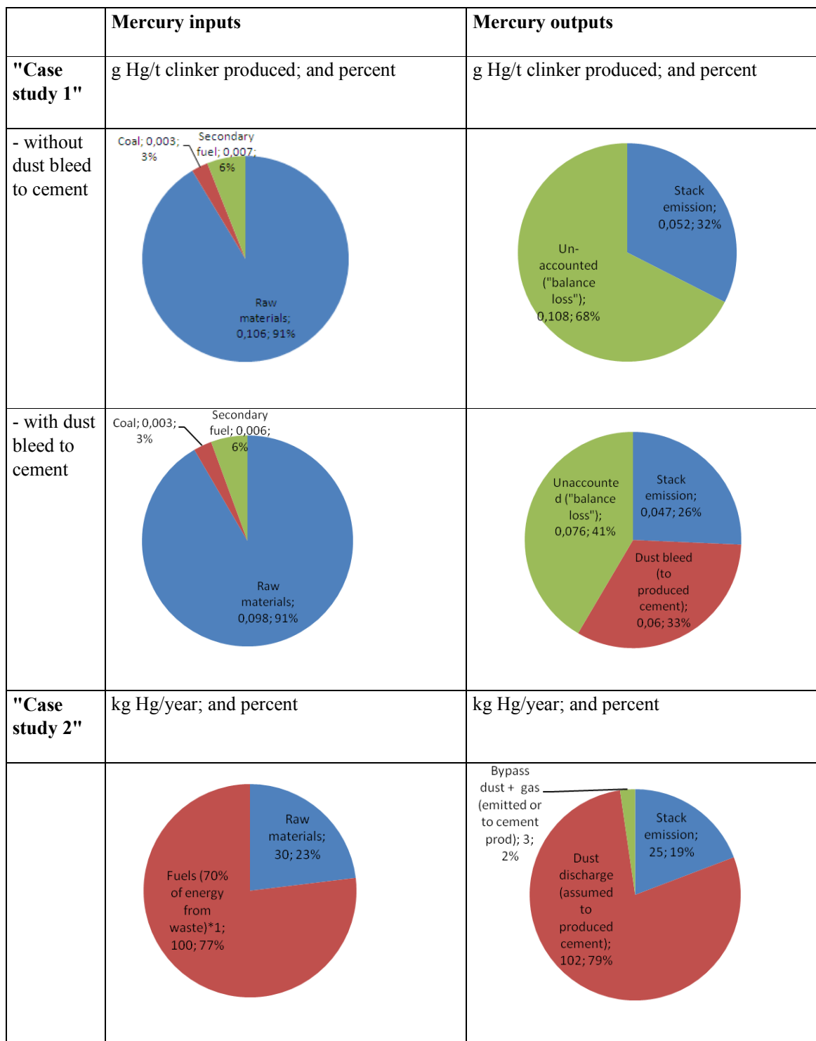
Figure 5-8 Mercury inputs and output distributions from two cement production facilities (data from CEMBUREAU, 2010. Note*1: Based on other data given in the reference, fossil fuel Hg contributions are assumed minimal).
