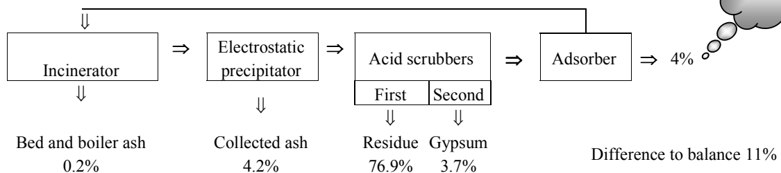
Figure 5-9 Balance of mercury in a sewage sludge incineration plant of Hamburg, Germany (Saenger et al. , 1999b)
