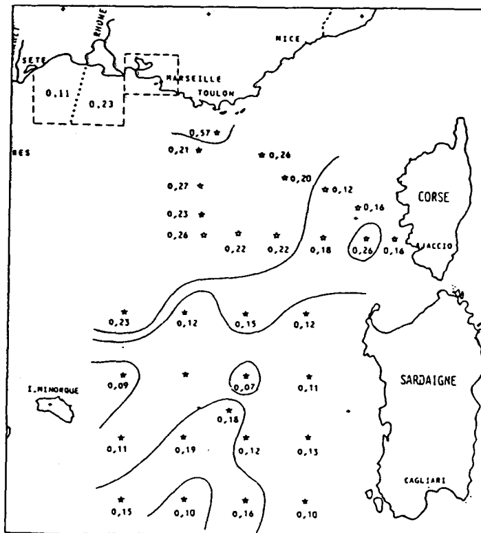
Figure 6. Mercury levels in sediments (mg/kg DM) in the Western Mediterranean (Arnoux et al.).
