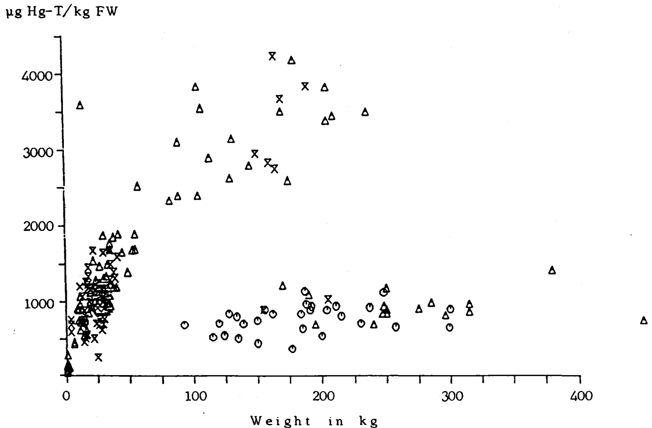
Figure 11. Total mercury concentrations in Thunnus thynnus from the Strait of Gibraltar (⊙), Spanish coast (x), the French coast (X) and Tyrrhenian Sea (Δ). The term FW denotes fresh weight. (Data from Renzoni et al. 1979; Establier, 1972, 1973, Ballister et al. , 1978; and Thibaud and Gouygou, 1979)
