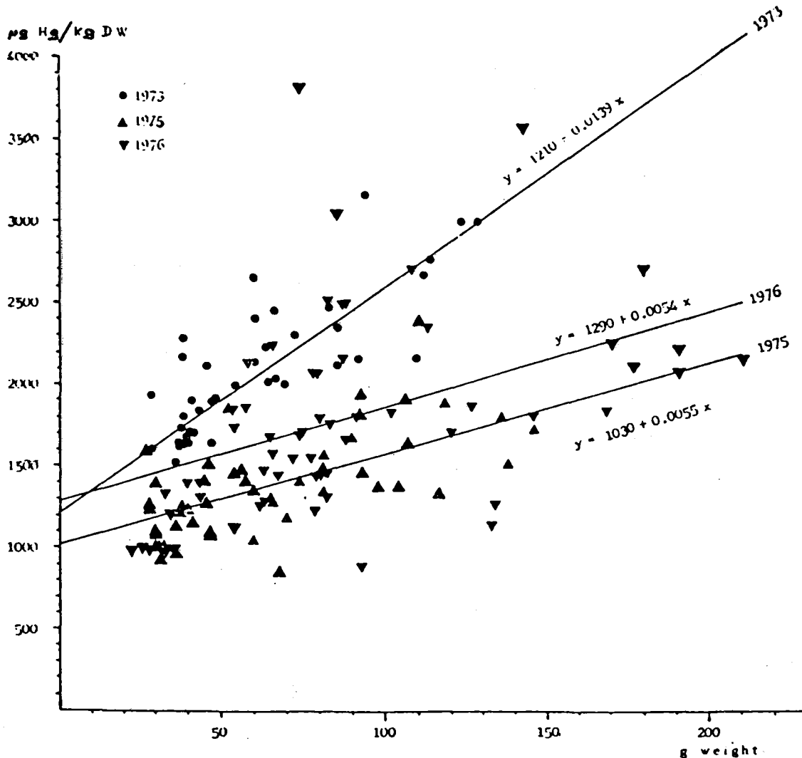
Figure 33. Mercury concentration versus weight in Scorpaena porcus from the banks of Vada before (1973) and after (1975 and 1976) waste treatment began in the Solvay chlor-alkali plant (Renzonei, 1977).
