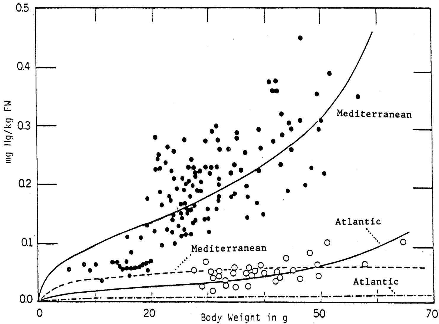
Figure 53. Total mercury concentrations in Sardina pilchardus from the Strait of Gibraltar (O) and Tyrrhenian Sea (●). The continuous lines show total Hg concentrations calculated by a model; intermittent lines show inorganic Hg concentration calculated by a model (Bernhard, 1985).
