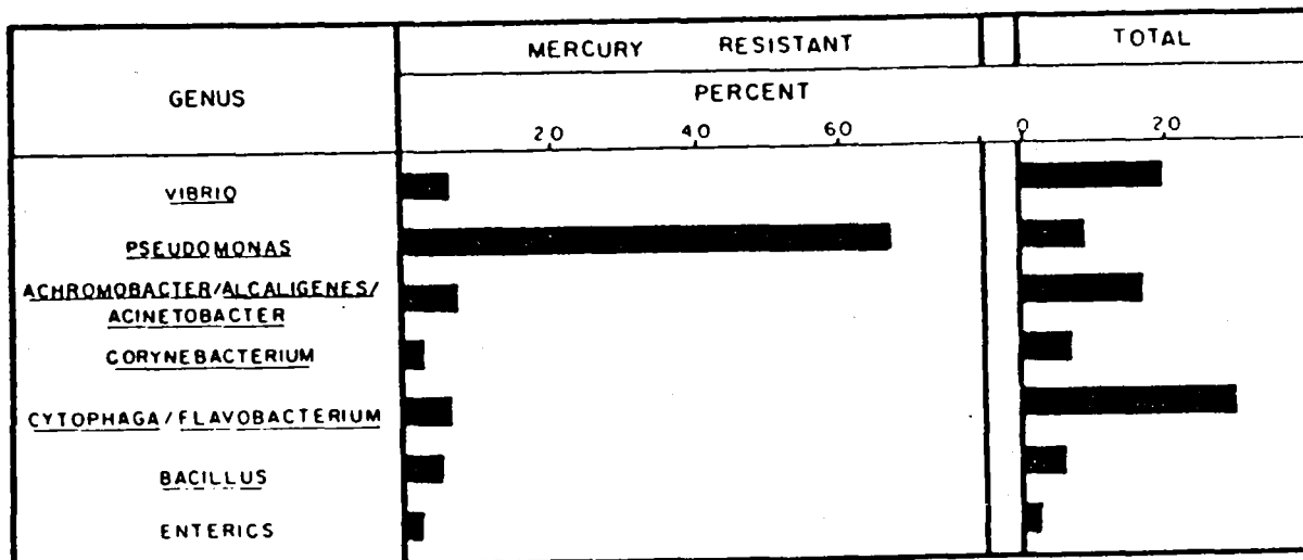
Figure 50. Average distribution of genera in total and HgCl 2 -resistant populations (Colwell et al. 1976)
