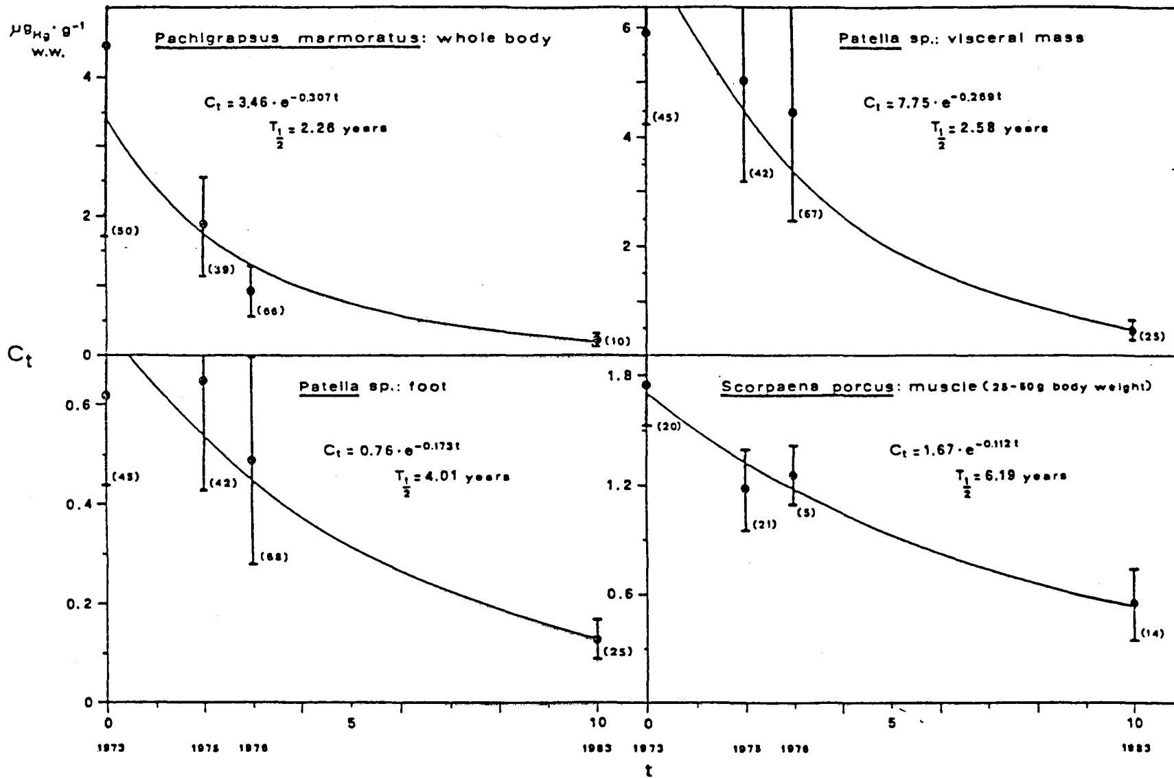
Figure 35. Recovery trends estimated from different "bioindicators" in Solvay outfall area (Bacci et al. 1986). C_t represents the Hg concentration in the indicator organisms according to a one compartment model, and T_{1/2} biological half-time of mercury in organisms.
