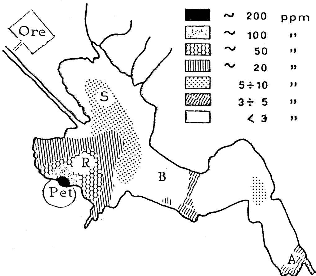
Figure 36. Mercury concentration in the surficial sediments of the S. Gilla Lagoon (Cagliari). A: entrance from the Gulf of Cagliari; Pet: petrochemical industry; Ore: ore processing industry; B, S, R: different zones in the lagoon (Porcu and Masala, 1983, modified).
