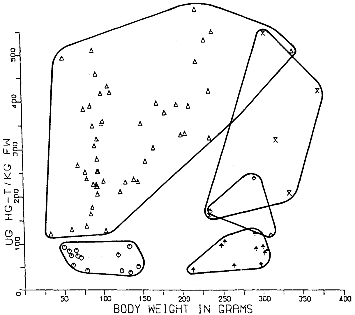
Figure 14. Total mercury concentrations in Scomber scomber and S. japonicus from the Strait of Gibraltar (O), Tyrrhenian Sea (Δ), Ostend (X) and Schevingen (↑). The term FW denotes fresh weight. (Data from Stoepler et al. 1979).
