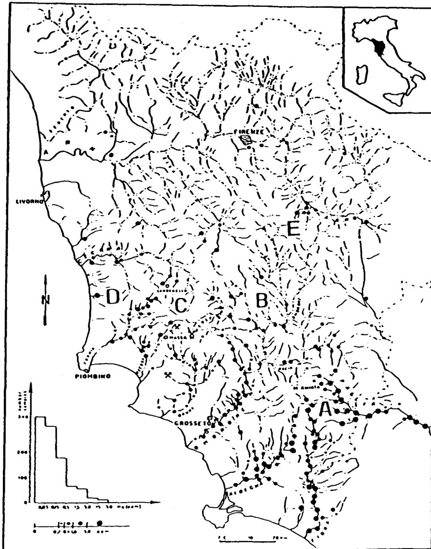
Figure 23. Distribution of mercury in river sediments around the mercury anomaly of Mt. Amiata (Tuscany) (Dall'Aglio, 1974).
