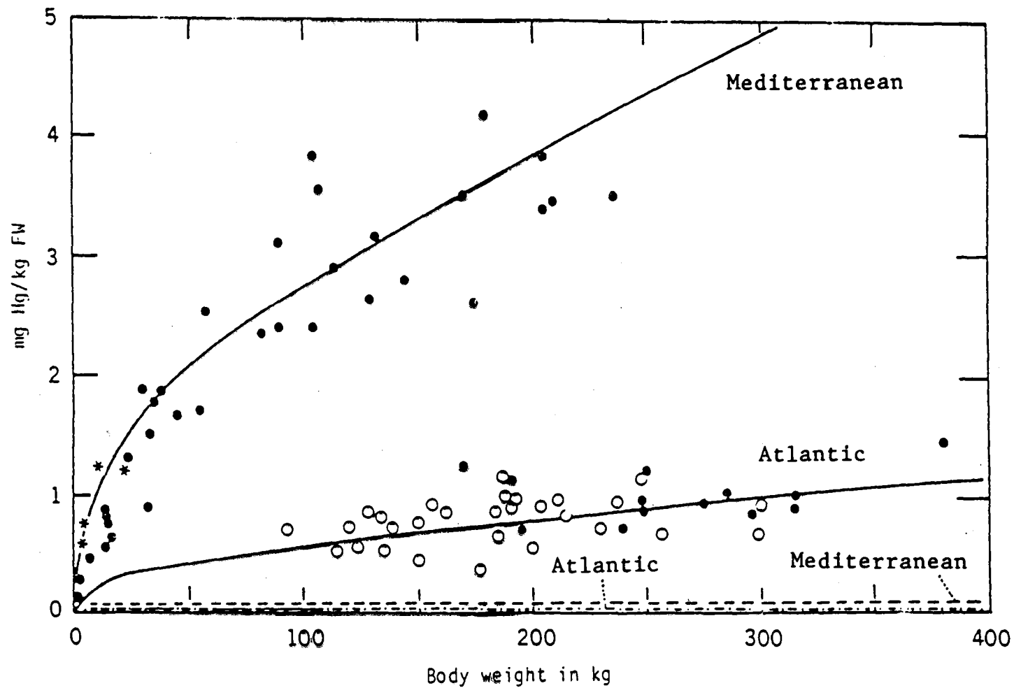
Figure 52. Total mercury concentrations in Thunnus thynnus from the Strait of Gibraltar (O), Tyrrhenian Sea (●) and Spanish coast (*). The continuous lines show total Hg concentrations calculated by a model; intermittent lines show inorganic Hg concentration calculated by a model (Bernhard, 1985).
