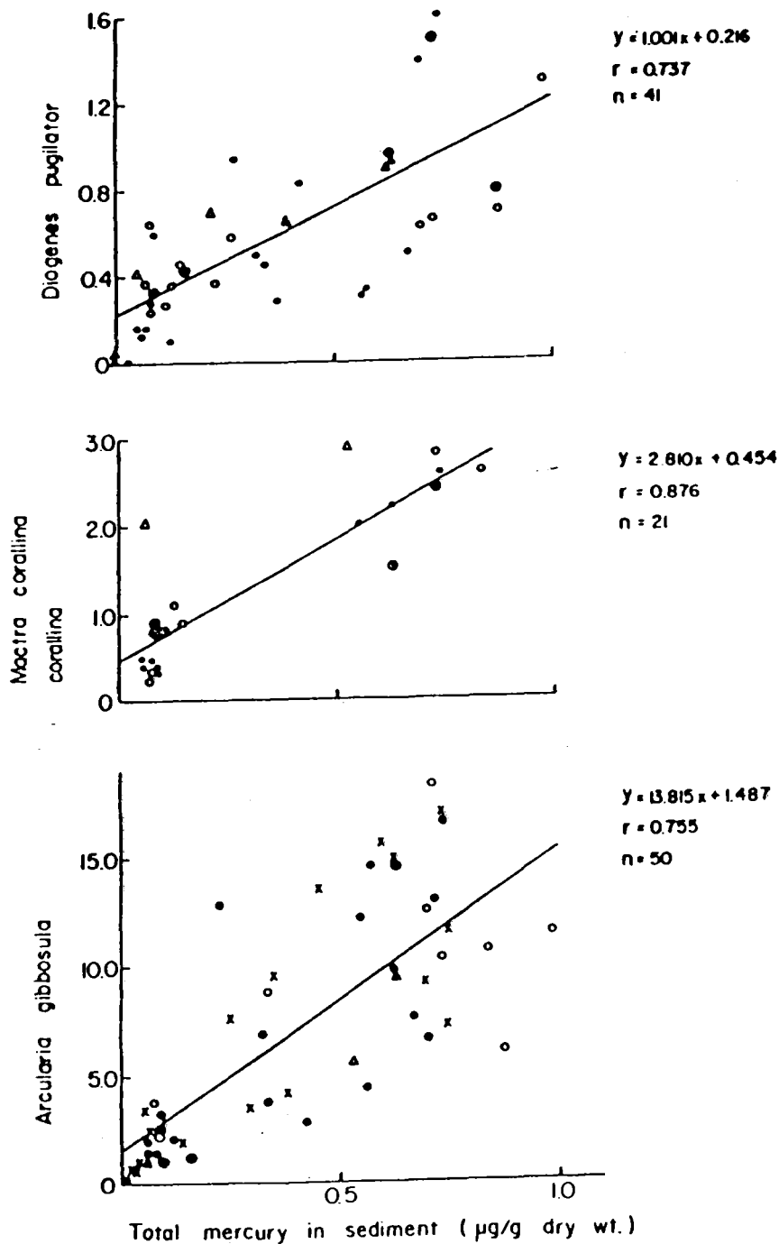
Figure 40. Relationship between mercury concentrations in three benthic organisms and surficial sediments from the coast of Israel (Hornung, 1986).
