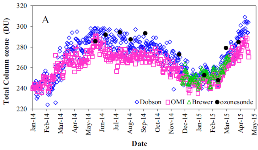
Figure 2.2. Seasonal daily variation of various quantities during the period 01/01/2014 to 31/05/2015 at the study site (13° 39' 58.57" N, 100° 36' 21.44" E): A) Daily column ozone obtained from Dobson spectrophotometer, Brewer spectrophotometer, ozonesonde and OMI/AURA satellite.
