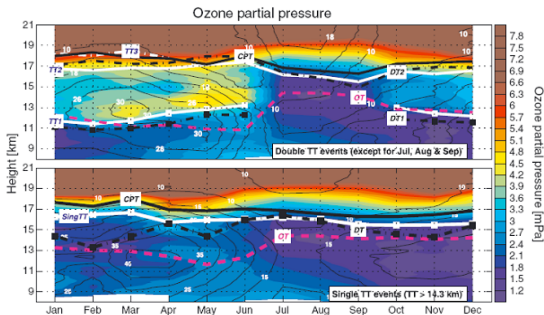
Figure 3: Time-height cross section of ozone partial pressure (mPa) and wind speed contours (ms -1 ) from 8 to 21 km height for (top) multiple and (bottom) single thermal tropopause events. The vertical coordinate is tropopause based. The different tropopause types are shown labeled with their corresponding acronym. TT1, TT2 and TT3 are the first, second and third thermal tropopauses, respectively; DT1 and DT2 are the first and second dynamical tropopause, respectively; OT is the ozone tropopause, and CPT is the Cold-Point tropopause.(Franco et al., 2013)
