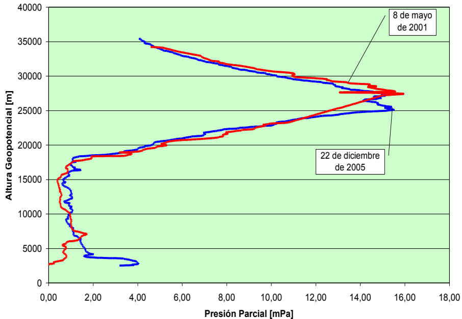
Illustration 1. Ozonesonde profiles of Bogota station which reached the higher height: one made on 22/12/2005 with 35424 m (blue) and second made on 08/05/2001 with 34247 m (red). (Source: IDEAM).
