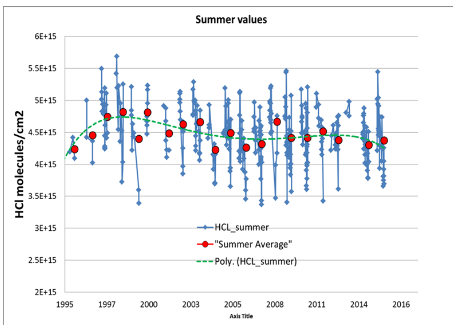
Figure 1. HCl column values from Harestua 1995 to 2015
