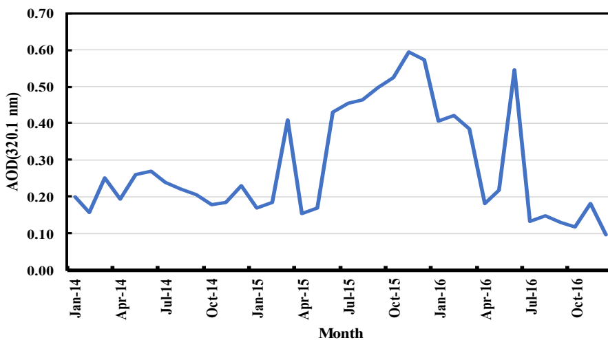
Fig. (4): Monthly variation of Aerosol optical Depth (AOD at 320.1 nm
