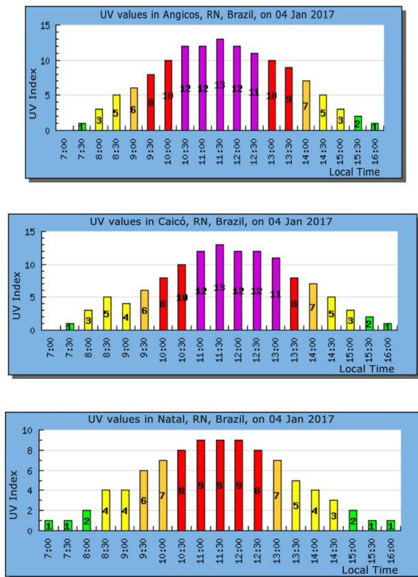
Figure 4: The UV index for Angicos, Caicó and Natal for 01/04/2017.
