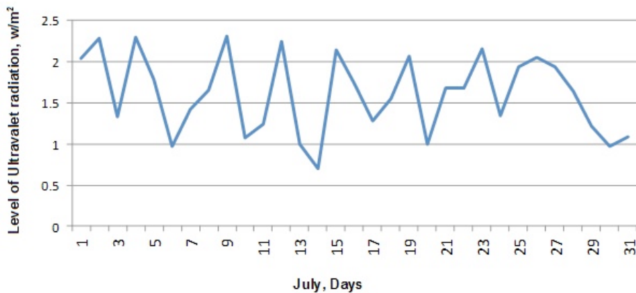
Figure 3. Daily average level of UV radiation
