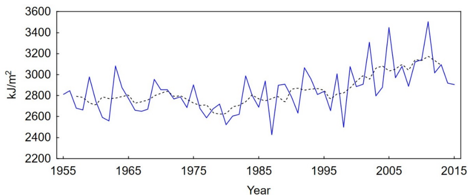
Figure 1. UVB annual doses (blue line) with 5-year moving average (black dotted line) from 1955 to 2015 at Tõravere, Estonia. Solely calculations have been used for the period 1955–2003 and measurements combined with calculations (in case of no available measurements) for the period 2004–2015.
