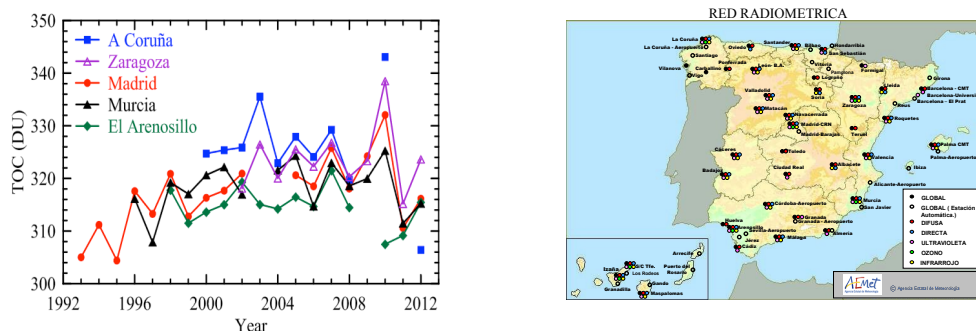
Figure 1: Temporal Evolution of yearly TOC values at five Spanish Stations (left),(Mateos et al., 2015) and the AEMET UV broadband network.
