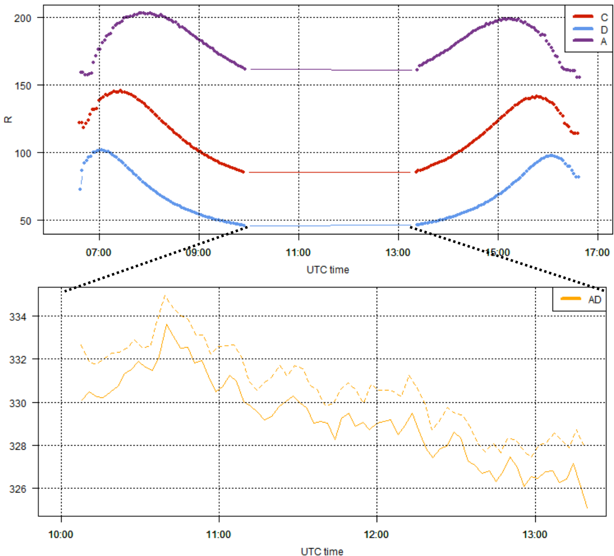
Figure 3: upper panel: Dobson (D051) Umkehr measurements for the 3 wavelength pairs A,C and D; lower panel: direct sun ozone column measurements by to independent Dobson instruments (D062 and D051) at Arosa.
