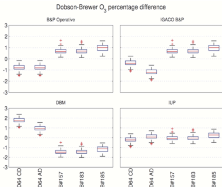
Figure 2: Percentage ratio between Dobson (Dobson 64 AD and CD pairs) and Brewer (B#157,B#183 and B#185) when apply the same Langley calibration and different cross section analysed (Bass & Paur, operative (B&P operative) and the temperature quadratic fit (IGACO B&P), the Daumont, Brion & Malicet (DBM) and the Serdyuchenko 2013 developed by the University of Bremen for the HARMONICS project. (Redondas et al., 2014)
