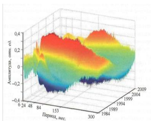
Figure 22. The results of wavelet transform of aerosol optical depth [12]
