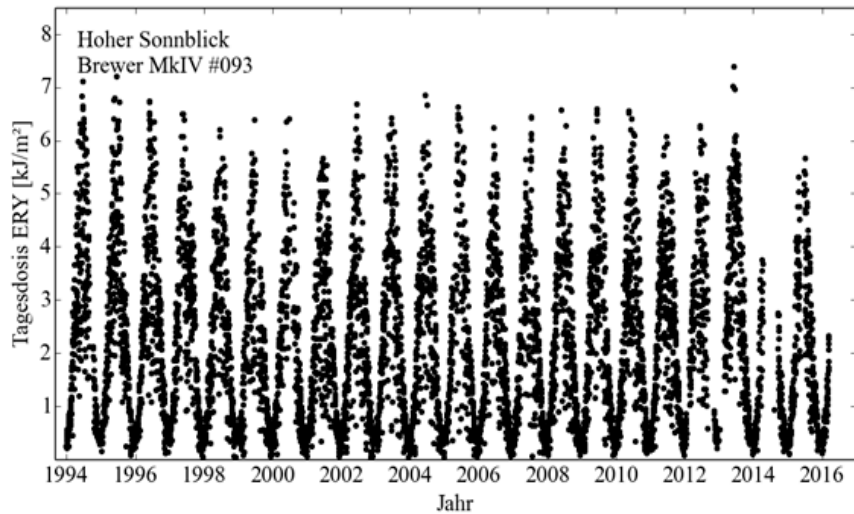
Fig. 5: Daily erythemal dose from Brewer MkIV #093 spectrophotometer between 1994 and 2016
