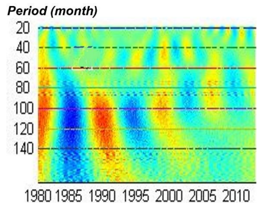
Figure 18. The results of wavelet analysis of time series of \text{H}_2\text{O} (1980-2015).
