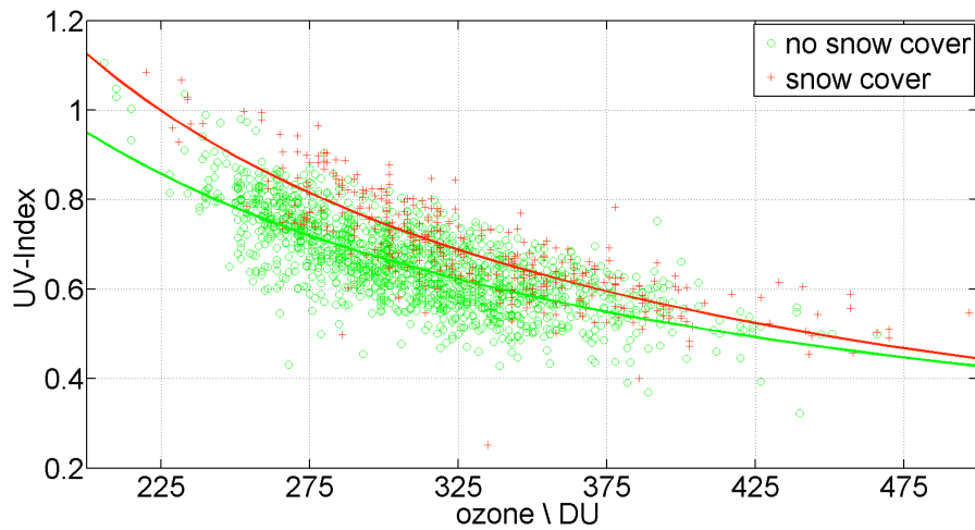
Fig. 3: Relation between UV-Index and ozone column
