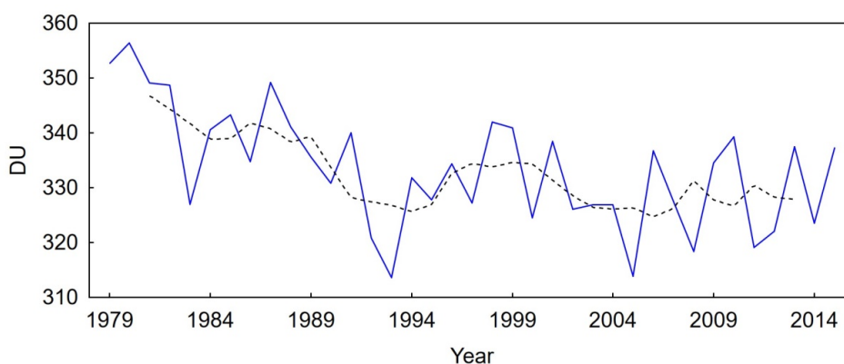
Figure 2. Annual average column ozone (blue line) in Estonia from 1979 to 2015 with 5-year moving average (black dotted line).
