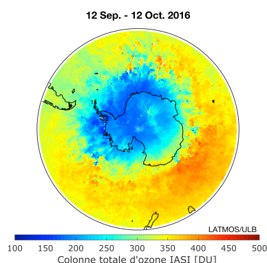
Figure 1. Total ozone column measured by IASI over the period 12/09–12/10/2016 over Antarctica
