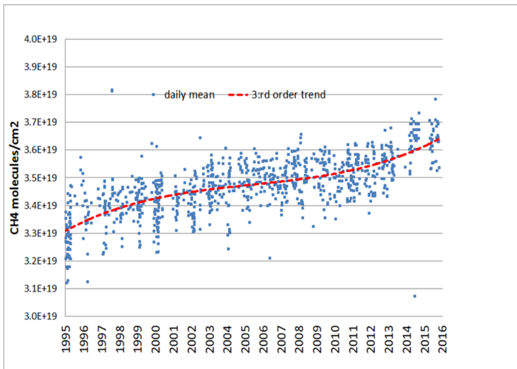
Figure 2. Column methane shows a positive trend at Harestua
