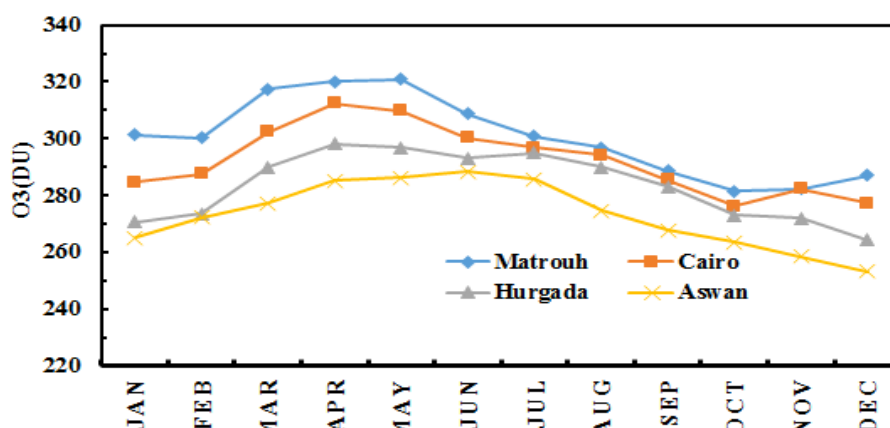
Fig.(2): Annual variation of ozone at Egyptian ozone observatories from 2010 to 2016
