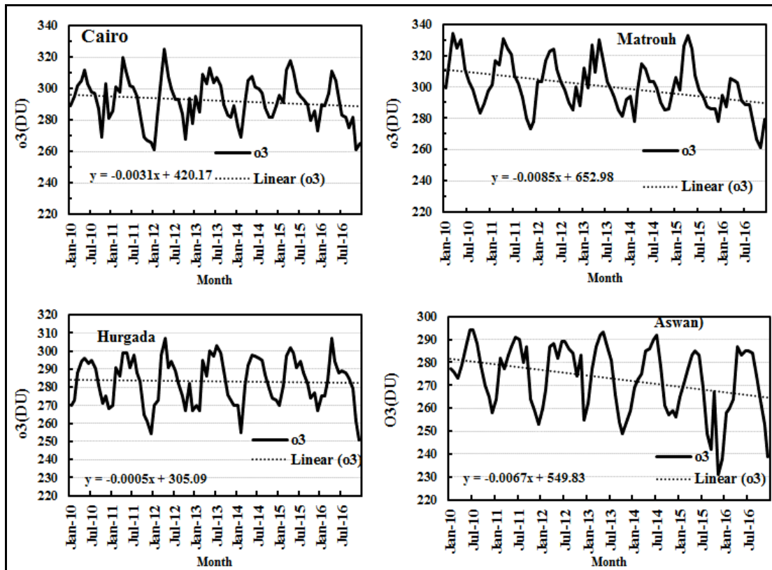
Fig.(3): Monthly variation and trend of ozone at Egyptian ozone stations 11.2 Variation of total column of sulfur dioxide (SO 2 ) and Aerosol Optical Depth (AOD) at northwest of Egypt
