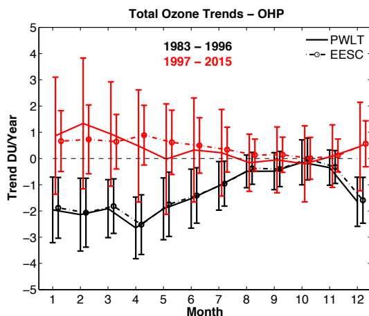
Figure 2. Total ozone trends during two periods (1983-1996 and 1997-2015) and for two methods: PWLT or EESC.
