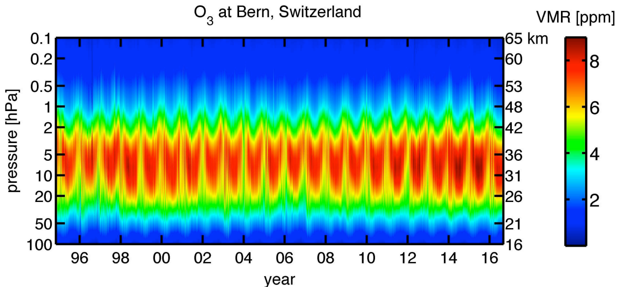
Figure 4: Ozone volume mixing ratio as function of time and pressure level above Bern. Observations were obtained by a 142-GHz microwave radiometer (IAP, Bern). Tick marks are on January, 1st of each year.
