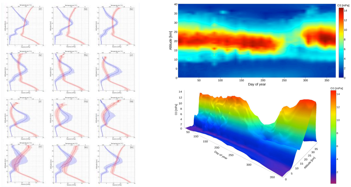
Vertical profile climatology from 28-year (November 1988–August 2016) ozone soundings at Marambio Station, Antarctic Peninsula (Sanchez et al, 2016). Left: monthly average ozone profile. Right: daily average ozone profile.
