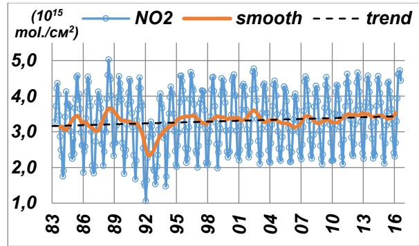
Figure 16. Time series of monthly average values of total \text{NO}_2 , obtained from average daily data on \text{NO}_2 , its smoothed curve (smooth) and linear trend (trend)
