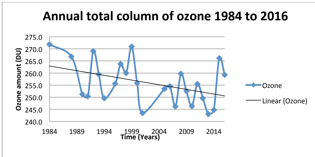
Fig: 1. Annual total column of ozone in Nairobi, Kenya
