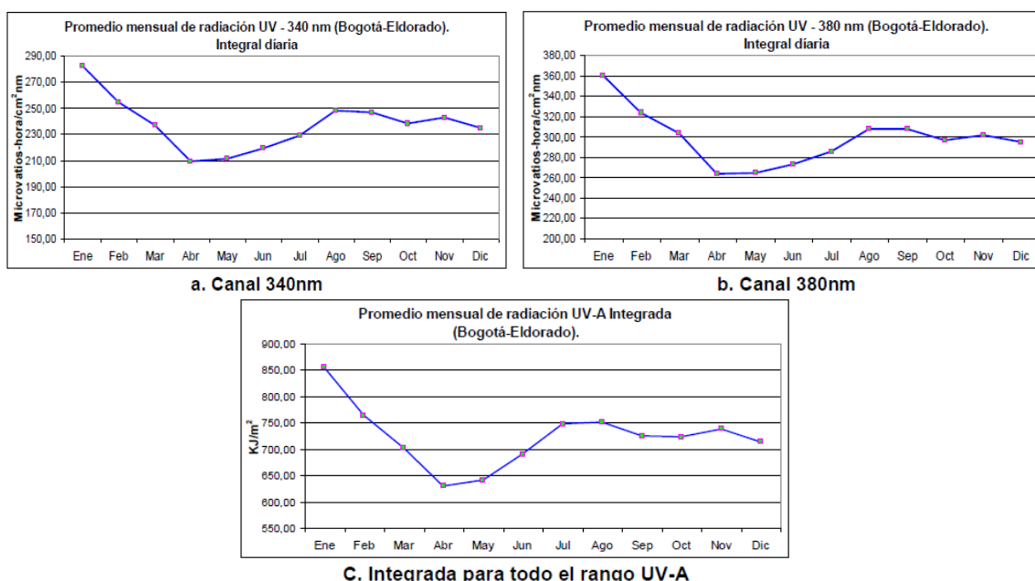
Illustration 5. Average monthly UV-A integrated day in the channel 340nm, 380nm and integrated for the UV-A range in Eldorado. (Source: IDEAM).
