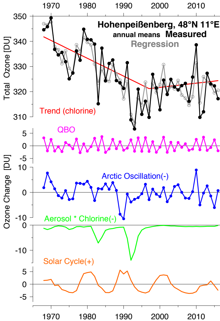
Fig. 7: Observed annual mean total ozone at Hohenpeissenberg, and multiple linear regression analysis of the magnitude of contributing factors. Top: Black: Observations at Hohenpeissenberg (47.8°N, 11°E). Gray: Multiple linear regression result. Red: Ozone variation attributed to Effective Equivalent Stratospheric Chlorine (EESC). Lower graphs: Ozone variation attributed to the QBO (magenta), to the Arctic Oscillation (AO, blue), to enhanced stratospheric aerosol (green), and to the 11-year solar cycle (orange). Plot by W. Steinbrecht, DWD.
