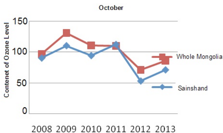
Figure 7. October average total ozone
