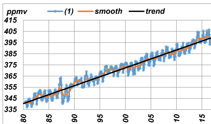
Figure 19. Variation of average monthly (1), inter annual (smooth) values of CO 2 and linear trend (trend).
