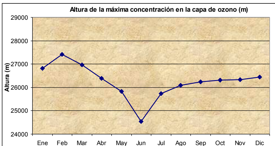
Illustration 3. Behavior of the height of the maximum concentration in the ozone layer, based on the ozone-soundings made in Bogotá. (Source: IDEAM).
