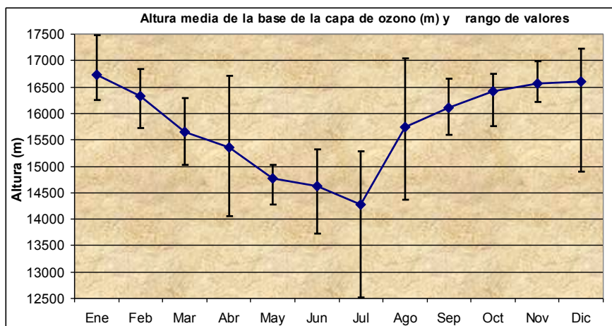
Illustration 2. Behavior of the monthly average height of ozone layer base. (Source: IDEAM).
