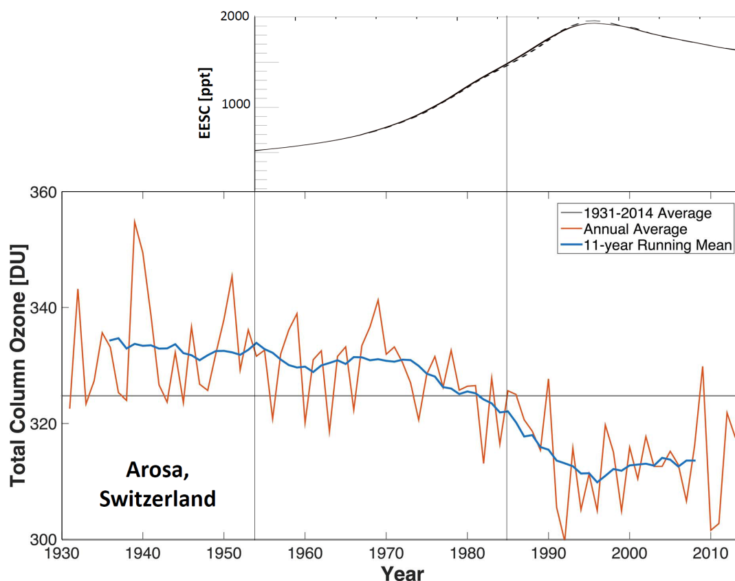
Figure 5: Total ozone time series from Arosa (annual mean values in Dobson Units [DU], lower panel) and effect of chemical ozone depletion as described by the Equivalent Effective Stratospheric Chlorine (EESC) for mid-latitudes (top panel), Fig. 4 of Staehelin et al., 2016).
