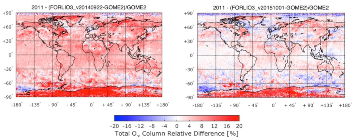
Figure 2. Global distribution of the relative differences (in %) between FORLI v20140922 (left panel) and FORLI v20151001 (right panel) against GOME-2A O3M-SAF TOCs averaged over 12 days of 2011 (on the 15th of each month) and over a 1° x 1° grid. The relative difference is calculated as: 100 \times (\text{FORLI-O}_3 - \text{GOME-2}) / \text{GOME-2} ( Boynard et al., 2016 ).
