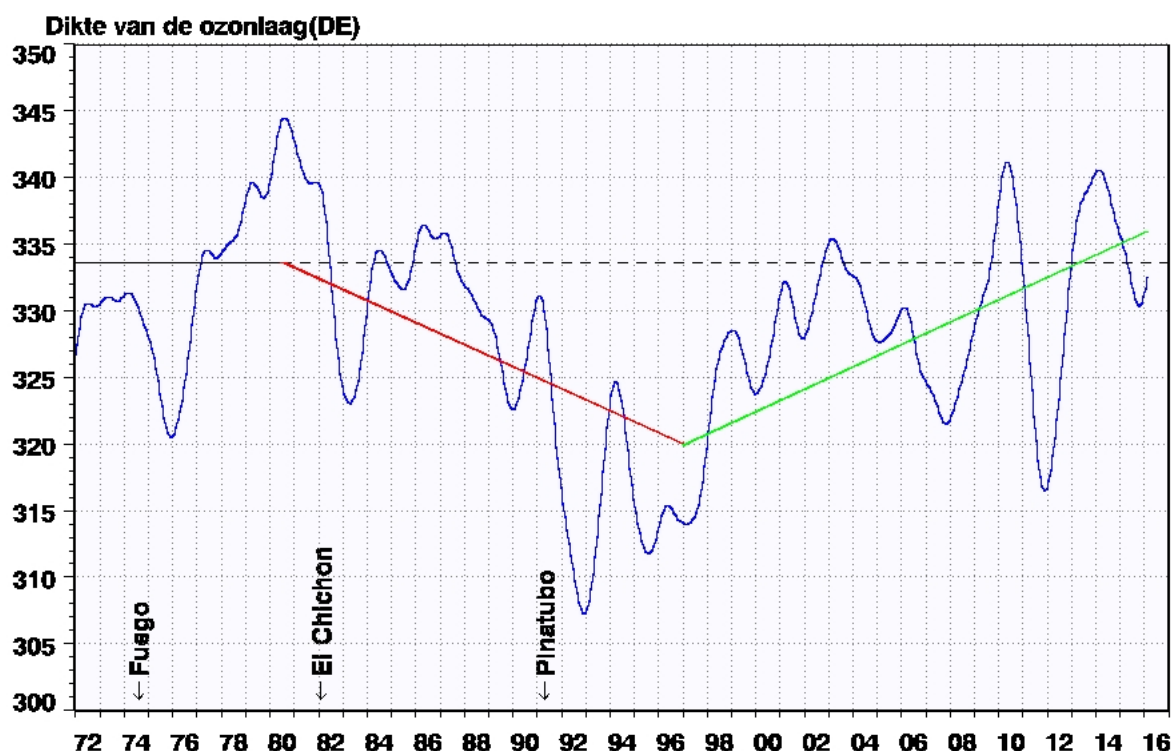
Figure 1. Running annual mean of total ozone (in Dobson Units) from Dobson and Brewer spectrophotometers at Uccle, together with a stepwise regression. The times of major volcanic eruptions, affecting the ozone layer are also indicated.
