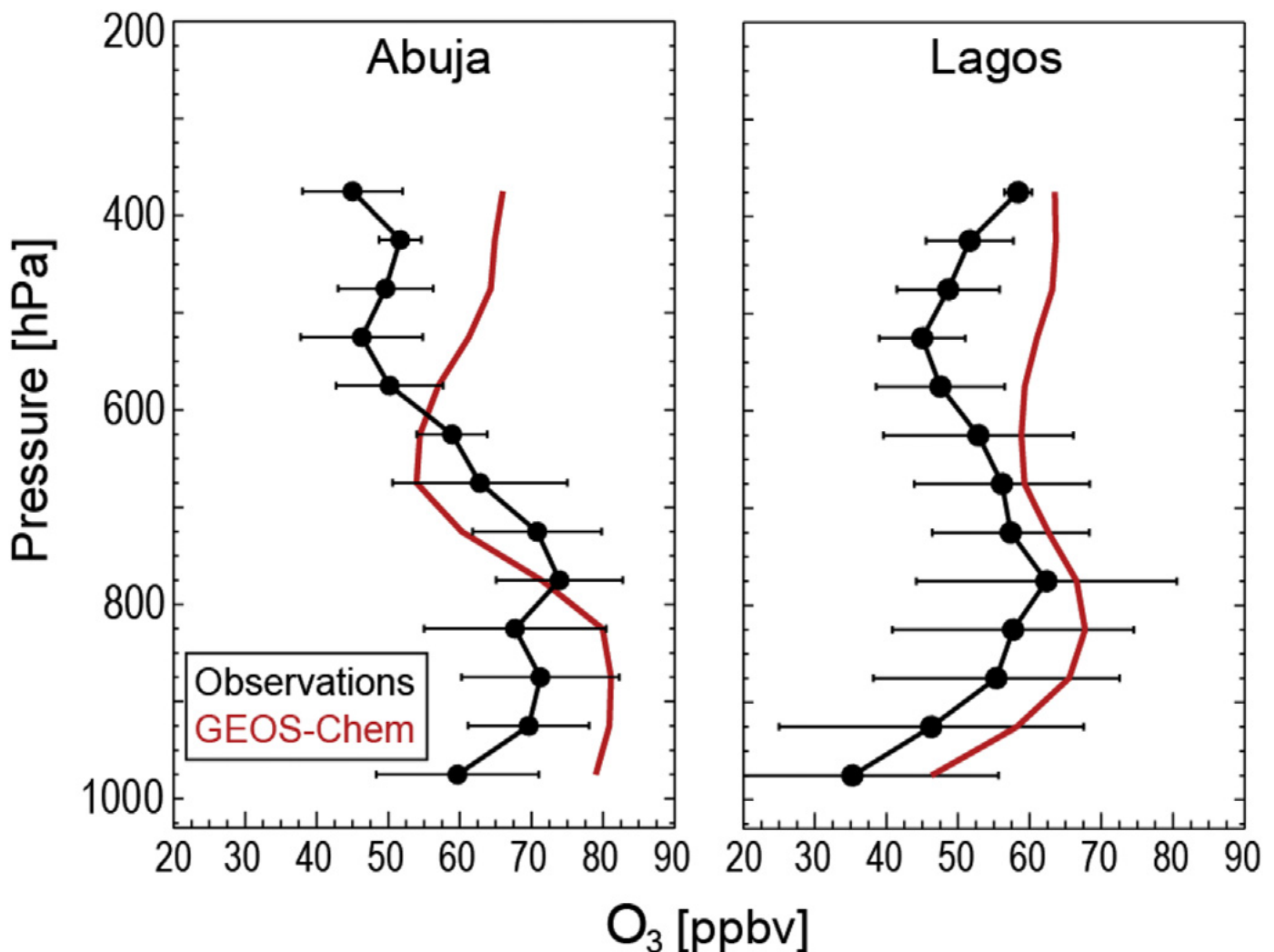
Fig. 1: Mean vertical profiles of O 3 concentrations over Abuja and Lagos in January to February
