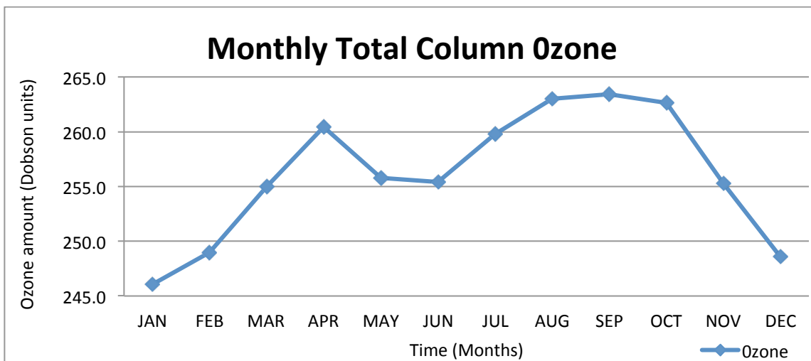
Fig: 2. Mean monthly total column of ozone
