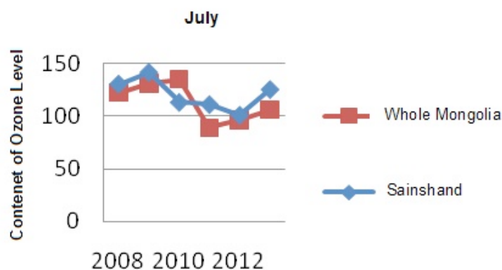
Figure 6. July average total ozone
