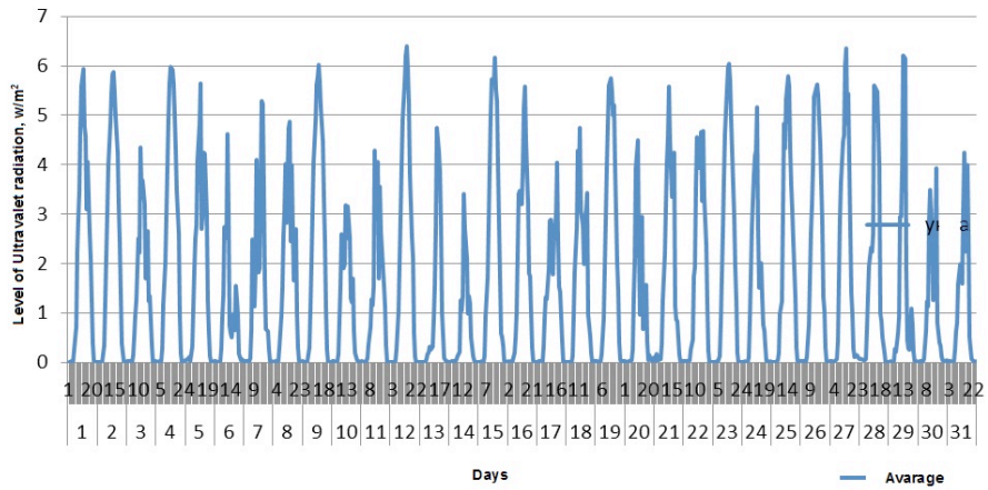
Figure 1. Level of UV radiation as of July 2013
