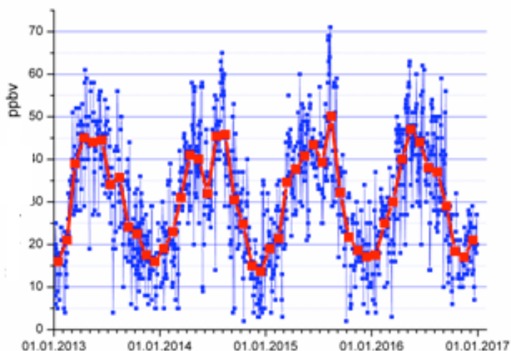
Figure 2.3 Surface ozone at NOMREC BSU Minsk Ozone Station for 2013-2016. Blue: noon concentrations. Red: monthly averages of noon values.
