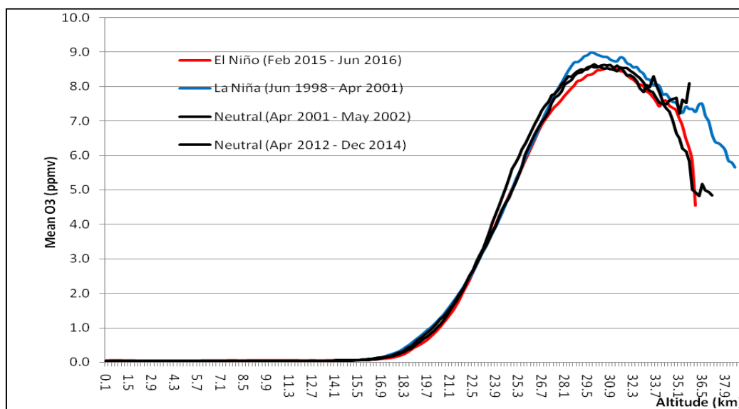
Figure 4. Vertical ozone profiles during strong El Niño (Feb. 2015-June 2016), moderate La Niña (June 1998-Apr. 2001) and two neutral periods (Apr. 2001-May 2002 & Apr. 2012-Dec. 2014).
