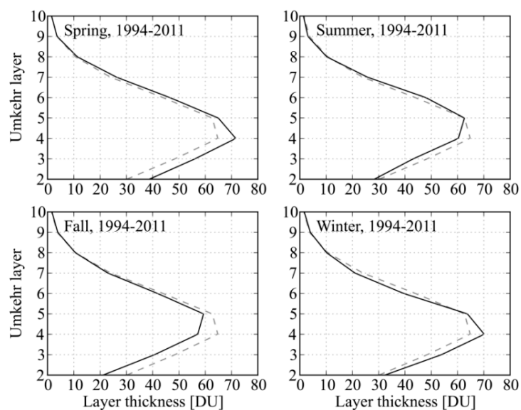
Fig. 1: Climatological Umkehr profiles, seasonal means (black line) and mean over the whole year (dashed line, grey) for spring, summer, fall and winter.
