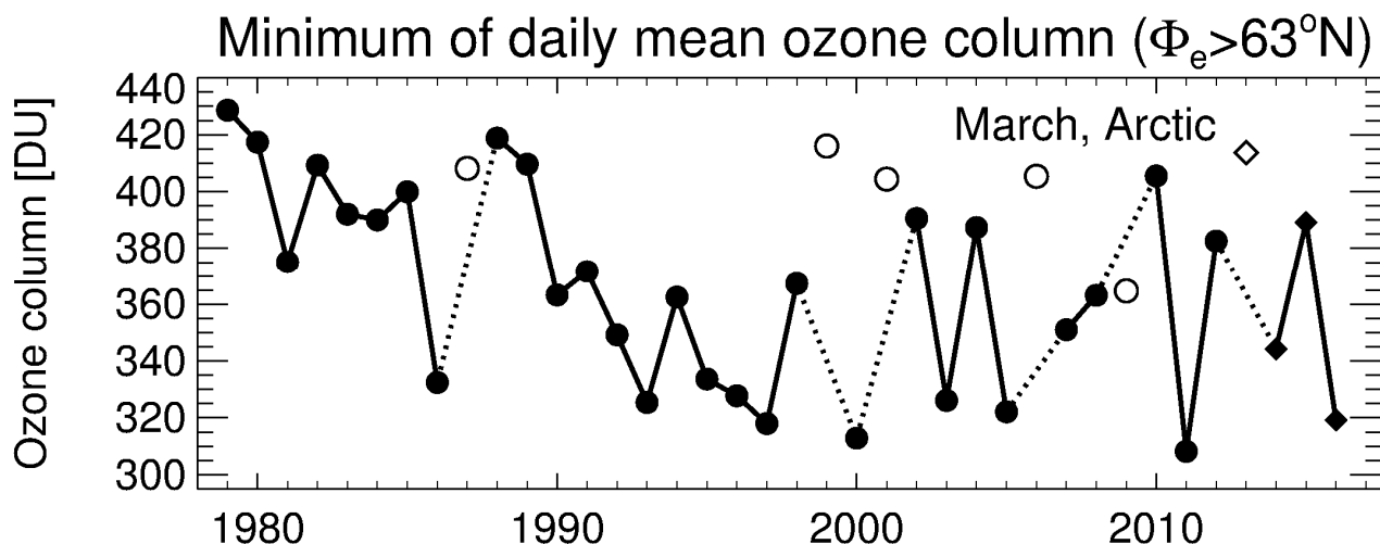
Fig. 14: Measure of Arctic ozone depletion given as the minimum of daily average column ozone poleward of 63° equivalent latitude in March. Open circles represent years in which the polar vortex broke up before March. Update from Müller et al. 2008, and WMO 2014.
