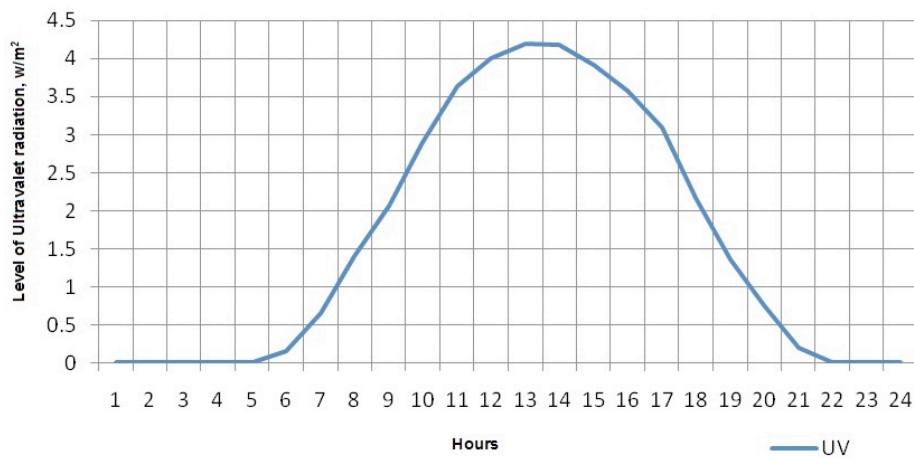
Figure 2. Daily trend of UV radiation
