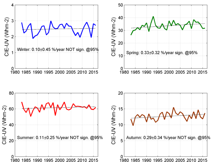
Figure 4. Seasonal CIE-weighted UV-radiation measured at Norrköping 1983-2016.
