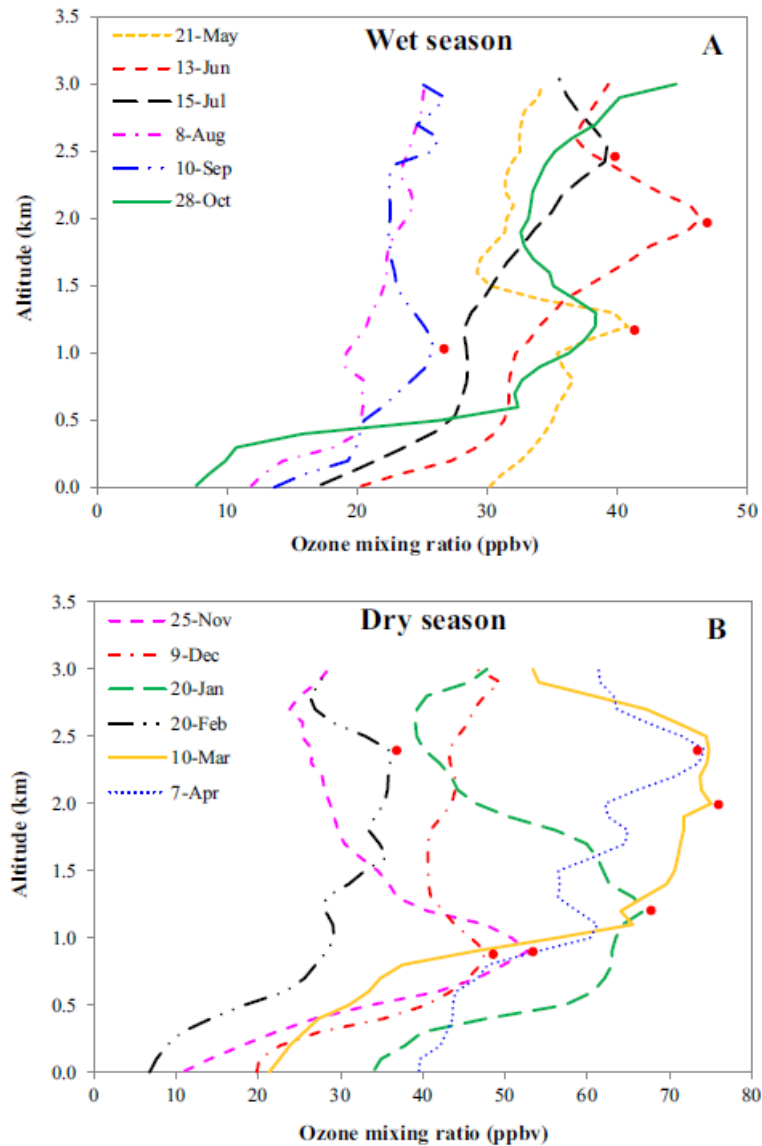
Figure 2.3. Ozone soundings showing mixing ratios in the bottom 3000 m of the atmosphere for A) the wet season from May-October, 2014 and B) the dry season from November 2014 to April 2015. Circles denote localised maxima.
