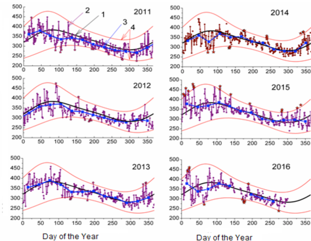
Figure 2.2. The TO average daily values over the territory of Belarus in 2011 - 2016. 1 – the annual variation of the climatic norm, 2 – observations data, 3 – monthly average values, 4 – 95% confidence interval. Asterisks denote the most significant ozone anomalies.
