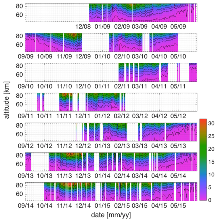
Figure 3. CO-profiles from KIMRA from Dec. 2008 to May 2015, Kiruna, Ryan et al. (2016b).
