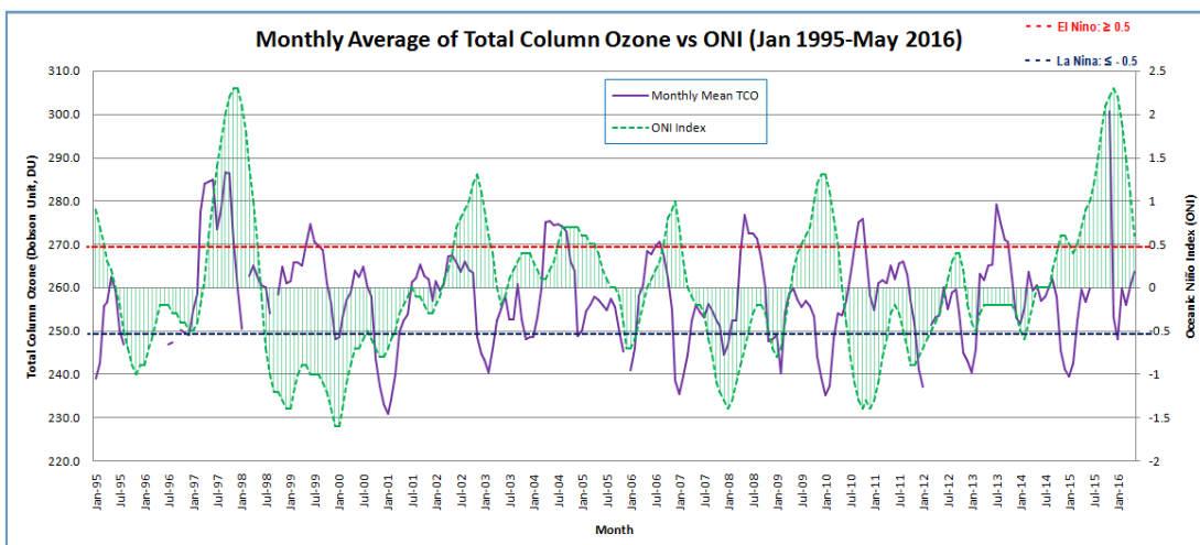
Figure 3. The monthly average of TCO and ONI in Petaling Jaya (1995-2016).
