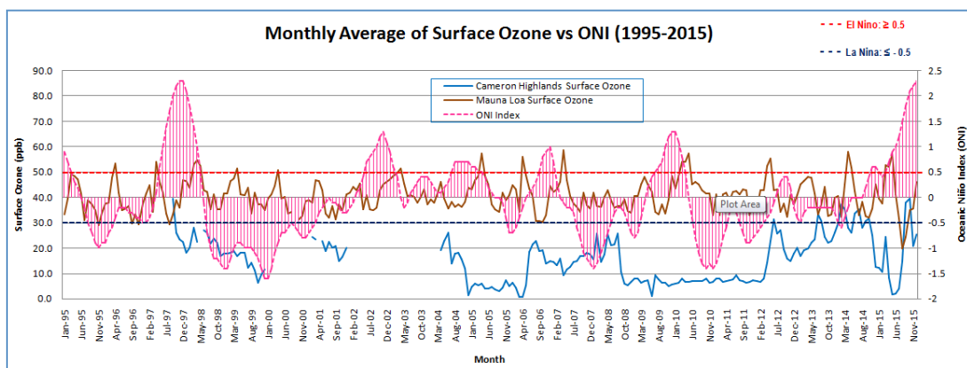
Figure 2. The monthly average of surface ozone and Ocean Niño Index (ONI) in Cameron Highlands and Mauna Loa (1995-2015).
