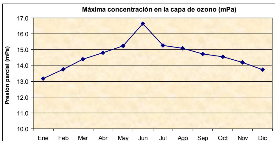
Illustration 4. Behavior of the maximum concentration in the ozone layer, based on the Ozonosondeos made in Bogotá. (Source: IDEAM).
