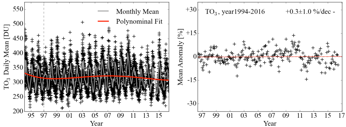
Fig. 4: Left: total ozone measured with the Brewer MkIV #93 spectro-photometer between 1994 and 2016 and monthly means; Right: year round trend estimates of monthly mean anomalies of total ozone
