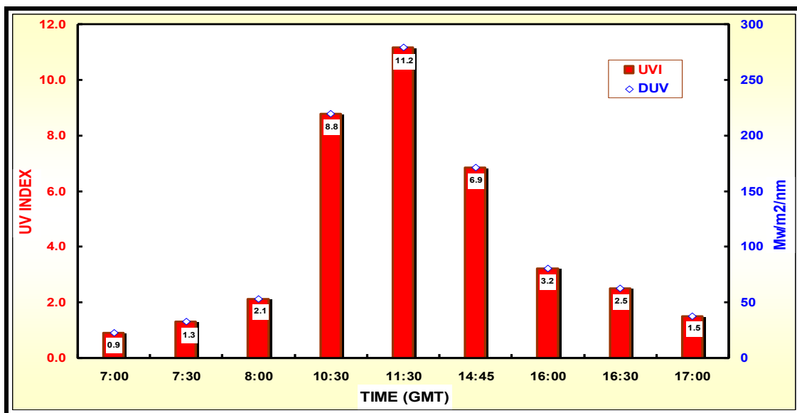
Fig.(6): Diurnal variation of Dangerous UV on a clear summer day over Matrouh
