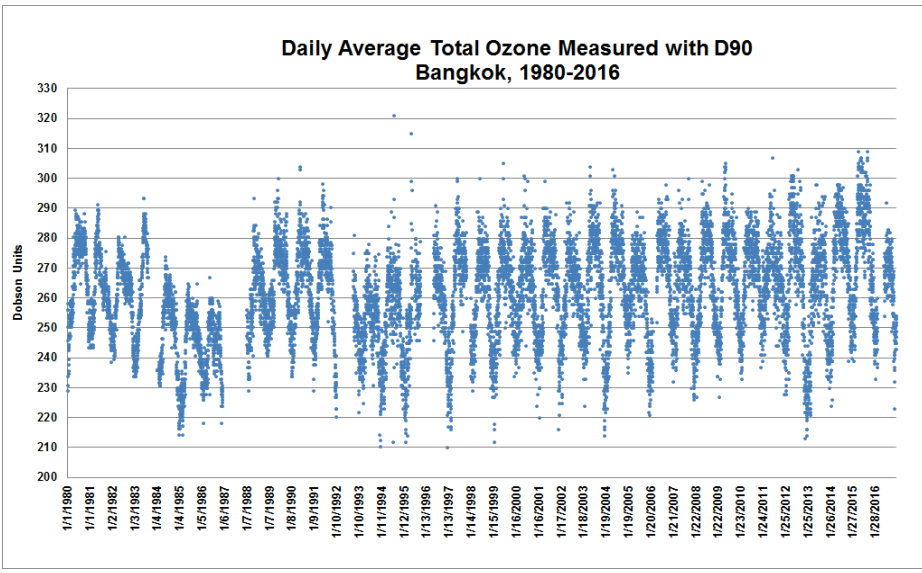
Figure 2.1. Daily average of total ozone measured with Dobson No.90 in Bangkok
