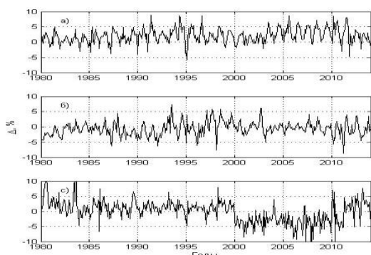
Figure 10. Relative deviation \Delta (%) between ground-based and satellite (V86) measurement of TO 1980-2013. a) – Hianghe Station (No208), b) – Kunming Station (No 209), c) – Issyk-Kul Station (No 347).
