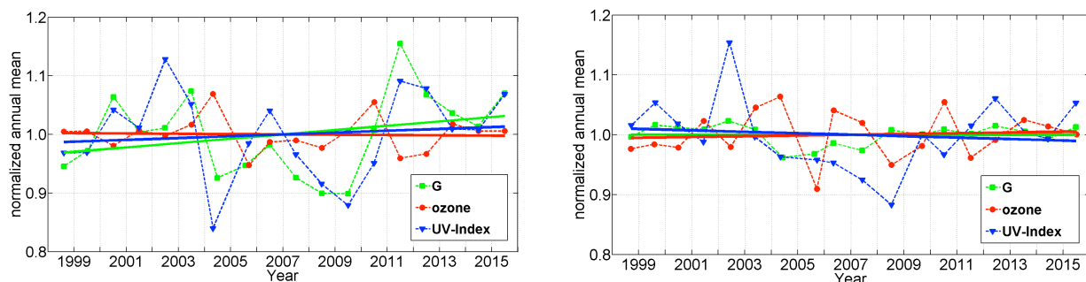
Fig. 2: Annual mean values (dots) of UV-Index, ozone and global radiation (G) for all weather conditions (left) and for days with clear sky conditions (right) at 19° solar elevation in Innsbruck, normalized to the respective mean value over 18 years. Straight lines show the linear fit.
