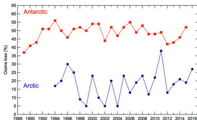
Figure 3. Ozone loss in Antarctica (red line) and Arctic (blue line) since 1989 and 1994, respectively.
