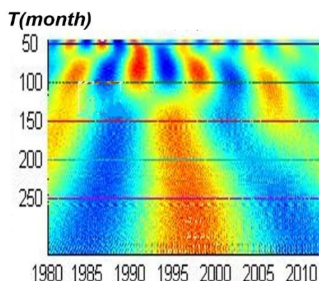
Figure 20. The results of wavelet analysis of time series of CO 2 1980-2015 [3]
