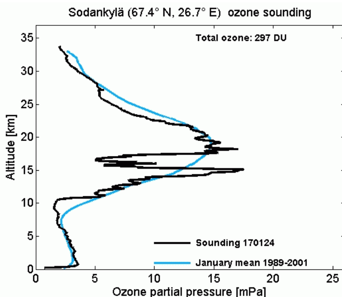
Figure 1. Ozone sounding at Sodankylä in January 2017. The ozone soundings have been made on regular basis in an effort to study Arctic stratospheric and tropospheric ozone changes. Results of the ozone soundings have been made publicly available through the FMI web site.
