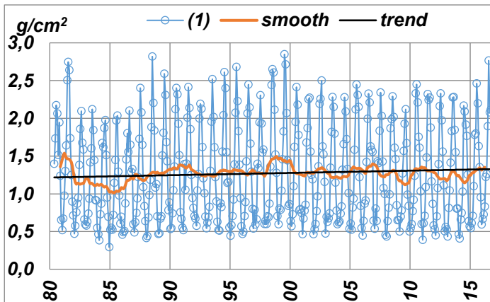
Figure 17. Variations of \text{H}_2\text{O} : monthly average (1), inter annual (smooth), linear trend (trend)
