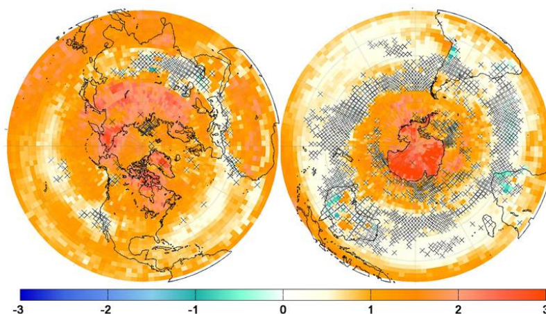
Figure 3. Global distribution of the trend values (given in DU/year) estimated by applying a multivariate regression model on daily IASI time series over the period 2008-2015. The crosses indicate that the trend in the grid cell is non-significant in the 95% confidence limits ( 2\sigma level) when accounting for the autocorrelation in the noise residual.
