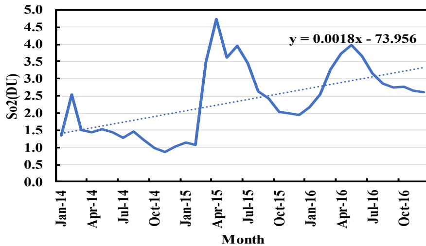
Fig. (5): Monthly variation of total column of sulfur dioxide (SO 2 )
