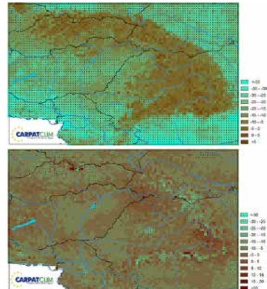
Figure 11: Change in the start date of the growing season 5°C (up) and 10°C (down) in days in the period of 1961–2010. Significant changes at 90% level are marked with dots (source: CARPATCLIM).
