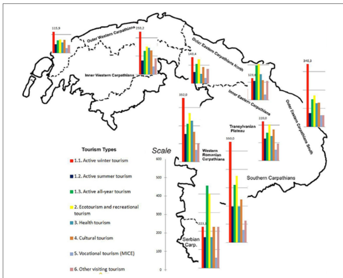
Figure 19: Vulnerability map of the Carpathian regions (source: CarpathCC).
