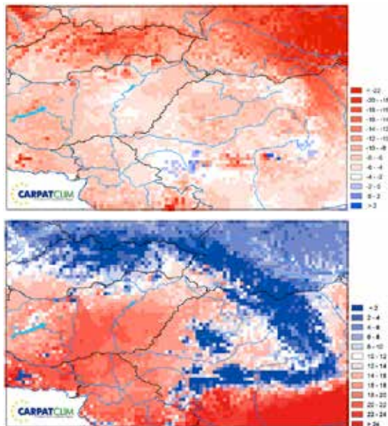
Figure 10: Change in the number of winter days per year (daily maximum < 0°C, up) and hot days per year (daily maximum ≥ 30°C, down) in the Carpathian region in the period of 1961–2010 (source: CARPATCLIM).
