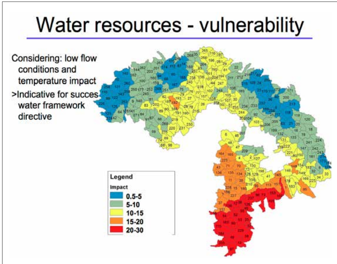
Figure 13: Vulnerability of water resources in the Carpathians (source: CarpathCC).
