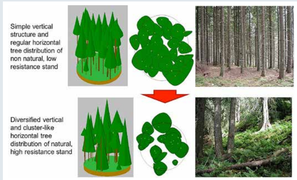
An extended cutting regime leads to adaptation of forest structure (source: CarpathCC Project presentation)
